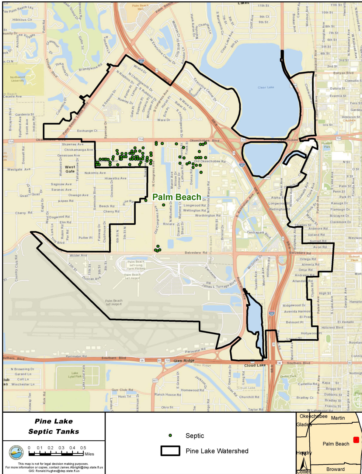
Figure 4.2. OSTDS in the Pine Lake Watershed
