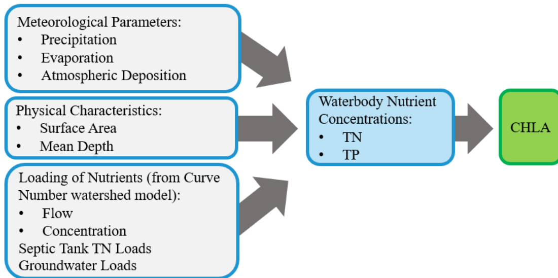
Figure 5.2. BATHTUB Model conceptual diagram
