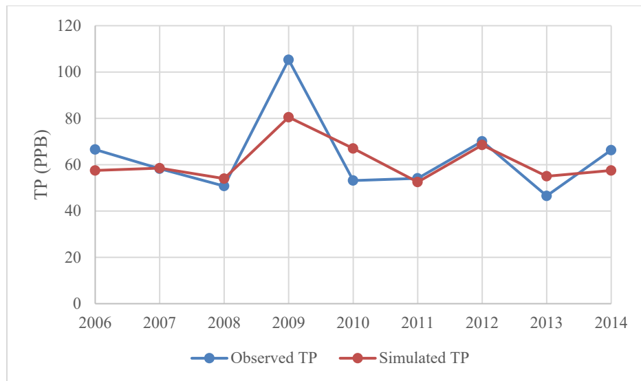
Figure 5.4. Predicted and observed TP concentrations in Pine Lake
