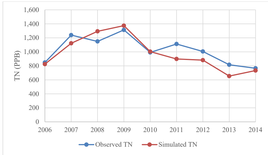
Figure 5.3. Predicted and observed TN concentrations in Pine Lake
