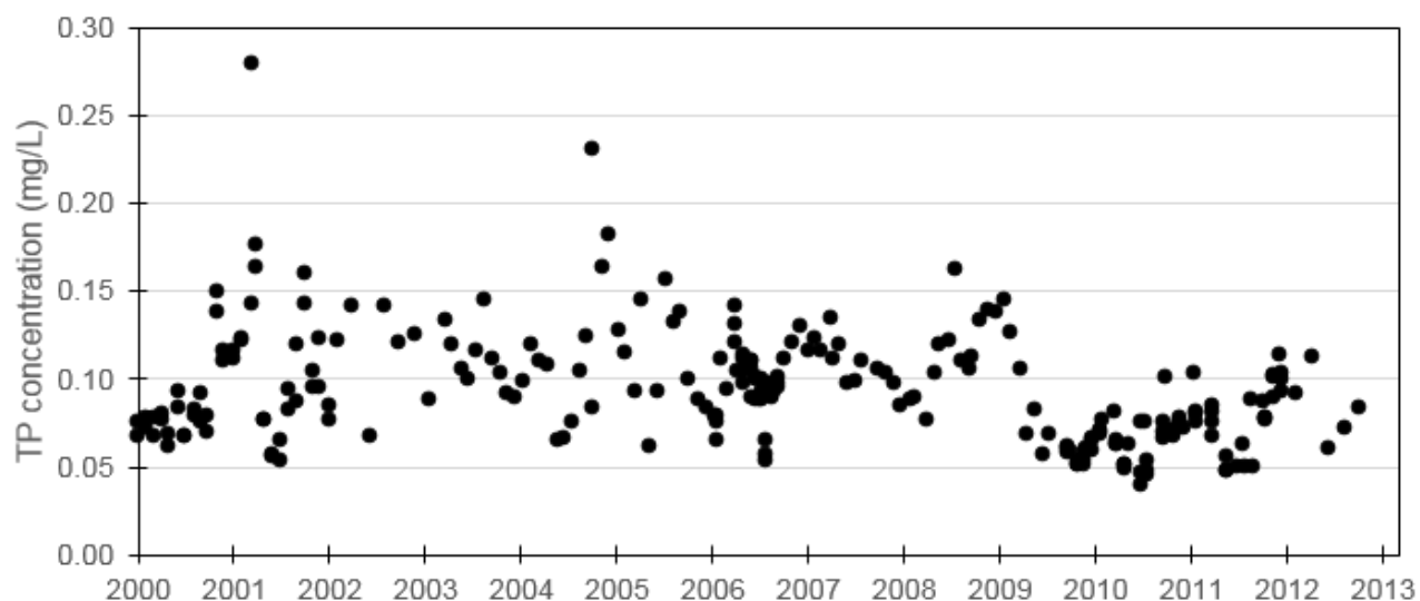
Figure 5.3a. TP Concentrations Measured for Lake Denham, 2000–12
