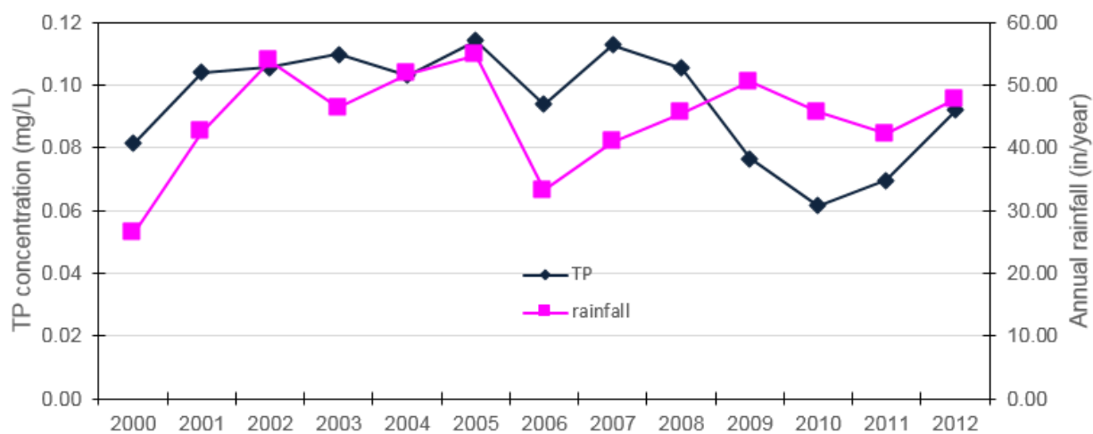
Figure 5.3b. Relationship between Annual Rainfall and TP AGM for Lake Denham, 2000–12
