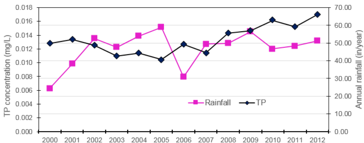
FIGURE 5.3B. RELATIONSHIP BETWEEN ANNUAL RAINFALL AND TP AGM
