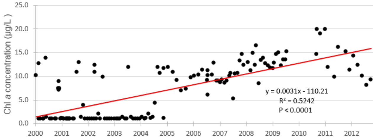
FIGURE 5.4A. CHL A CONCENTRATIONS MEASURED FOR LAKE WEIR, 2000–12
