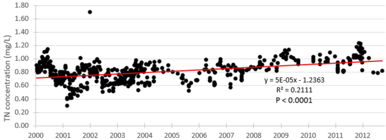
FIGURE 5.2A. TN CONCENTRATIONS MEASURED FOR LAKE WEIR, 2000–12
