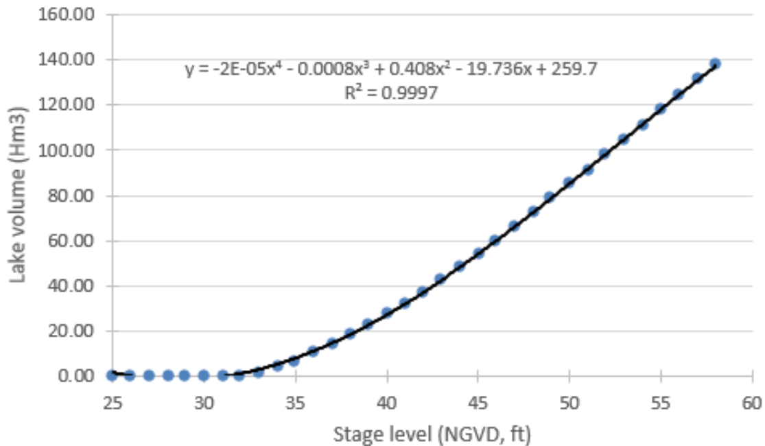
FIGURE 5.7. CHARACTERISTIC CURVE BETWEEN LAKE STAGE AND LAKE CUMULATIVE VOLUME FOR LAKE WEIR
