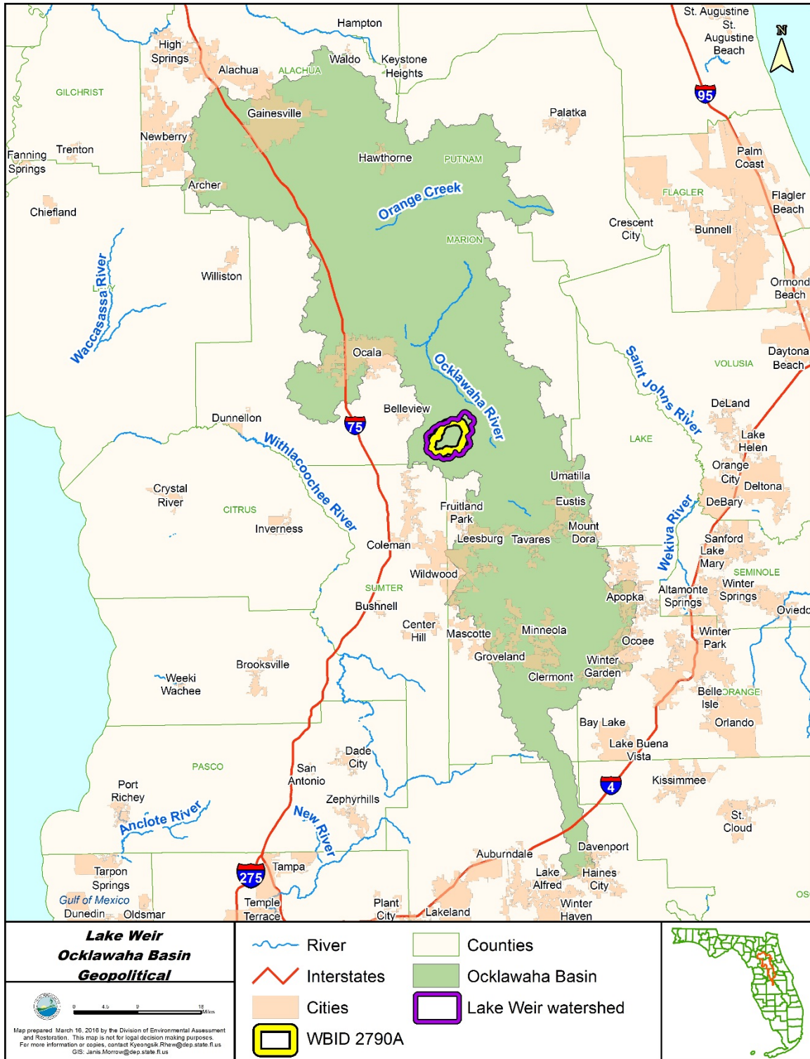
FIGURE 1.1. LOCATION OF LAKE WEIR (WBID 2790A) IN THE OCKLAWAHA BASIN AND MAJOR GEOPOLITICAL AND HYDROLOGIC FEATURES IN THE AREA
