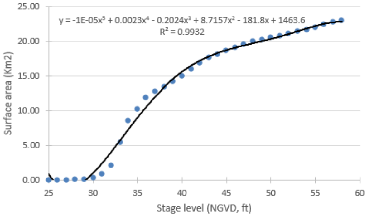
FIGURE 5.6. CHARACTERISTIC CURVE BETWEEN LAKE STAGE AND LAKE SURFACE AREA FOR LAKE WEIR
