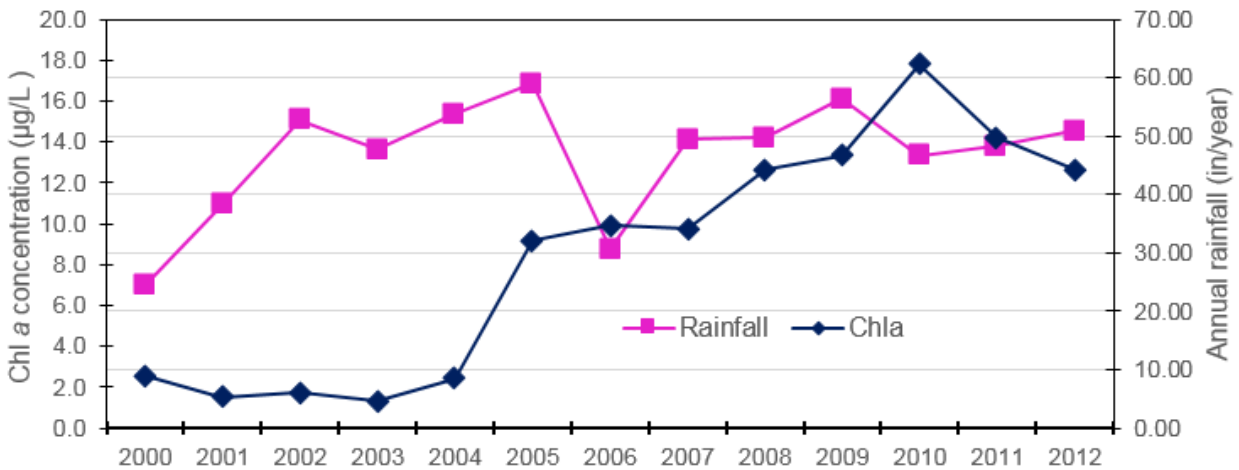
FIGURE 5.4B. RELATIONSHIP BETWEEN ANNUAL RAINFALL AND CHL A AGM
