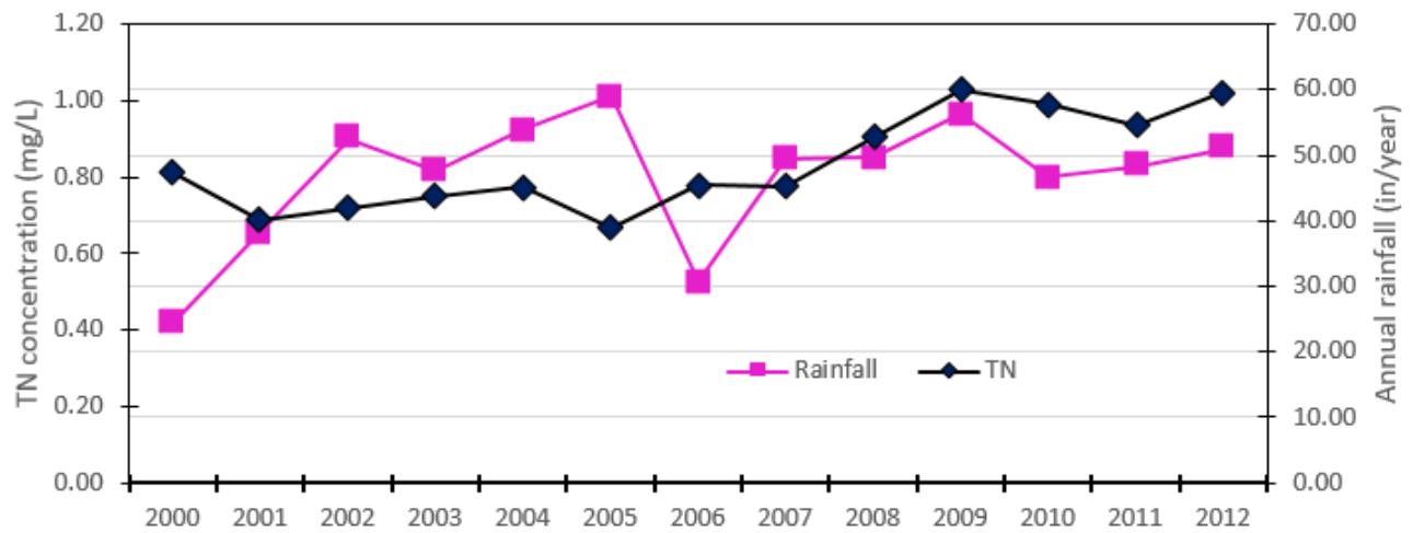
FIGURE 5.2B. RELATIONSHIP BETWEEN ANNUAL RAINFALL AND TN AGM, 2000–12
