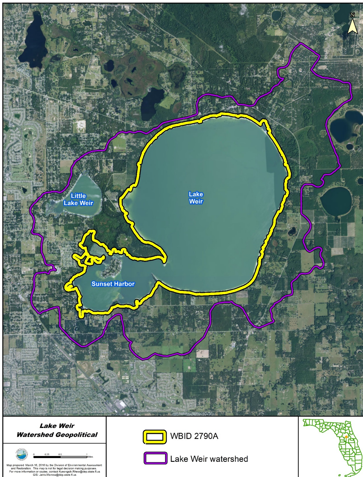
FIGURE 1.2. DETAILED VIEW OF LAKE WEIR IN MARION COUNTY AND HYDROLOGIC FEATURES IN THE AREA
