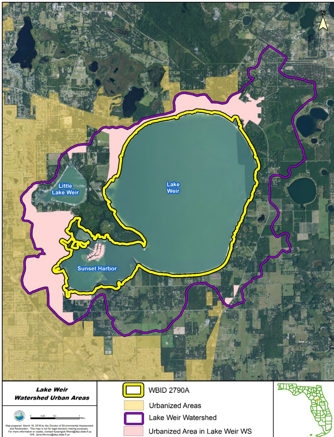
FIGURE 4.1. URBANIZED AREAS IN THE LAKE WEIR WATERSHED (UNITED STATES CENSUS BUREAU 2010)
