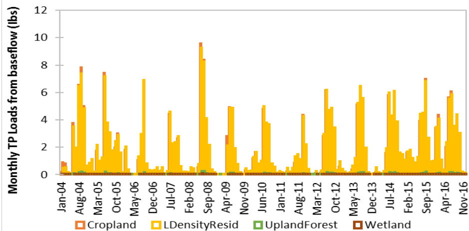
Figure 4.10. Simulated monthly TP loads to Lake Persimmon via surface runoff (top), interflow (middle), and baseflow (bottom) during the simulation period, 2004–16
