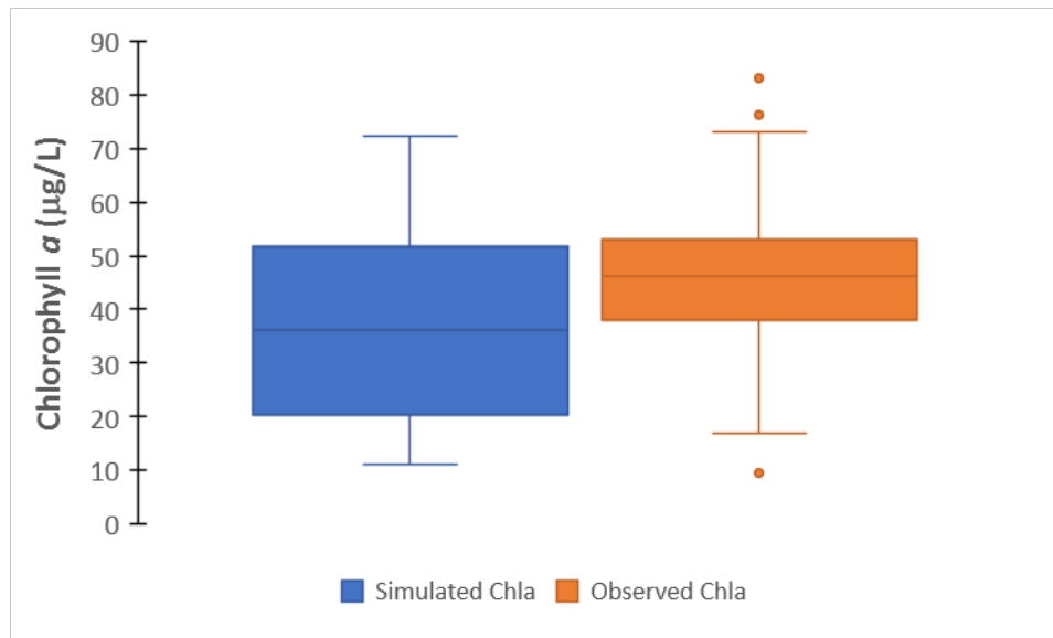
Figure 5.10. Box-whisker plot of simulated versus observed chlorophyll a (µg/L) in Lake Persimmon
