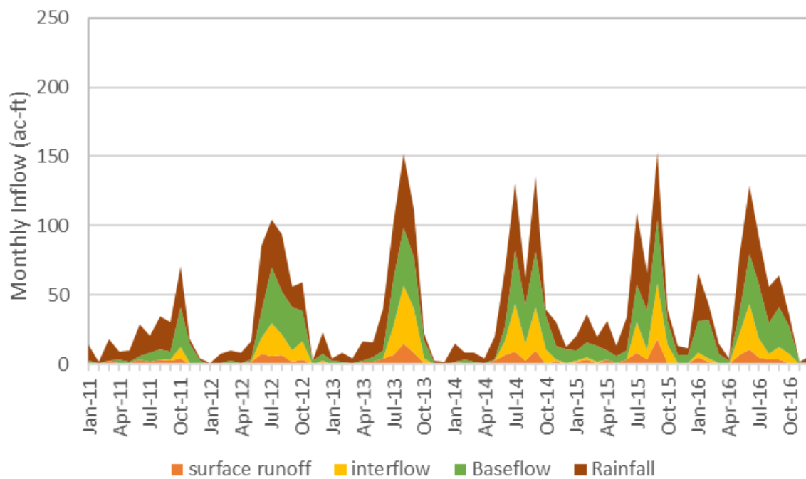
Figure 4.7. Simulated monthly inflows to Lake Persimmon during the simulation period, 2004–10 (top) and 2011–16 (bottom)
