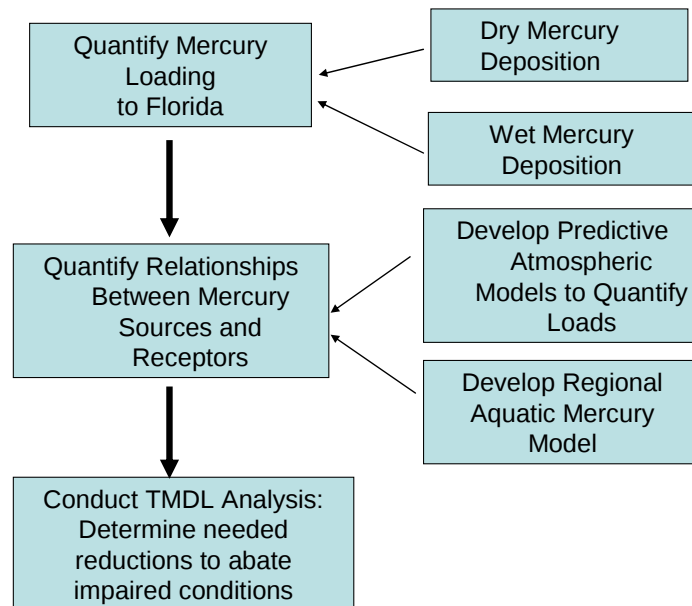
Figure 1. Overview of the technical components of a statewide Mercury TMDL.
