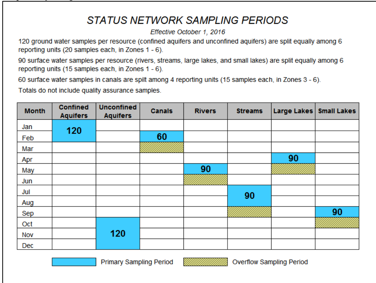
Figure 2. Status Network sampling periods. Samples are split evenly among the state's six zones, except for canals, which are split evenly among Zones 3-6.
