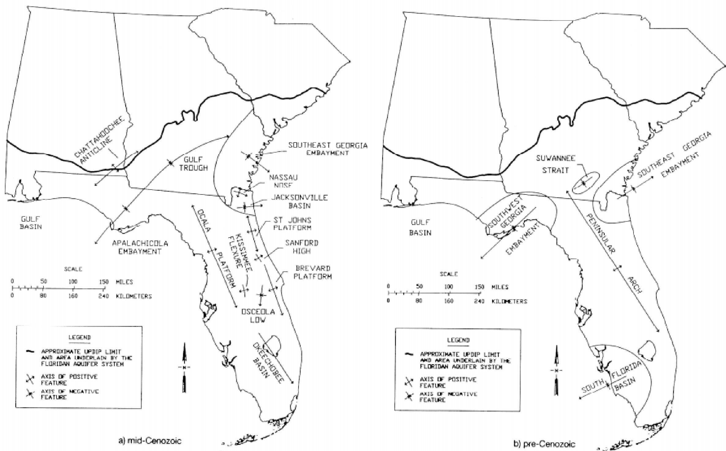
Figure 4. Structural features of Florida: a) mid-Cenozoic b) pre-Cenozoic
