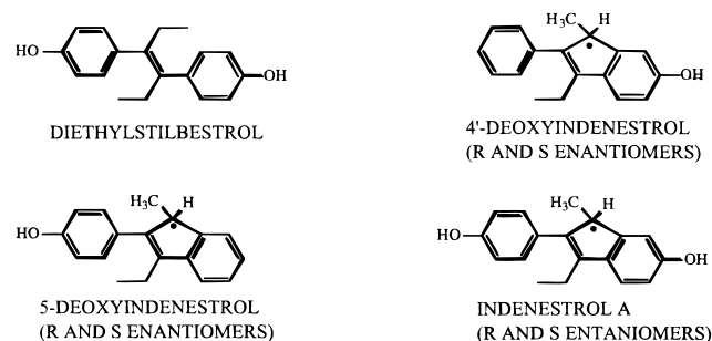
Figure 7. Structures of compounds in DES subset.
