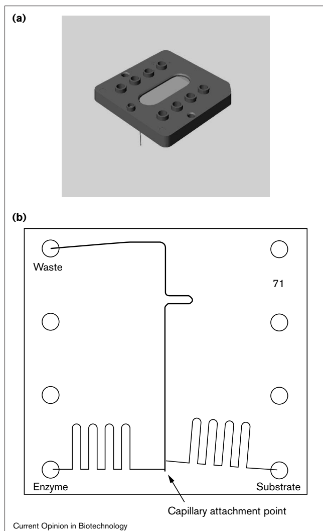
(a) A microfluidic device for running continuous-flow enzyme inhibition assays. Test compounds are injected via a fused-silica capillary attached to the microchip. (b) Schematic layout of a continuous-flow enzyme inhibition assay chip.
