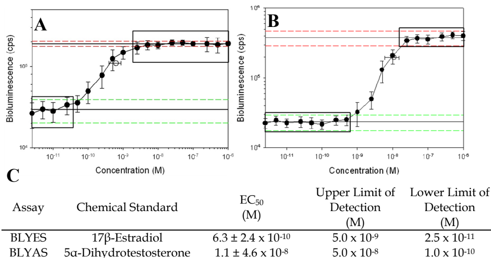
Fig. 3. A. S. cerevisiae BLYES standard curve (n = 13) using 17β-estradiol. B. S. cerevisiae BLYAS standard curve (n = 13) using dihydrotestosterone as a standard. Open circle: calculated EC_{50} values with error bars. A 50% effective concentration ( EC_{50} ) value was determined from the midpoint of the linear portion of the sigmoidal dose response curve. The mean and standard deviation values were calculated from replicate EC_{50} values for each standard to determine the variability between assays. C. Summary of EC_{50} values for BLYES and BLYAS strain with upper and lower limits of detection.
