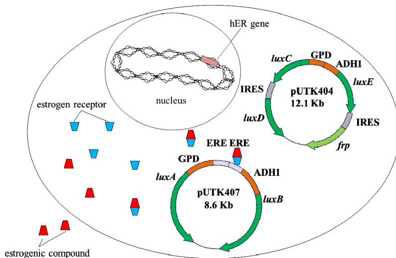
Fig. 2. Schematic representation of S. cerevisiae BLYES. Estrogenic compounds cross the cell membrane and bind to the human estrogen receptor (hER). This complex interacts with estrogen response elements (RE) initiating transcription of luxA and luxB . S. cerevisiae BLYES contains the human estrogen receptor in its genome, while S. cerevisiae BLYAS has the human androgen receptor in the genome.
