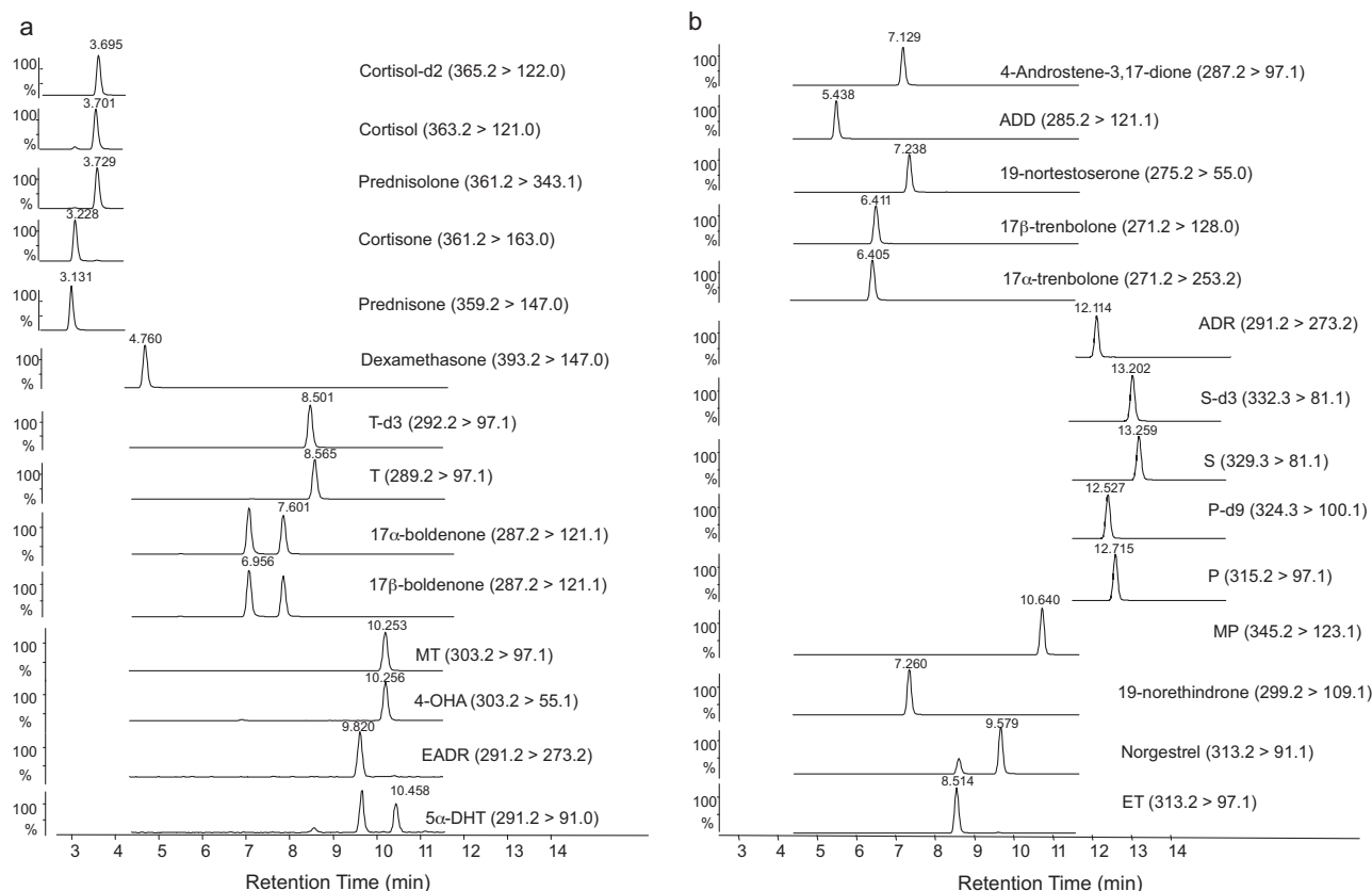
Fig. 3. (A) Extracted ion chromatograms (EIC) of the quantitative ions for glucocorticoids, androgens and progestagens in standard solution at the concentration each of 100 ng/L. Conditions: RR/MS/MS with positive ionization in MRM mode. T-d3, testosterone-d3; T, testosterone; MT, methyltestosterone; 4-OHA, 4-hydroxy-androst-4-ene-17-dione; EADR, epi-androsterone; 5α-DHT, 5α-dihydrotestosterone; ADD, androsta-1,4-diene-3,17-dione; S-d3, stanozolol-d3; S, stanozolol; P-d9, progesterone-d9; P, progesterone; MP, medroxyprogesterone; ET, ethynyl testosterone. (B) Extracted ion chromatograms (EIC) of the quantitative ions for glucocorticoids, androgens and progestagens in standard solution at the concentration each of 100 ng/L. Conditions: RR/MS/MS with positive ionization in MRM mode. T-d3, testosterone-d3; T, testosterone; MT, methyltestosterone; 4-OHA, 4-hydroxy-androst-4-ene-17-dione; ADR, androsterone; 5α-DHT, 5α-dihydrotestosterone; ADD, androsta-1,4-diene-3,17-dione; S-d3, stanozolol-d3; S, stanozolol; P-d9, progesterone-d9; P, progesterone; MP, medroxyprogesterone; ET, ethynyl testosterone.
