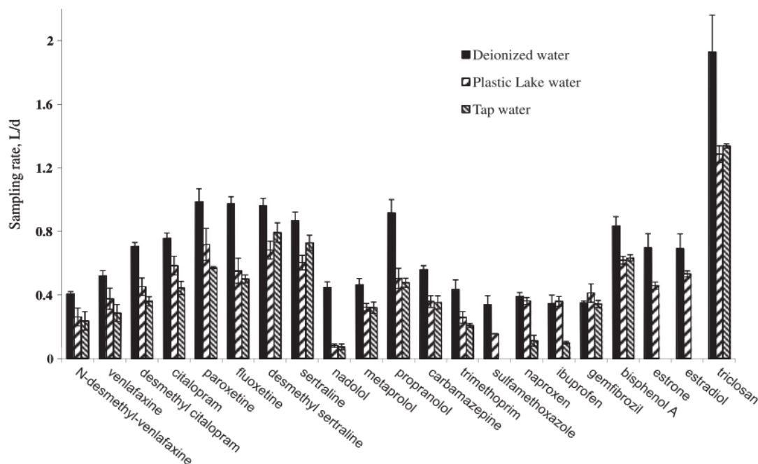
Fig. 2. The comparison of sampling rates of model compounds determined with Peterborough dechlorinated tap water and Plastic Lake water from the present study and with the deionized water cited from Li et al. (2010b). The pH of Plastic Lake water, dechlorinated tap water and deionized water were 6.13, 8.46 and 5.43, respectively. The concentration of dissolved organic carbon in Plastic Lake water, dechlorinated tap water and deionized water were 3.33, 4.55, <1 mg L -1 , respectively. The pH of the dechlorinated tap water was adjusted to 7 for uptake experiments. The pH values of deionized water and Plastic Lake water were not adjusted for these experiments. The temperature of the chamber where the uptake experiments were conducted was set at 25 °C for all these three types of water.
