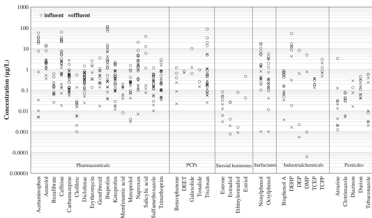
Fig. 1. Average concentrations (on logarithmic Y axis) reported for the selected micropollutants in WWPT influents and effluents (data from Table 2).
