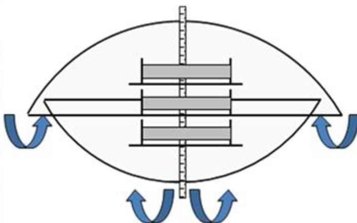
Figure 9. Double-bowl design for deploying semipermeable membrane devices (SPMDs) in air. Schematic on right shows three SPMDs contained inside the device (arrows show air movement direction around the lip of the bottom bowl and holes in the bottom of the device). Photograph and schematic by David Alvarez, U.S. Geological Survey.
