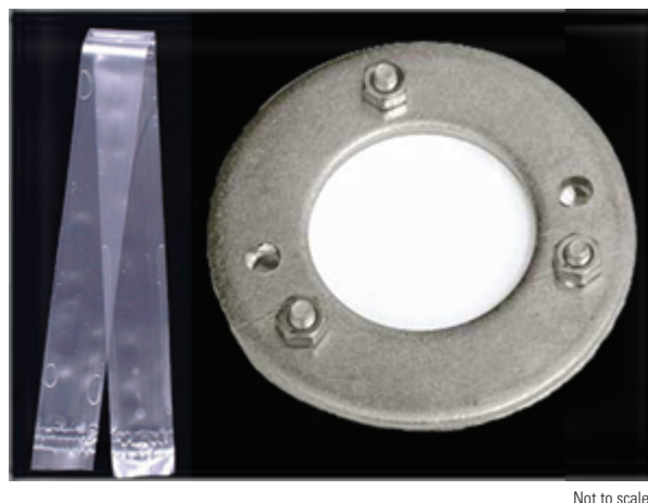
Figure 1. Semipermeable membrane device (SPMD, left) and the polar organic chemical integrative sampler (POCIS, right). Photographs by Randal Clark, U.S. Geological Survey (left) and Environmental Sampling Technologies (right).
