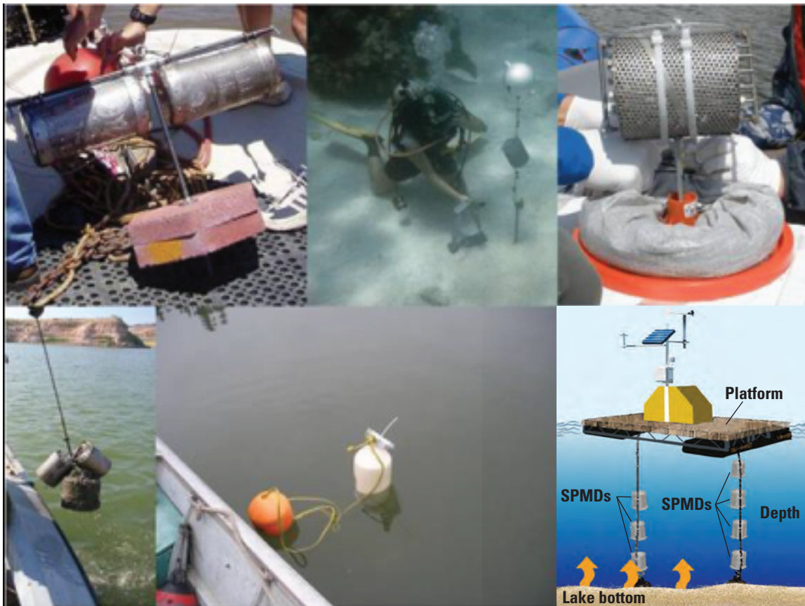
Figure 5. Deployment options in deep water suspending the canister off the bottom or for determining the vertical gradient of contaminant concentrations. Photographs by Kelly Smalling, U.S. Geological Survey (top left), David Alvarez, U.S. Geological Survey (top center, top right), Michael Rosen, U.S. Geological Survey (bottom left), and Jennifer Morace, U.S. Geological Survey (bottom center).
