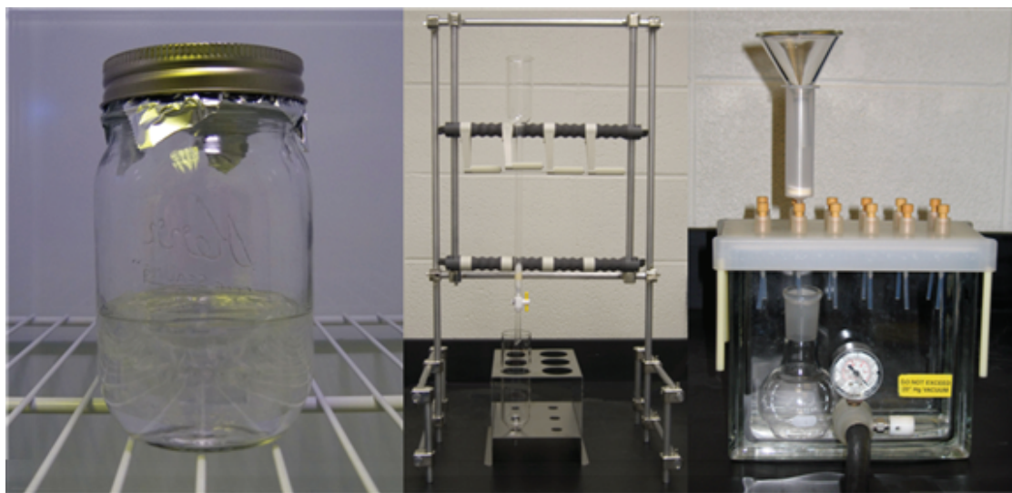
Figure 10. A typical semipermeable membrane device (SPMD) dialysis (left), polar organic chemical integrative sampler (POCIS) extraction using glass chromatography columns (center), and POCIS extraction using solid phase extraction cartridges (right). Photographs by David Alvarez, U.S. Geological Survey.
