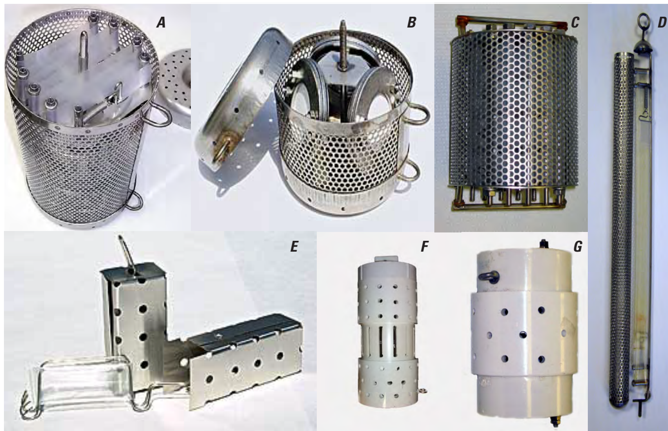
Figure 2. Custom and commercially available deployment canisters for semipermeable membrane devices (SPMDs) and polar organic chemical integrative samplers (POCIS). A , Commercially available large stainless steel canister for SPMDs or POCIS. B , Commercially available small stainless steel canister for SPMDs or POCIS. C , Custom “Prest-style” canister for SPMDs or POCIS. D , Commercially available stainless steel well sampling device. E , Commercially available stainless steel mini-SPMD canister. F , Custom large polyvinyl chloride (PVC) canister for POCIS. G , Custom PVC canister for POCIS. Photographs by Environmental Sampling Technologies ( A , B , E ) and David Alvarez, U.S. Geological Survey ( C , D , F , G ).
