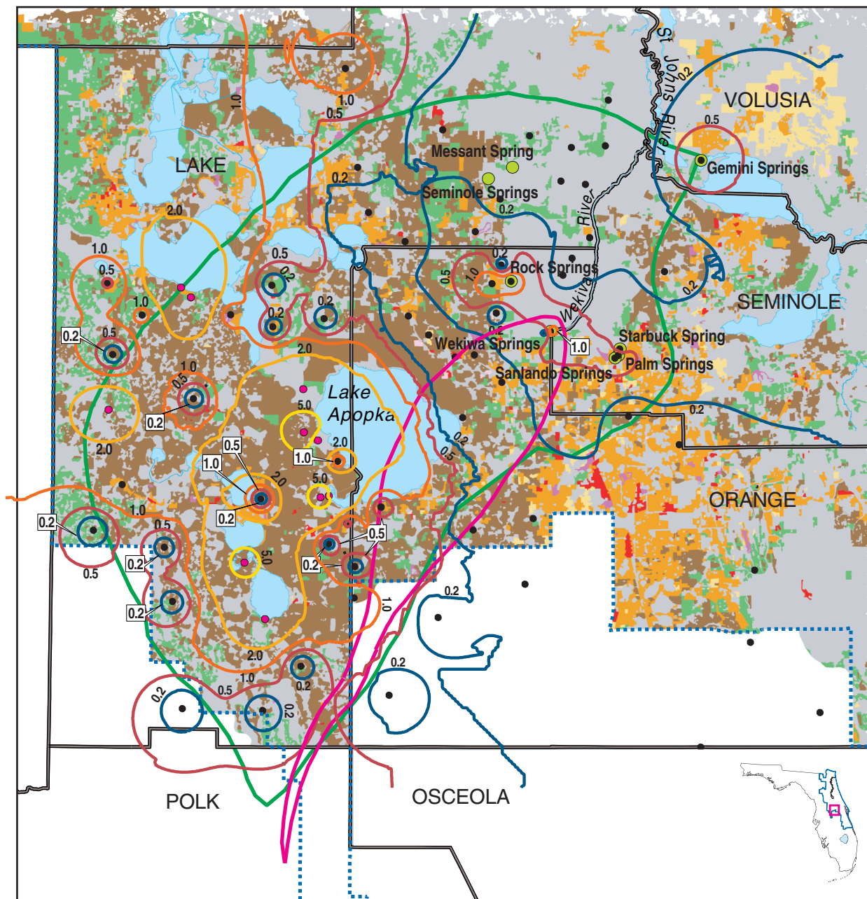
Figure 17. Relationship between total and dissolved nitrate nitrogen and 1973 land use in the study area
