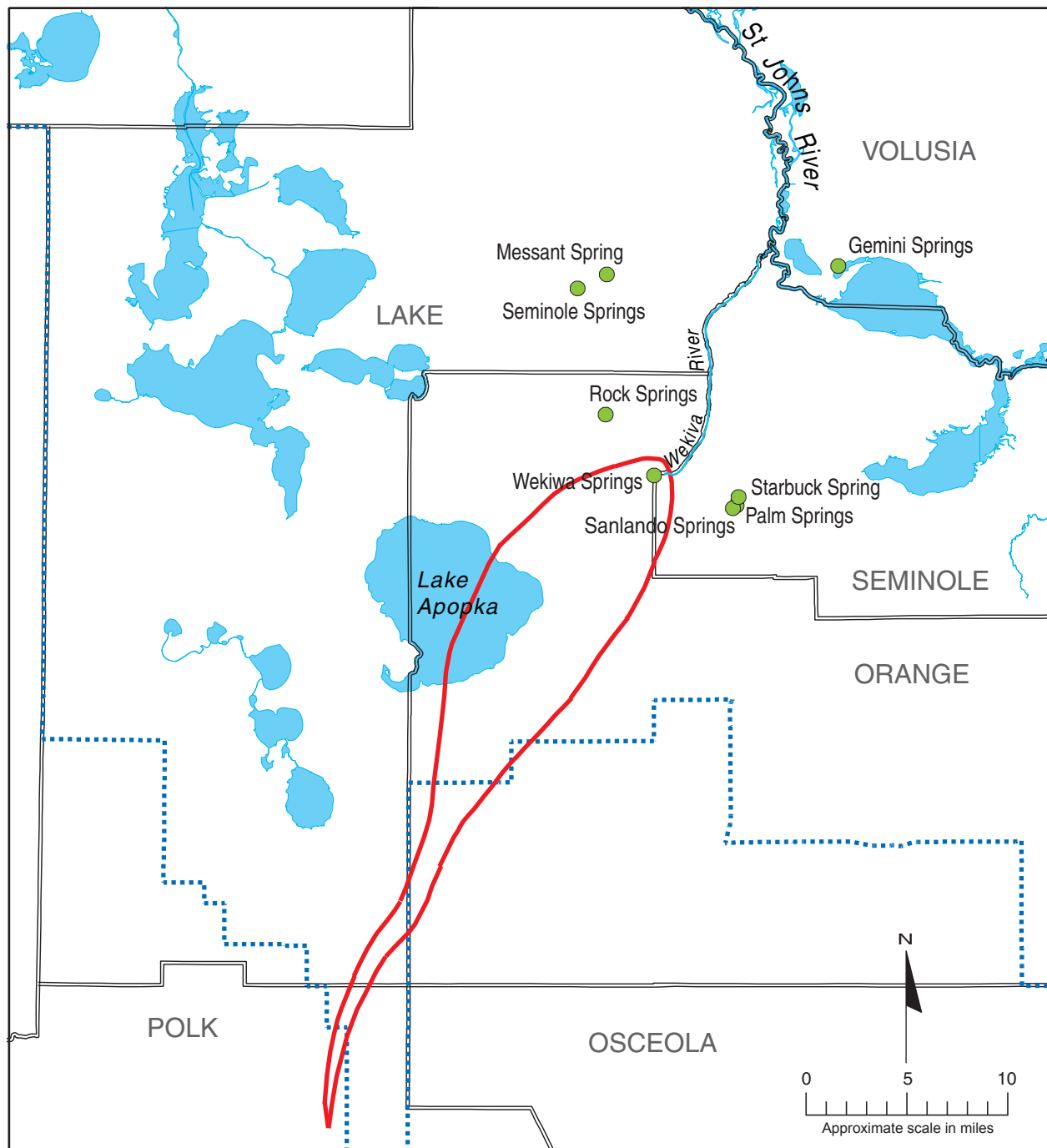
Figure 3. Wekiwa Springs groundwater basin (B. McGurk, SJRWMD, pers. com. 2000)
