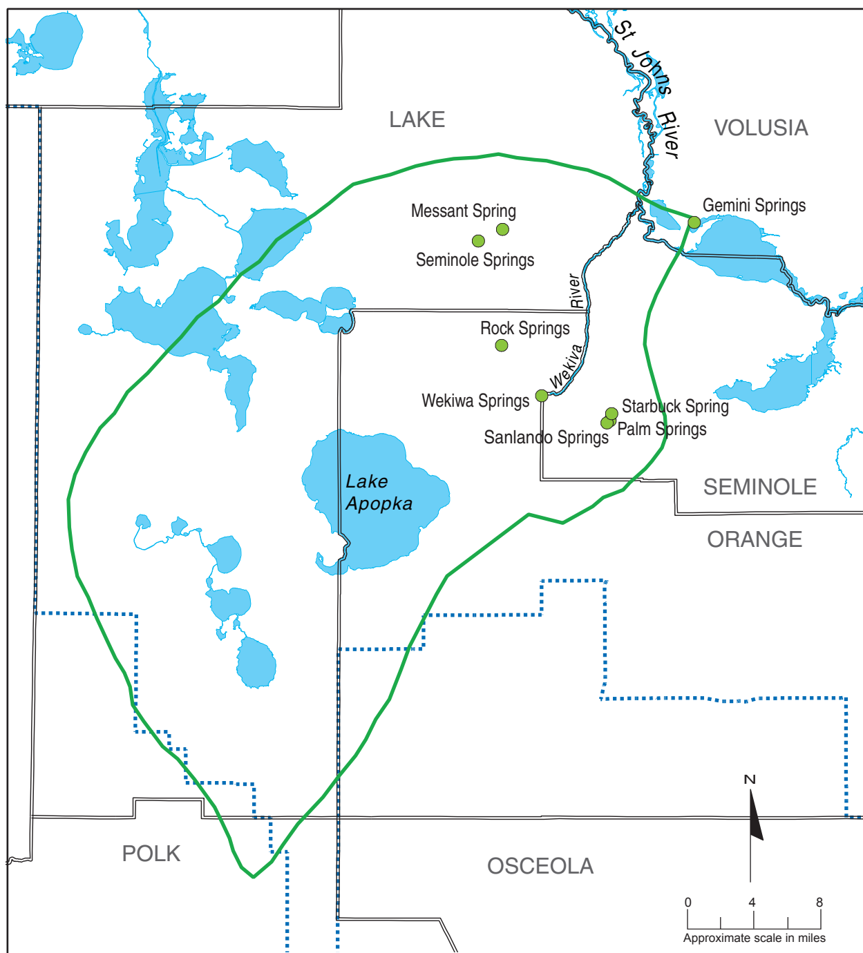
Figure 2. Wekiva groundwater basin study area (from Tibbals 1990)
