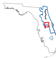
Figure 2. Wekiva groundwater basin study area (from Tibbals 1990)
