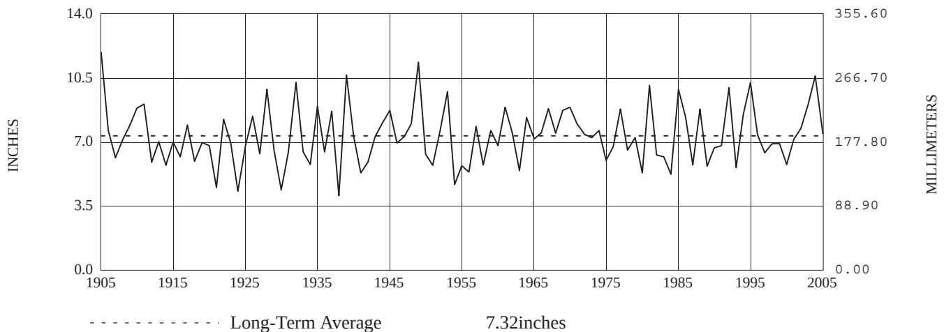
FLORIDA PRECIPITATION AUGUST, 1905-2005
