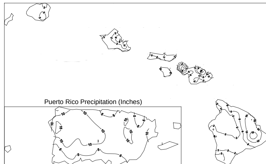
Hawaii Precipitation (Inches) August 2005
