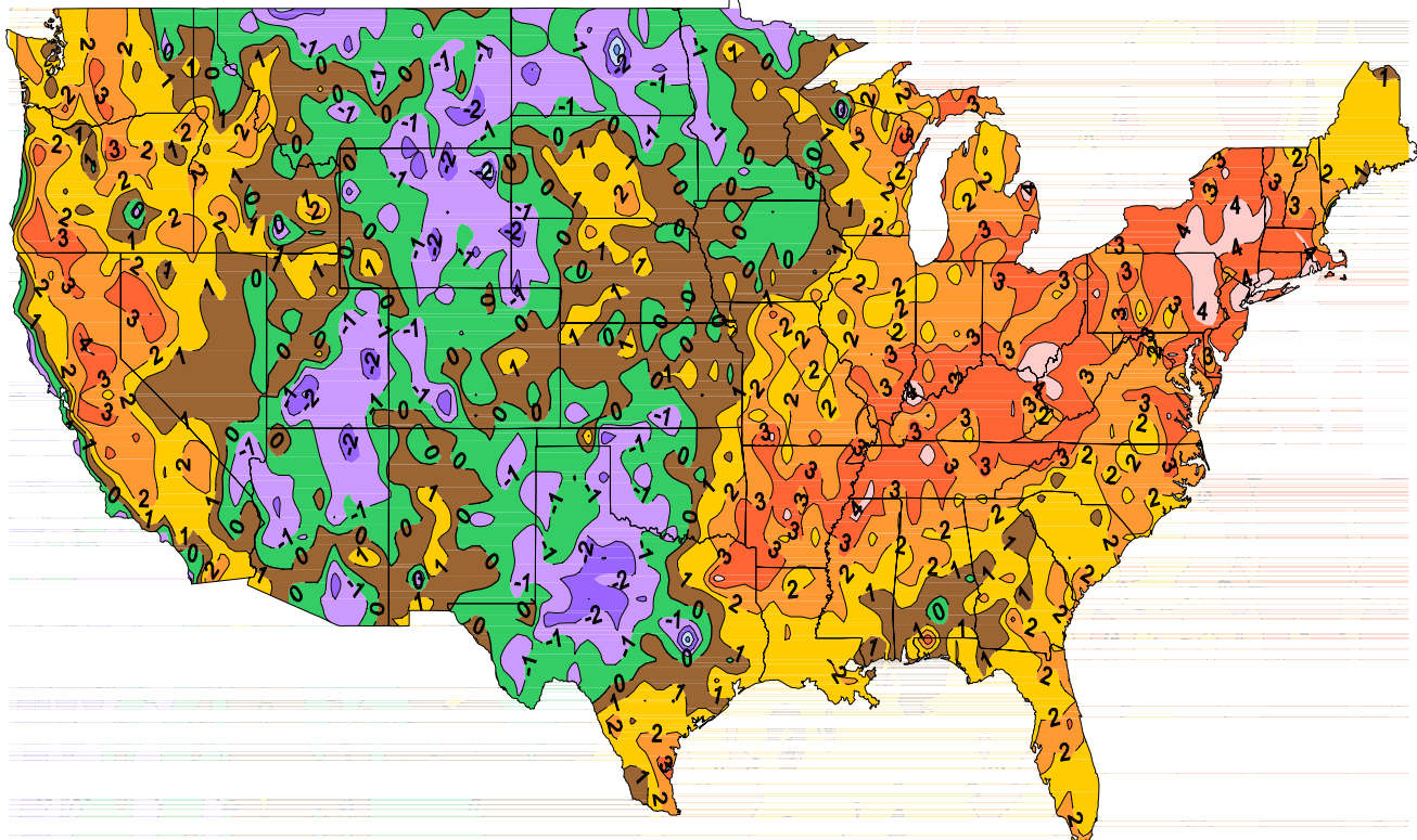
Departure of Average Temperature from Normal (Degrees F) August 2005
