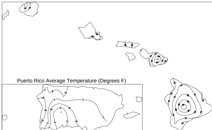
Hawaii Average Temperature (Degrees) August 2005
