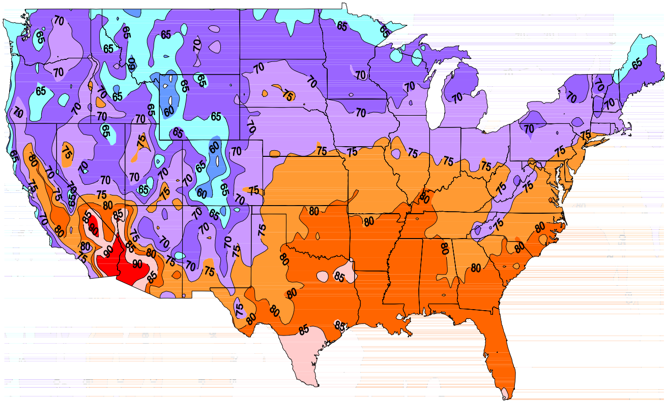
Average Temperature (Degrees F) August 2005
