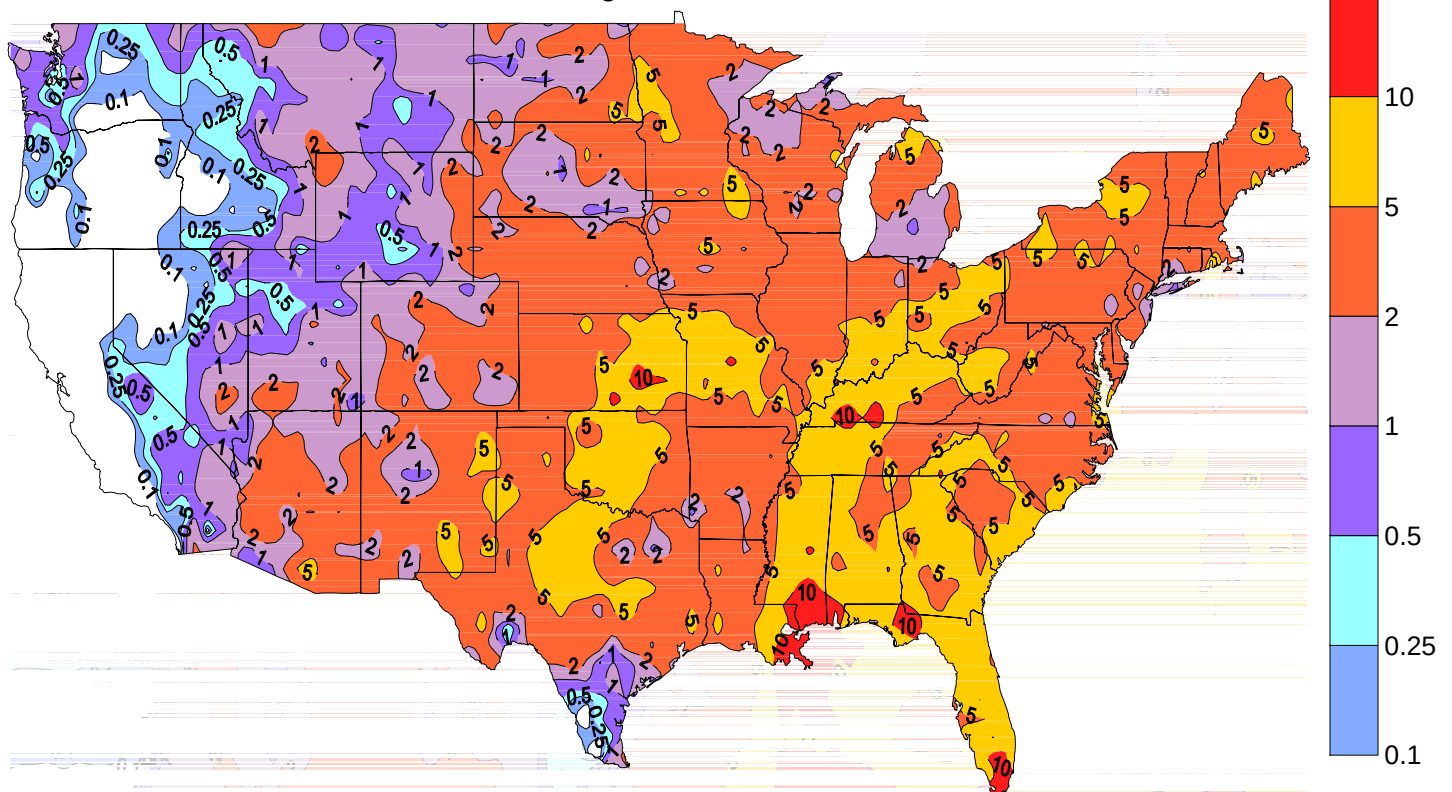
Percent of Normal August 2005
