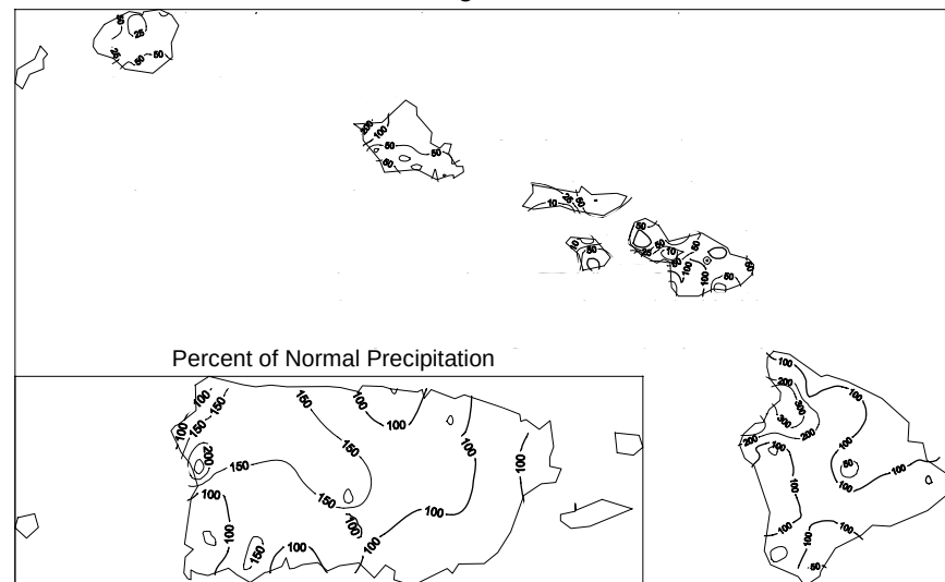
Hawaii Percent of Normal Precipitation August 2005
