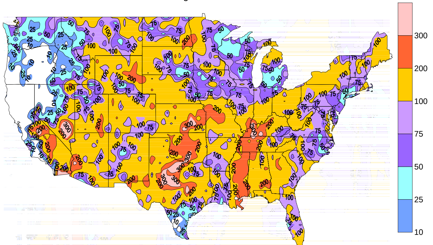
Percent of Normal August 2005
