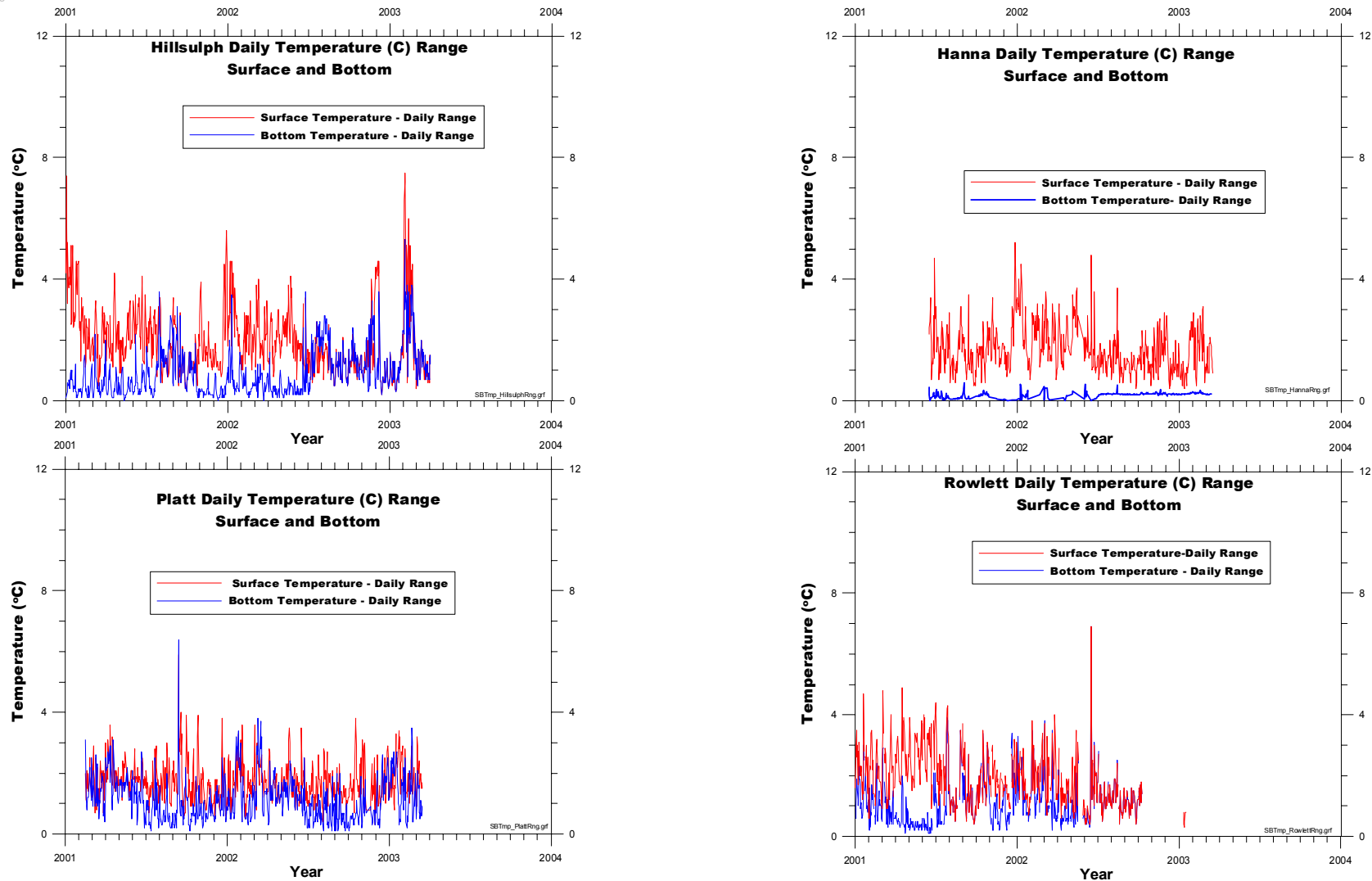
Figure 3-33. Daily ranges of water temperatures (maximum – minimum) for surface and bottom waters at four data recorders in the Hillsborough River operated by the USGS.
