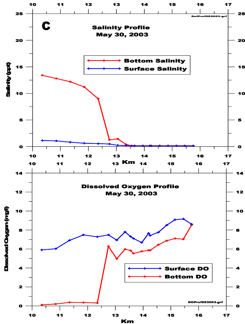
Figure 3-24 C and D. Longitudinal gradients of surface and bottom salinity and dissolved oxygen concentrations in the lower river between kilometer 10 and the dam for May 30, 2003 and February 19, 2003.
