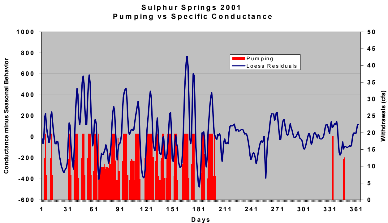
Figure 2-26. Residual values for conductance vs. day of the year and pumpage from Sulphur Springs for 2001.
