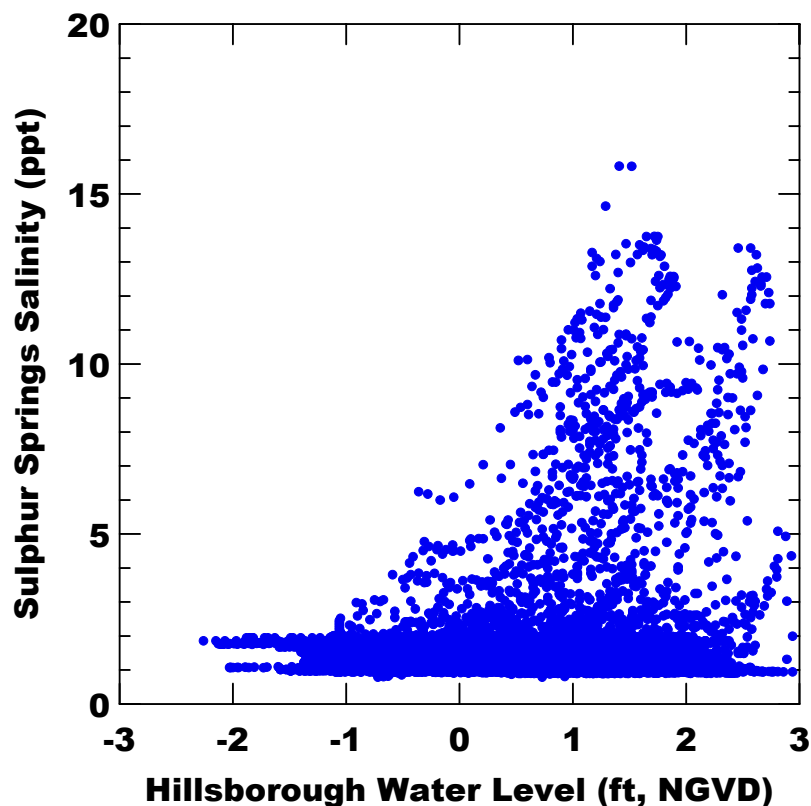
Figure 5-8. Relation between 15-minute values for water levels in the lower river and salinity at the recorder in the upper spring run for flows between 10 and 18 cfs from the spring pool.
