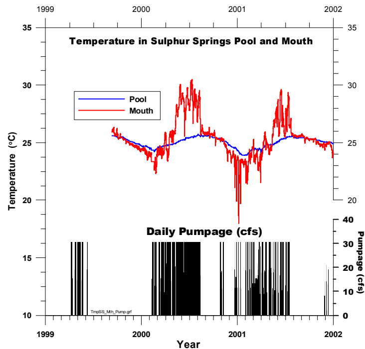
Figure 3-27. Comparison of water temperatures in Sulphur Springs pool and the data recorder at the mouth of the spring run over withdrawals from the spring pool.
