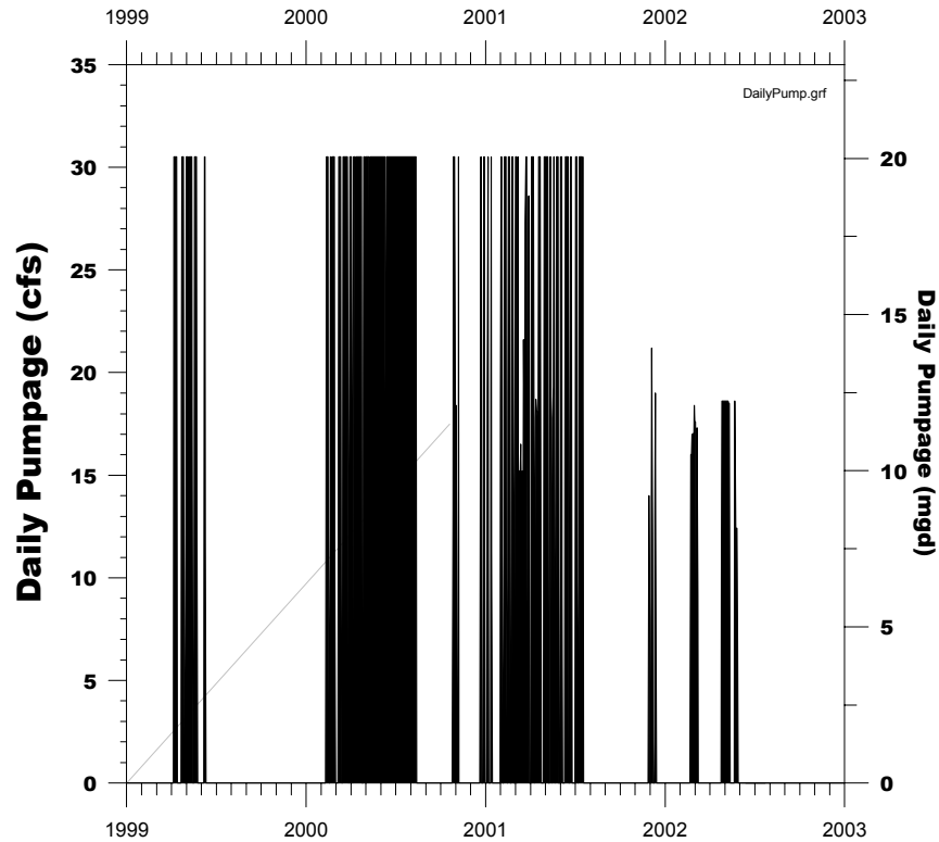
Figure 2-11. Average daily pumpage from Sulphur Springs 1999-2002.
