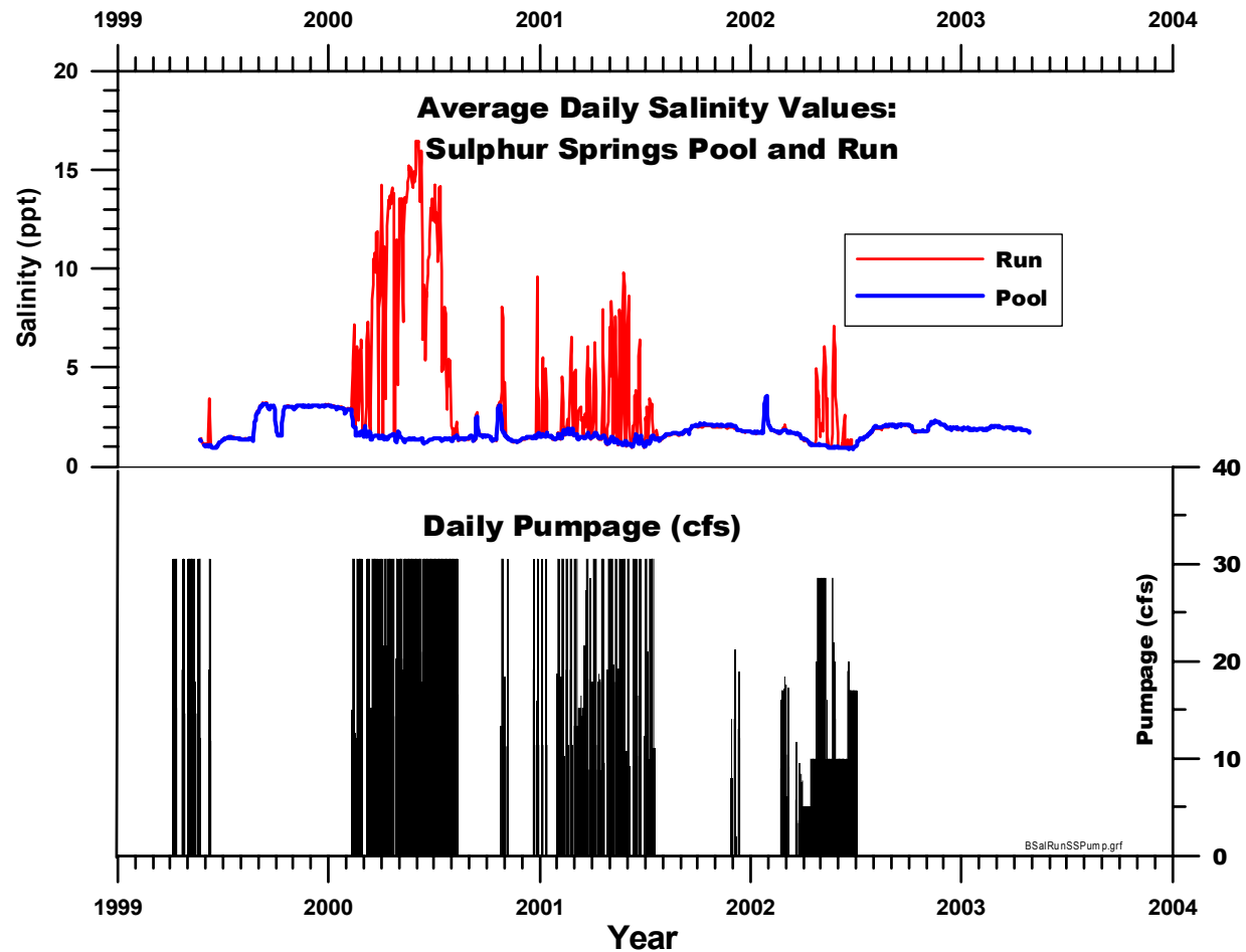
Figure 3-5. Average daily salinity values for the spring pool and the data recorder in the upper spring run over pumpage from the pool for 1999 – 2002.
