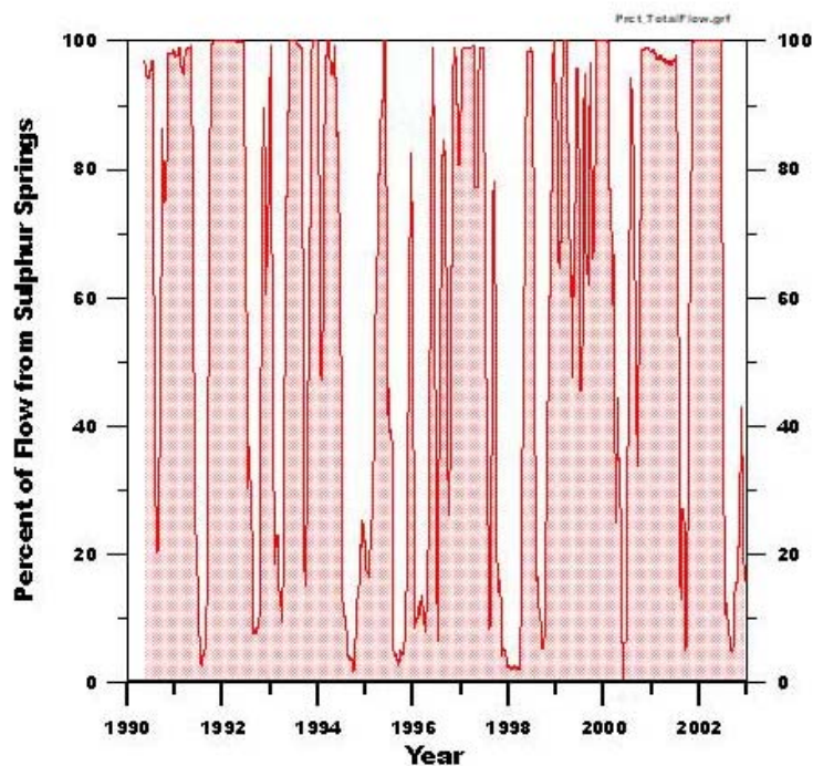
Figure 3-11. Time series of percent of daily gaged inflow to the lower river comprised by flow from Sulphur Springs.
