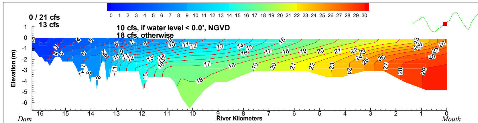
Figure 5-21. Two-dimensional plot of salinity distributions for inflows of 13 cfs of springwater at the dam and 18 cfs of springwater at Sulphur Springs when water levels in river above 0.0 feet; switching to 21 cfs at the dam and 10 cfs at Sulphur Springs when river stage goes below 0 feet NGVD. (Scenario 13)
