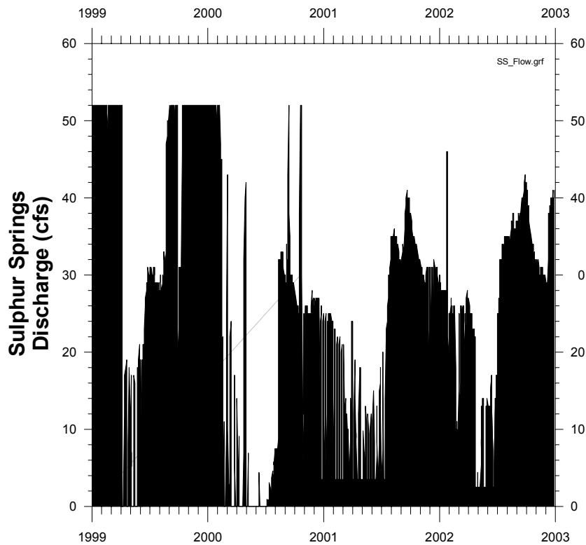
Figure 2-12. Daily discharge from Sulphur Springs 1999 - 2002.
