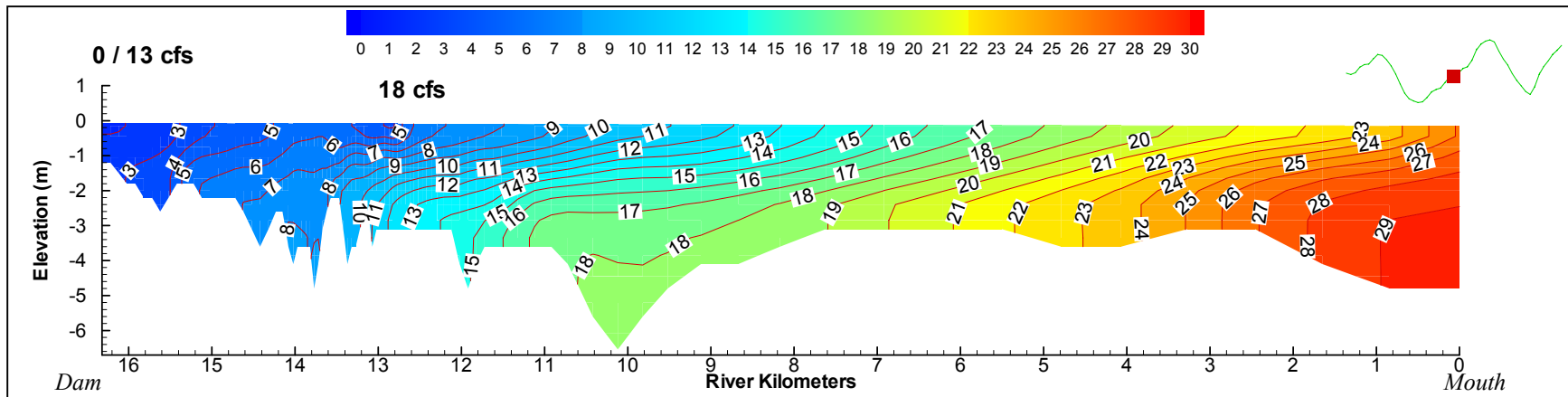
Figure 5-17. Two-dimensional plot of salinity distributions for inflows of 13 cfs of springwater at the dam and 18 cfs of springflow at Sulphur Springs. (Scenario 9)
