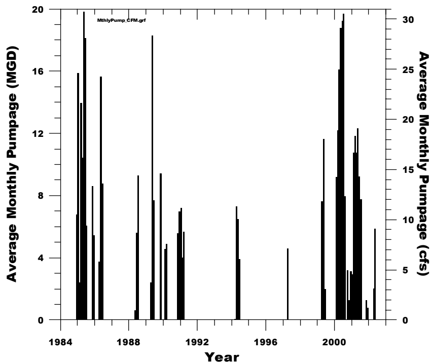
Figure 2-10. Average monthly pumpage rates from Sulphur Springs for 1984-2002.
