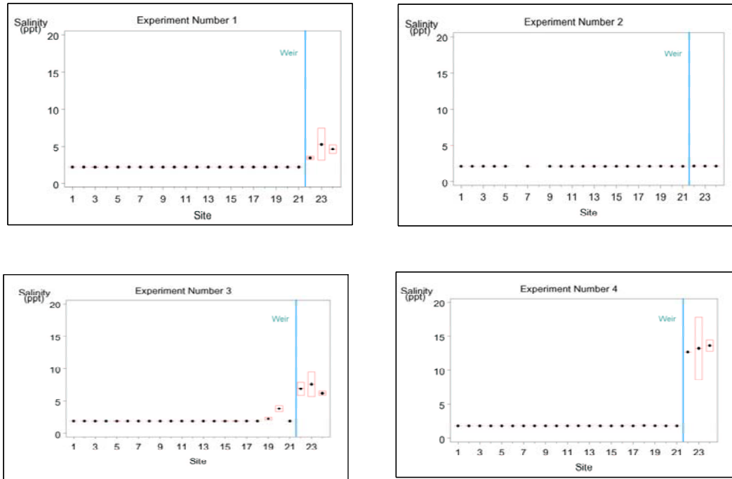
Figure 5-3. A – D. Box and whisker plots for salinity measurements at 23 stations in the upper and lower spring run for six flow experiments. Data include all salinity values from the water column (top to bottom) (2 pages).
