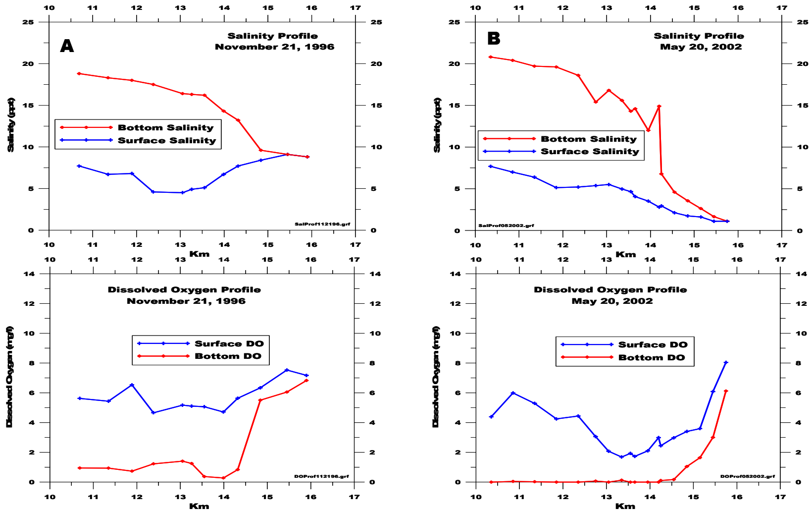
Figure 3-24 A and B. Longitudinal gradients of surface and bottom salinity and dissolved oxygen concentrations in the lower river between kilometer 10 and the dam for November 21, 1996 and May 20, 2002.
