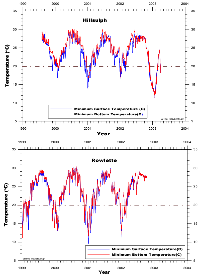
Figure 3-31. Time series of surface and bottom water temperatures at four data recorders in the Lower Hillsborough River operated by the USGS.
