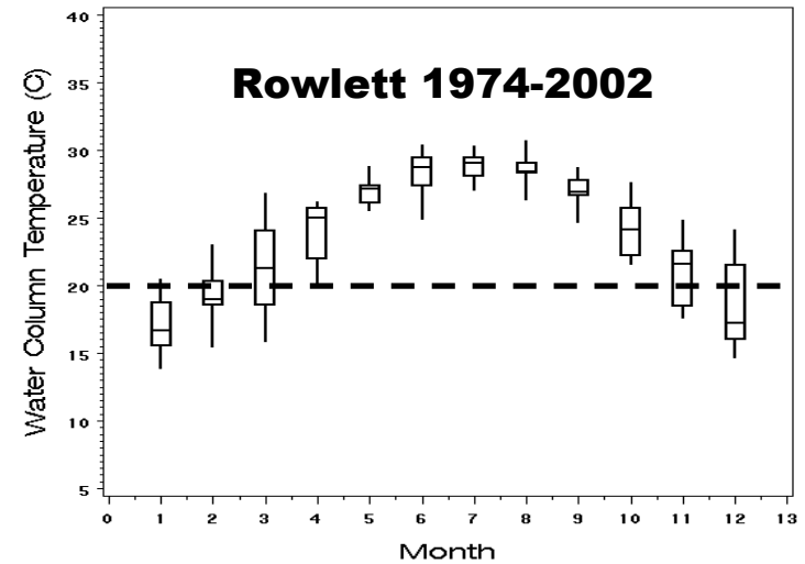
Figure 3-28. Box and whisker plots of monthly water temperatures for the periods of record at four sites monitored by the EPCHC ambient monitoring program (all depths combined).
