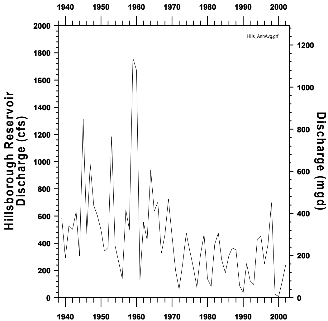
Figure 3-8. Average yearly flows to the lower river from the Hillsborough River Reservoir.
