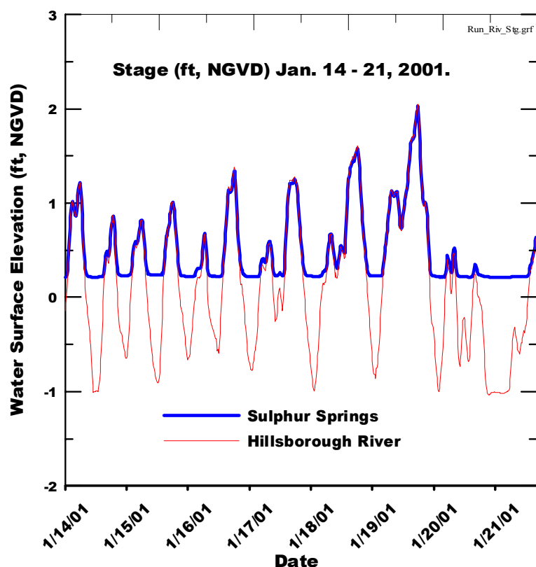
Figure 3-2. Time series graph of water levels in upper spring run and river near the moth of the spring during a period of normal flow from the spring pool (January 14 – 21, 2001).
