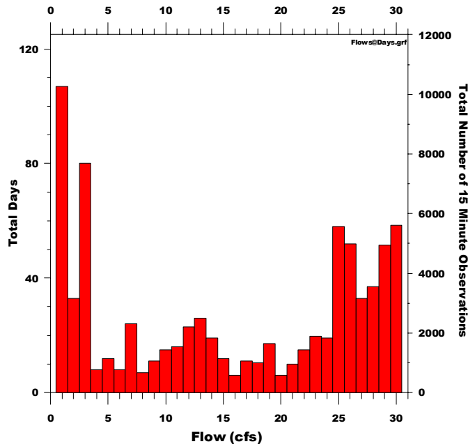
Figure 5-4. Number of days in 1 cfs flow classes for flows from Sulphur Springs pool. Data restricted to periods when there was no flow to the lower river from the Hillsborough River reservoir.
