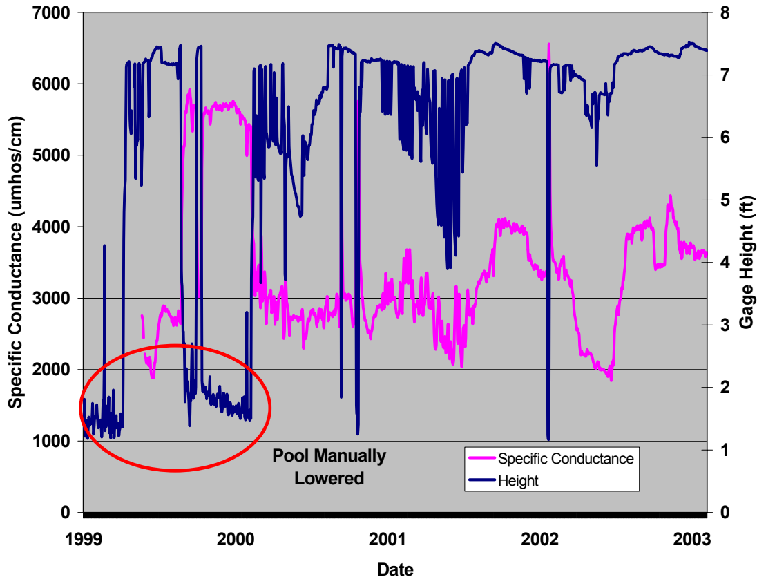
Figure 2-23. Average daily values of water levels and specific conductance for Sulphur Springs Pool for 1999 through 2002.
