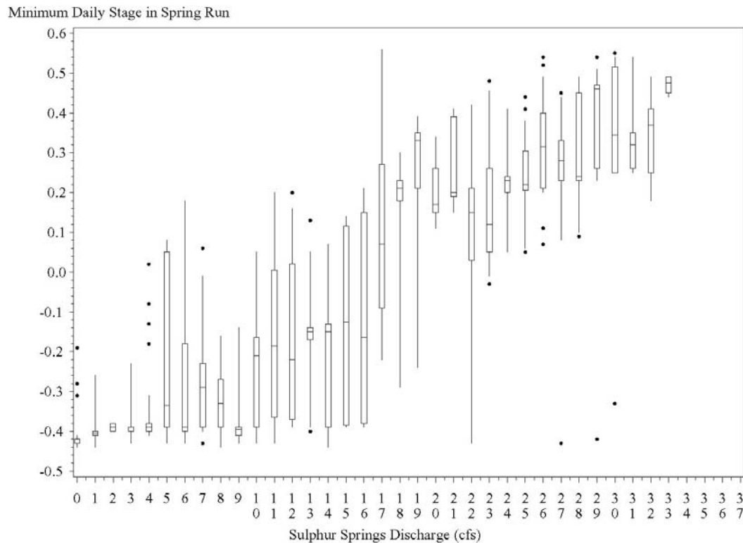
Figure 5-10. Box and whisker plot of daily minimum water levels in the upper spring run in 1 cfs flow classes from Sulphur Springs pool.
