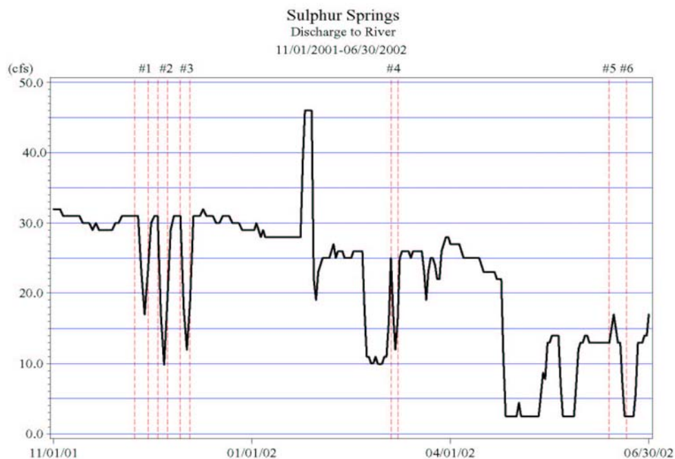
Figure 5-1. Average daily flows from Sulphur Springs Pool for November 2001 through June 2002 with reference lines denoting periods of experimental flow releases.
