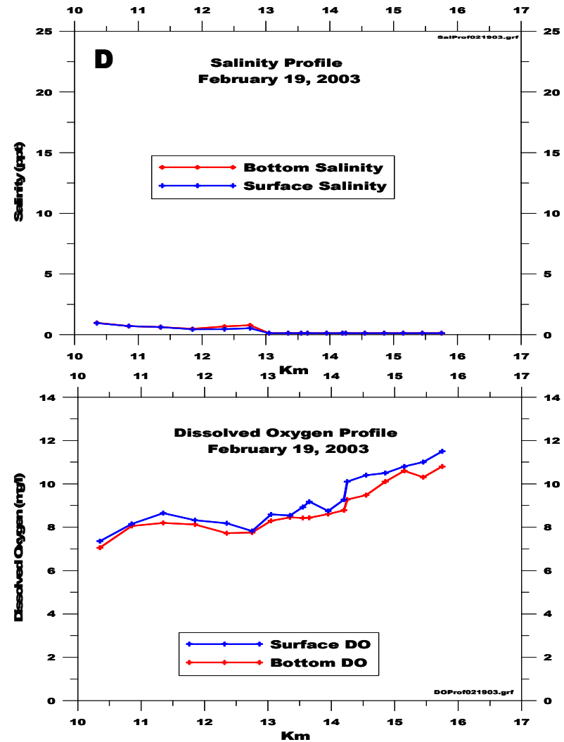
Figure 3-24 C and D. Longitudinal gradients of surface and bottom salinity and dissolved oxygen concentrations in the lower river between kilometer 10 and the dam for May 30, 2003 and February 19, 2003.
