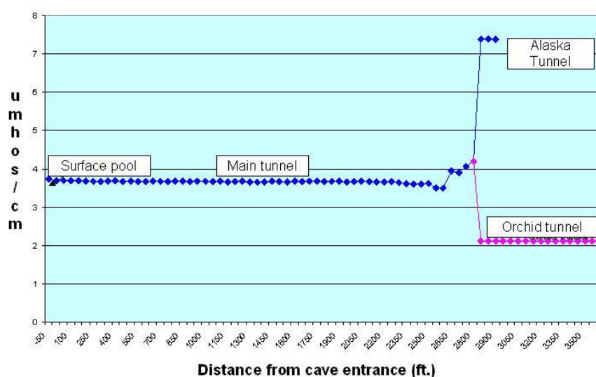
Figure 2-22A. Specific conductance in the Sulphur Springs cave system on November 15, 1998. Adapted from Schrueder, Inc. Used with permission of the City of Tampa.
