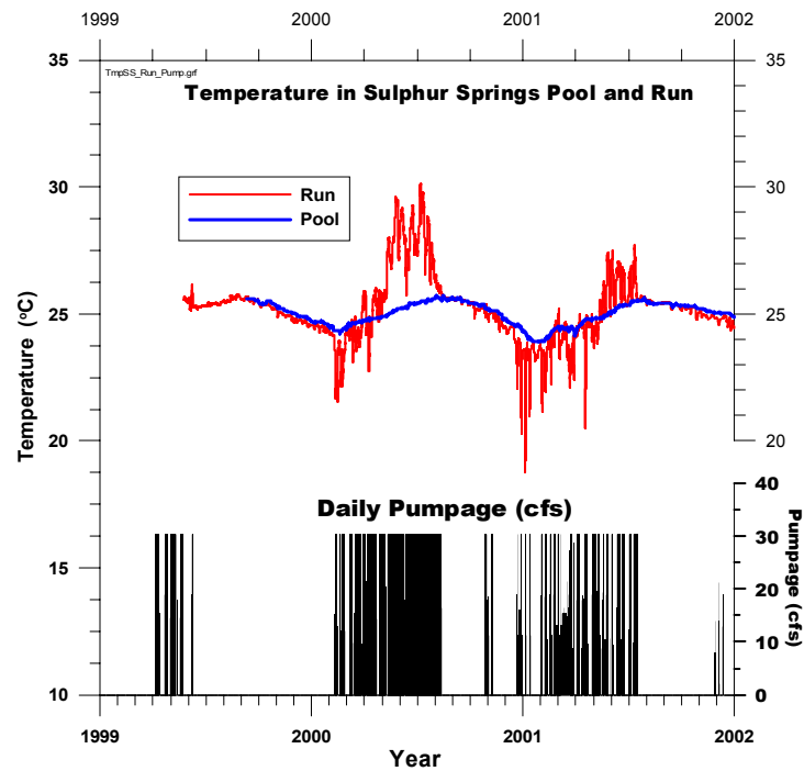
Figure 3-26. Comparison of water temperatures in Sulphur Springs pool and the data recorder in the upper spring run over withdrawals from the spring pool.
