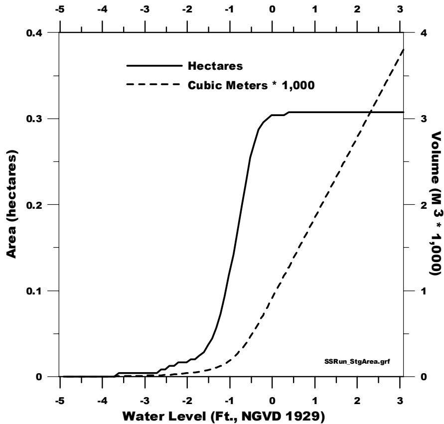
Figure 2-8. Surface area and volume of Sulphur Springs Run as a function of water level in the spring run.
