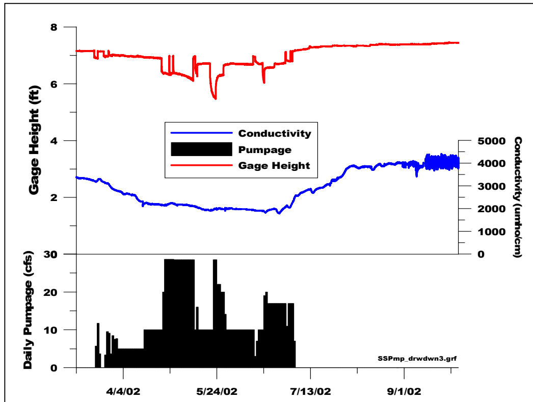
Figure 2-27. Response of water levels and conductance to withdrawals after modification of water diversion facilities at Sulphur Springs, March - September, 2002.
