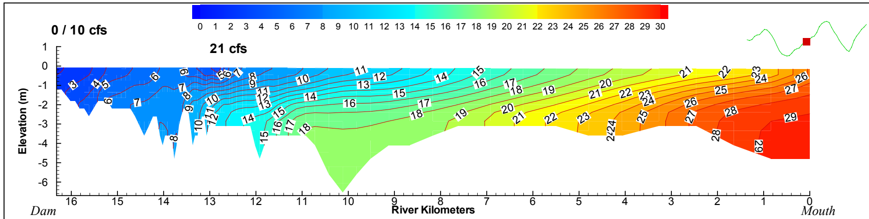
Figure 3-20. Two-dimensional plot of salinity distributions for inflows of 0 cfs of river water and 10 cfs of spring water at the dam and 21 cfs of springflow at Sulphur Springs.
