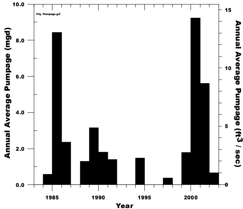
Figure 2-9. Average annual pumpage rates from Sulphur Spring by the City of Tampa for 1984-2002.
