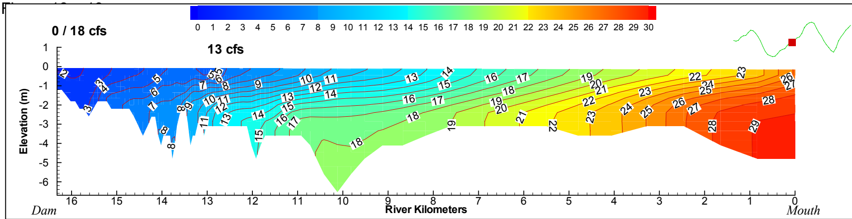
Figure 5-18. Two-dimensional plot of salinity distributions for inflows of 18 cfs of springwater at the dam and 13 cfs of springflow at Sulphur Springs. (Scenario 10)
