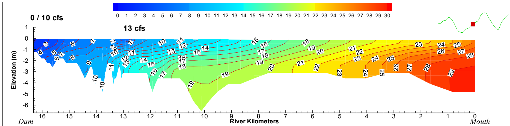
Figure 5-15. Two-dimensional plot of salinity distributions for inflows of 10 cfs of springwater at the dam and 13 cfs of springflow at Sulphur Springs. (Scenario 7)
