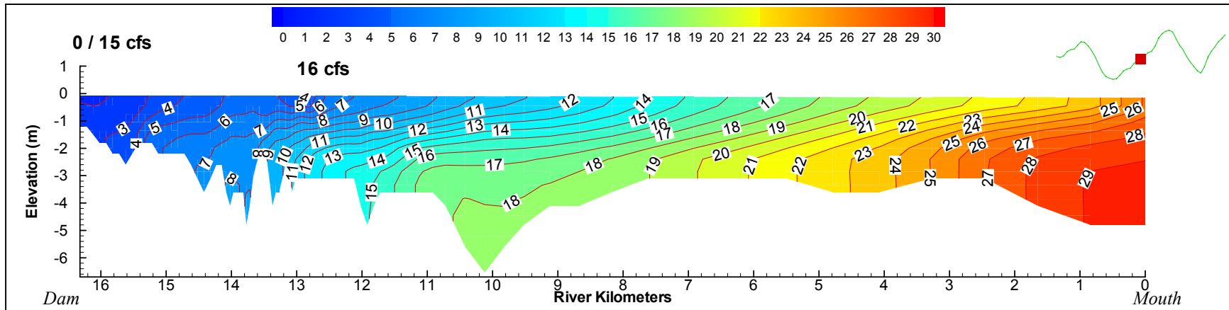
Figure 3-21. Two-dimensional plot of salinity distributions for inflows of 0 cfs of river water and 15 cfs of spring water at the dam and 16 cfs of springflow at Sulphur Springs.
