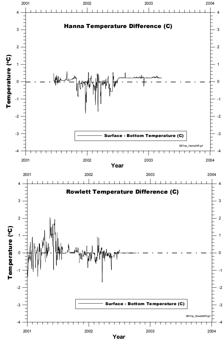
Figure 3-32. Vertical temperature differentials (surface minus bottom) at four data recorders in the Hillsborough River operated by the USGS.
