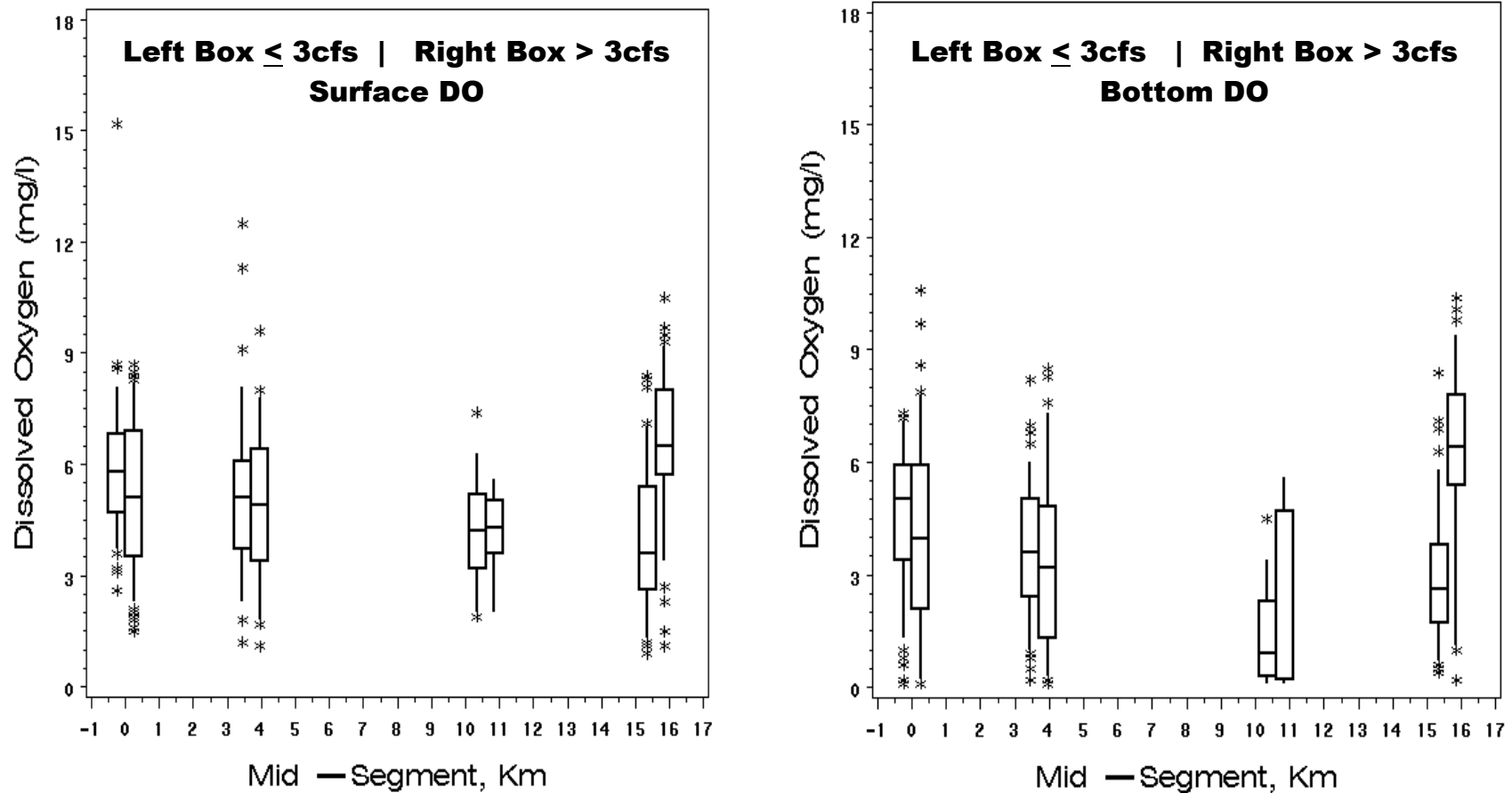
Figure 3-23. Box and whisker plots of surface and bottom dissolved oxygen concentrations for the periods of record at EPCHC ambient monitoring stations on the Lower Hillsborough River for flow and no flow conditions.
