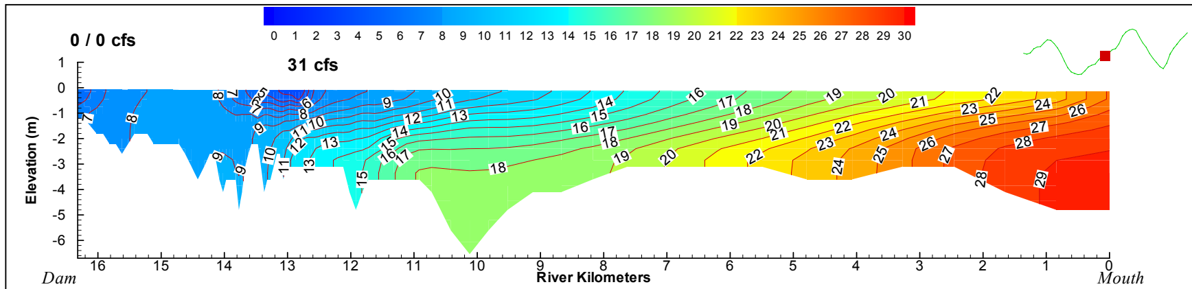
Figure 5-12. Two-dimensional plot of salinity distributions for inflows of 0 cfs of springwater at the dam and 31 cfs of springflow at Sulphur Springs.
