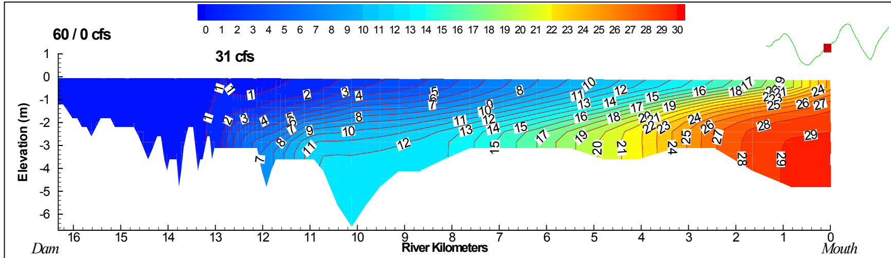
Figure 3-18. Two-dimensional plot of salinity distributions for inflows of 60 cfs of river water at the dam and 31 cfs of spring water at Sulphur Springs.
