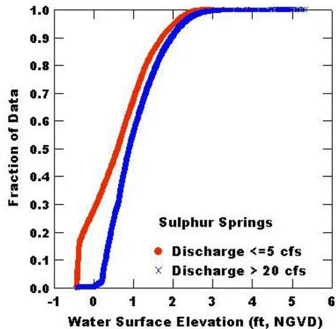
Figure 3-3. Stage duration curves for water levels in the upper spring run for periods of normal flow ( > 20 cfs) and low flow ( < 5 cfs).
