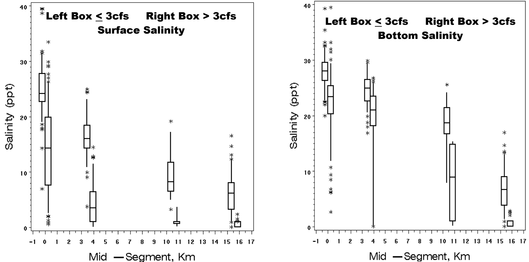
Figure 3-14. Box and whisker plots of surface and bottom salinity values at the EPCHC ambient monitoring stations on the Lower Hillsborough River for flow and no flow conditions. Data taken from the period of record at each station.
