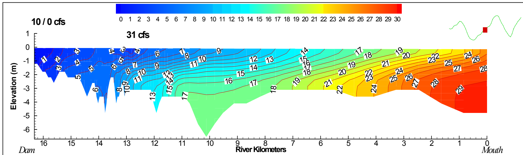
Figure 3-17. Two-dimensional plot of salinity distributions for inflows of 10 cfs of river water at the dam and 31 cfs of spring water at Sulphur Springs.
