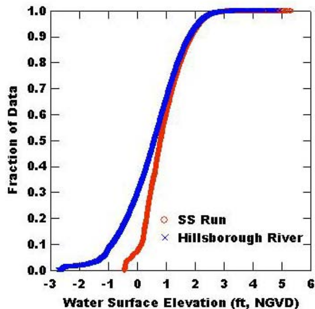
Figure 3-1. Stage duration curves of water levels in the upper spring run and the Hillsborough River near the mouth of the spring.
