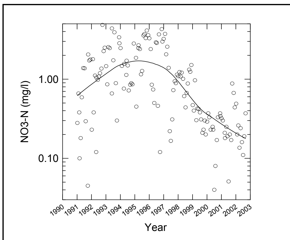
Figure 2-28. Temporal trend in nitrate nitrogen in the Sulphur Springs Pool for 1991-2003 (three values not shown).
