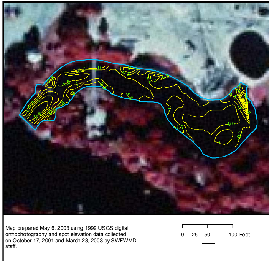
Figure 2-7. Bathymetric map of Sulphur Springs Run. Yellow lines are one-half foot contours relative to NGVD, 1929.
