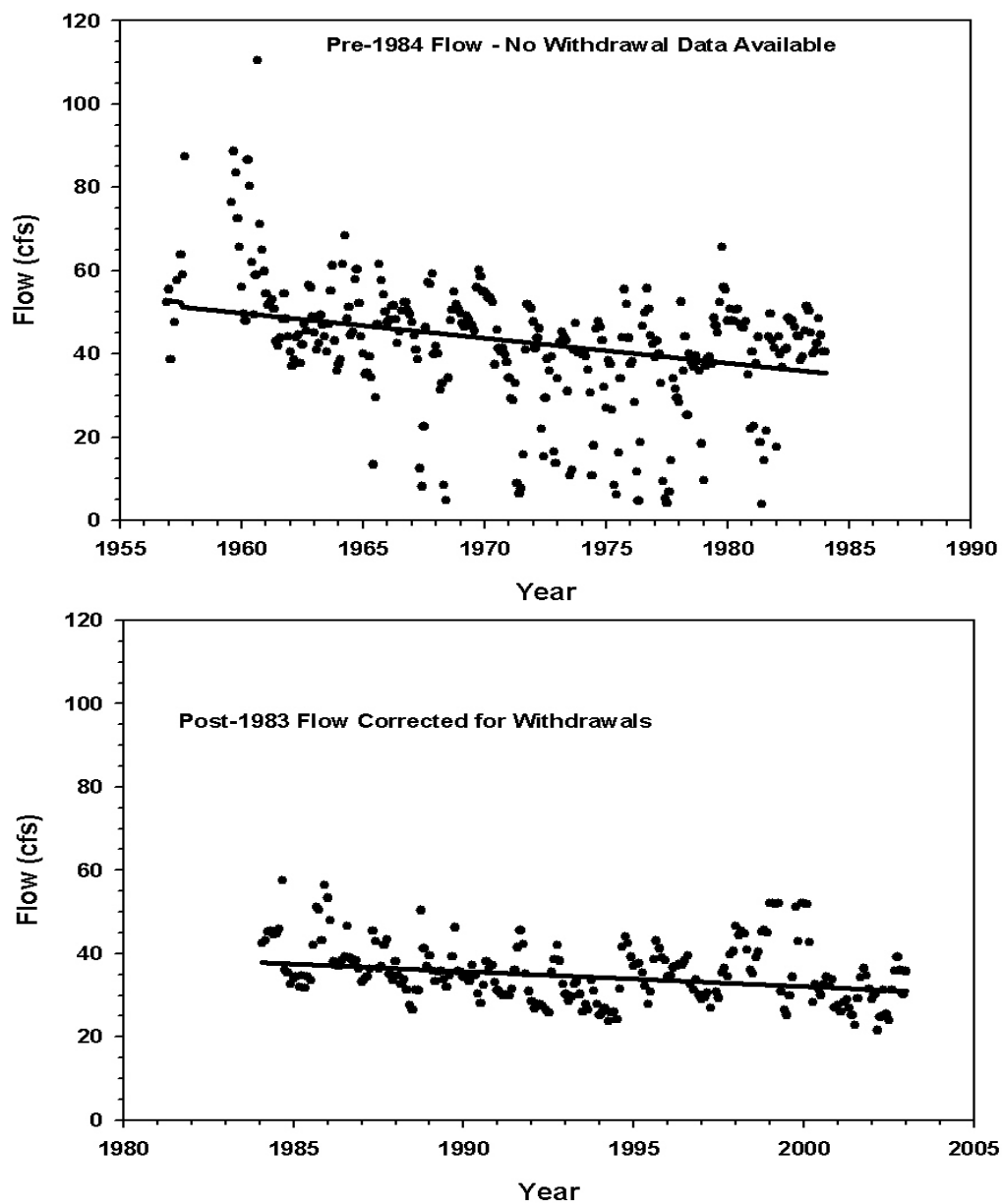
Figure 2-19 . Temporal trend of monthly Sulphur Springs flows: corrected and uncorrected for withdrawals. Kendall-Theil slope shown.
