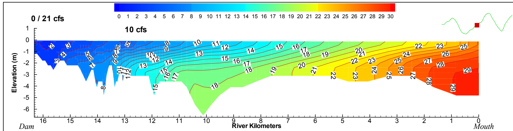
Figure 5-19. Two-dimensional plot of salinity distributions for inflows of 21 cfs of springwater at the dam and 10 cfs of springflow at Sulphur Springs. (Scenario 11)
