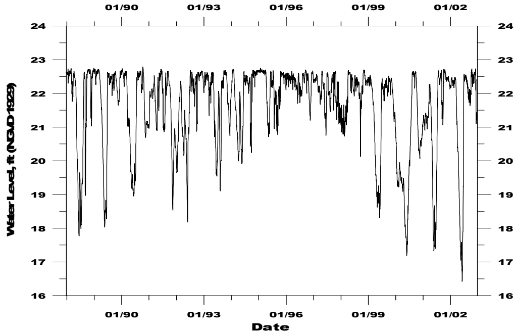
Figure 5-22. Average daily water levels in the Hillsborough River reservoir for 1988-2003.
