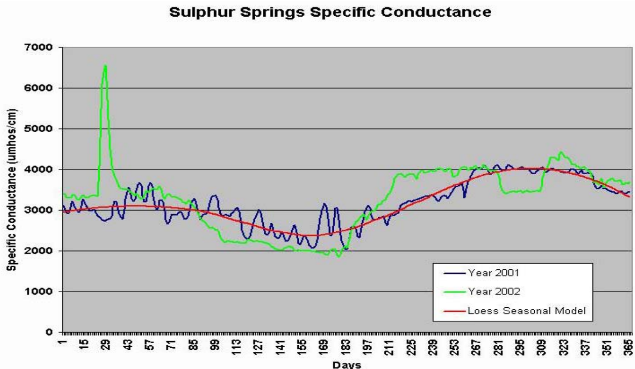
Figure 2-25. Average specific conductance values for each day of the year for 2001 and 2002 with a LOESS line fitted to the 2001 data.
