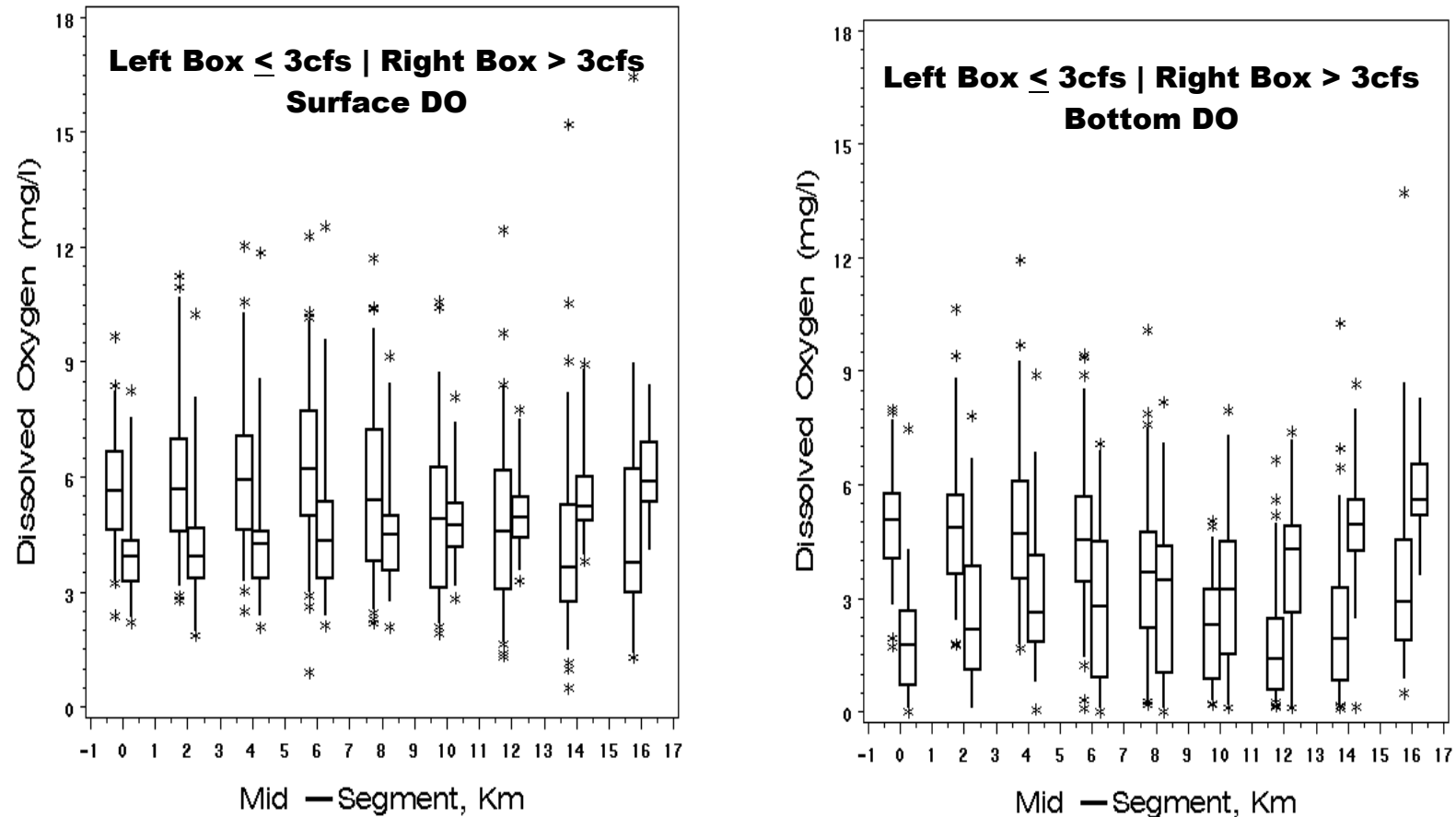
Figure 3-22. Box and whisker plots of surface and bottom dissolved oxygen concentrations in two-kilometer segments in the Lower Hillsborough River for flow and no flow conditions. Data taken from the HBMP and the EPCHC HIMP programs during 2000-2002.
