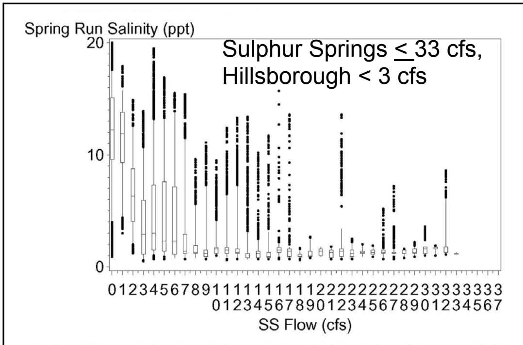
Figure 5-5. Box and whisker plot of 15 minute salinity measurements at the data recorder in the upper spring run. Data restricted to periods when there was no flow to the lower river from the Hillsborough River reservoir.
