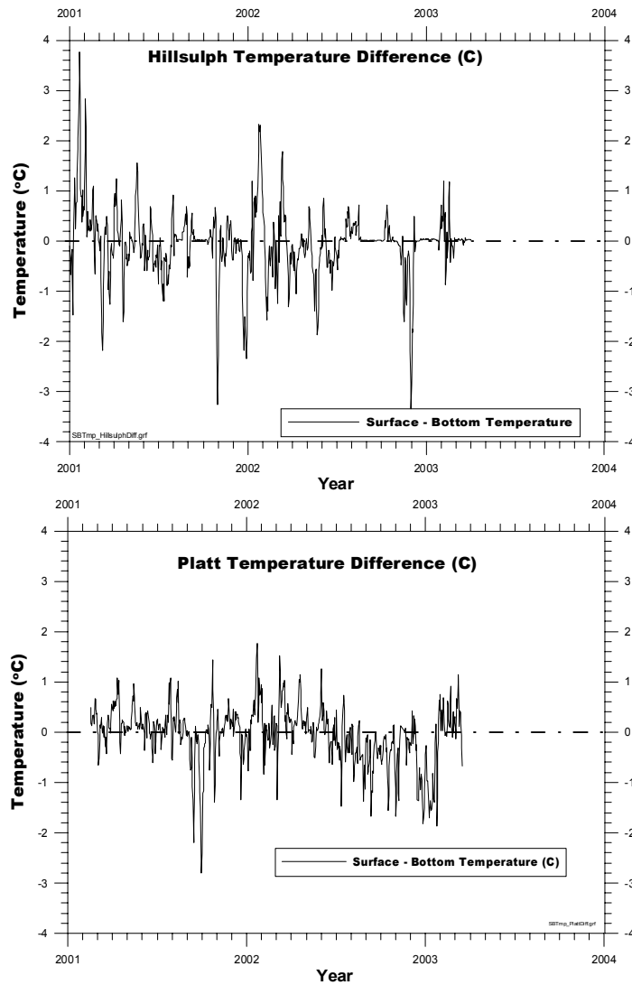
Figure 3-32. Vertical temperature differentials (surface minus bottom) at four data recorders in the Hillsborough River operated by the USGS.
