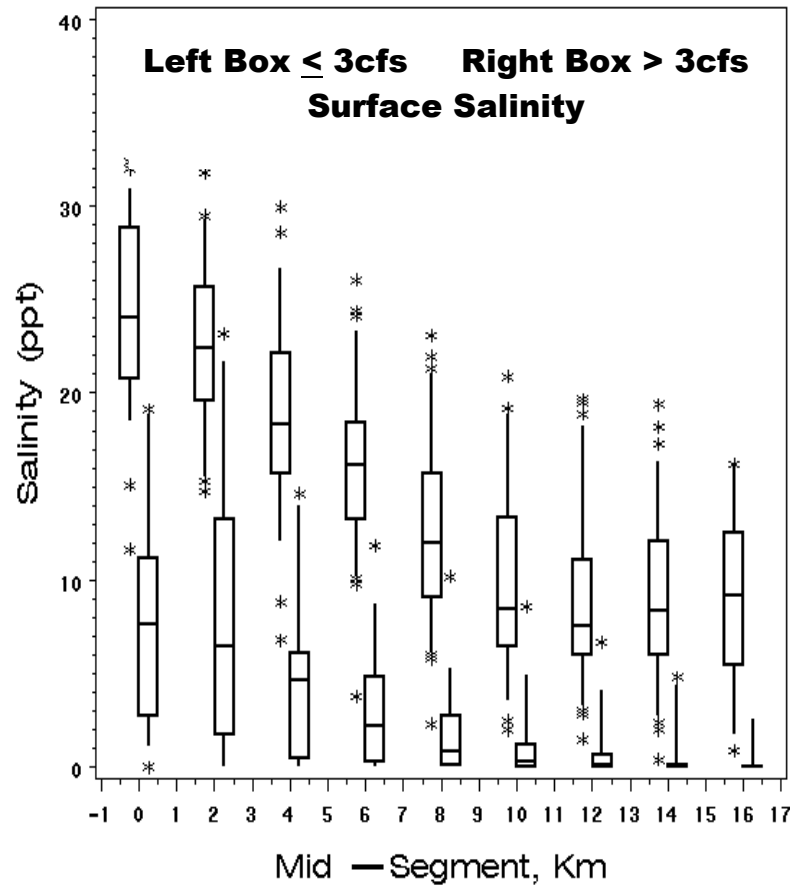
Figure 3-13. Box and whisker plots of surface and bottom salinity values in two kilometer segments in the Lower Hillsborough River for flow and no flow conditions. Data taken from the HBMP and the EPCHC HIMP programs for 2000 – 2002.
