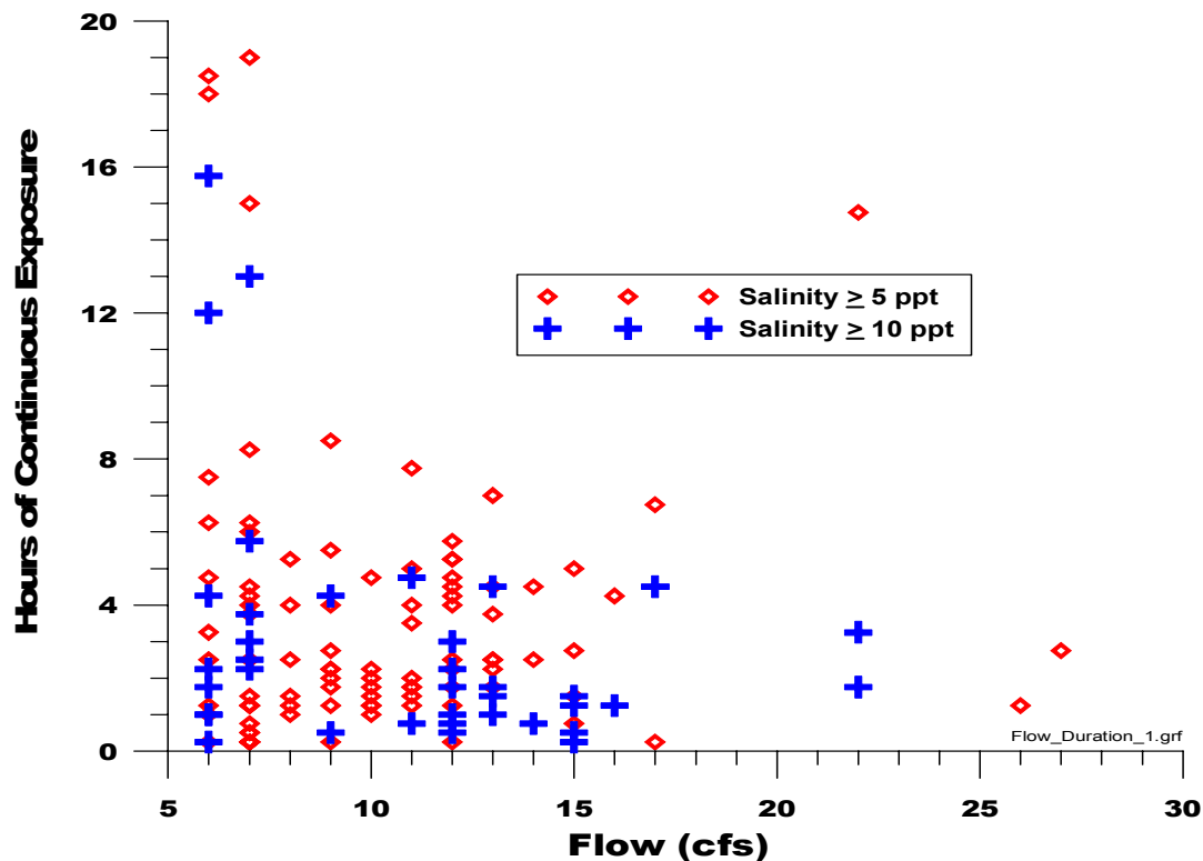
Figure 5-7. Duration of salinity incursions greater than or equal to 5 ppt or 10 ppt at the data recorder in upper spring run for 1 cfs flow classes from Sulphur Springs.
