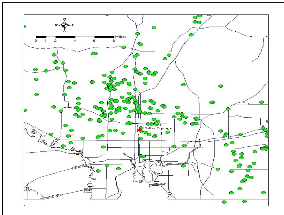
Figure 2-17. Known sinkholes locations near Tampa, Florida.
