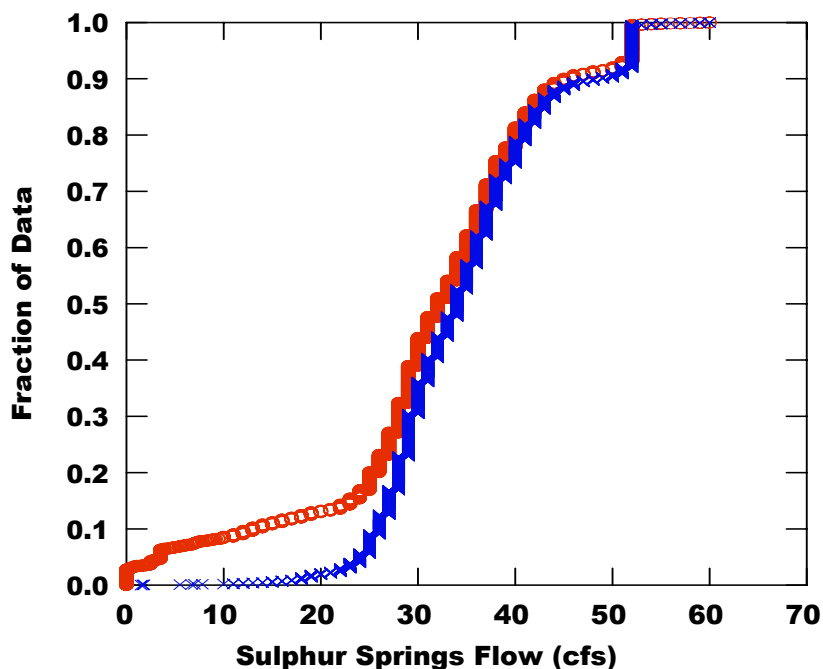
Figure 2-16. Flow duration curves for daily flow values from Sulphur Springs for days with no withdrawals (blue) and complete daily records (red) for 1991 – 2002.
