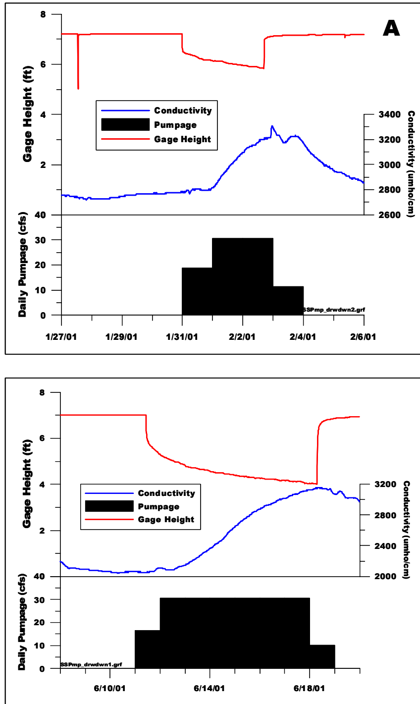
Figure 2-24. Water level and specific conductance response to withdrawals from the Sulphur Springs Pool for two periods during 2001.
