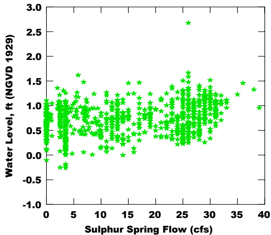
Figure 5-9. Relationships between daily mean, maximum, and minimum water levels in the upper spring run and flow from Sulphur Springs pool.
