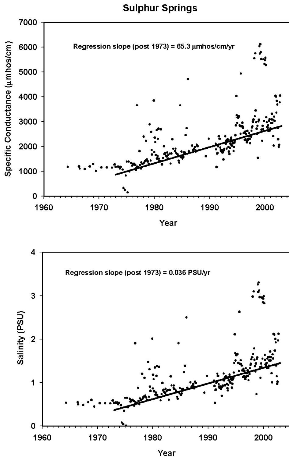
Figure 2-21. Temporal trend of specific conductance and salinity in the Sulphur Springs Pool. Kendall-Theil slope shown.
