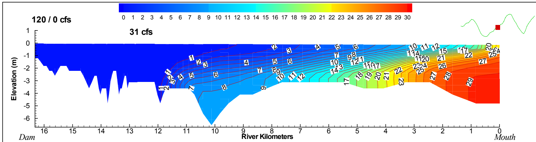
Figure 3.19. Two-dimensional plot of salinity distributions for inflows of 120 cfs of river water at the dam and 31 cfs of spring water at Sulphur Springs.
