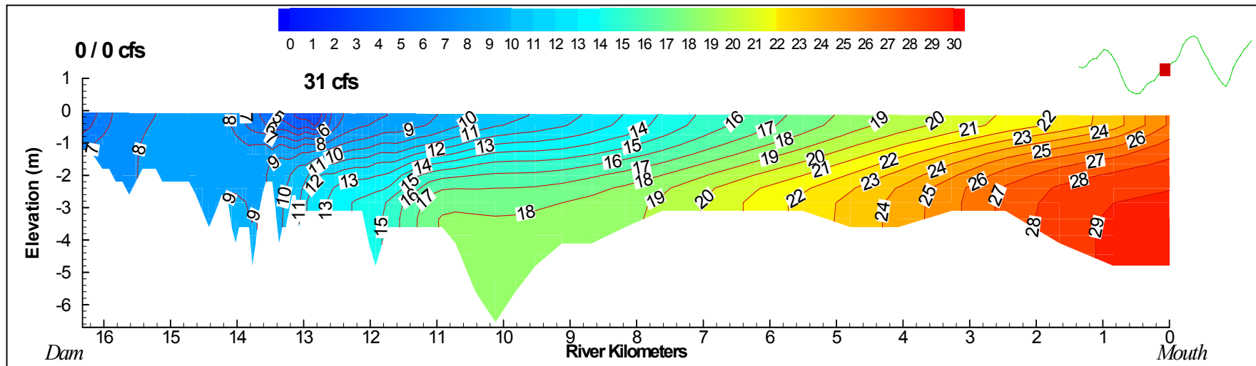
Figure 3-16. Two-dimensional plot of salinity distributions for inflows of 0 cfs at the dam and 31 cfs of springflow at Sulphur Springs.
