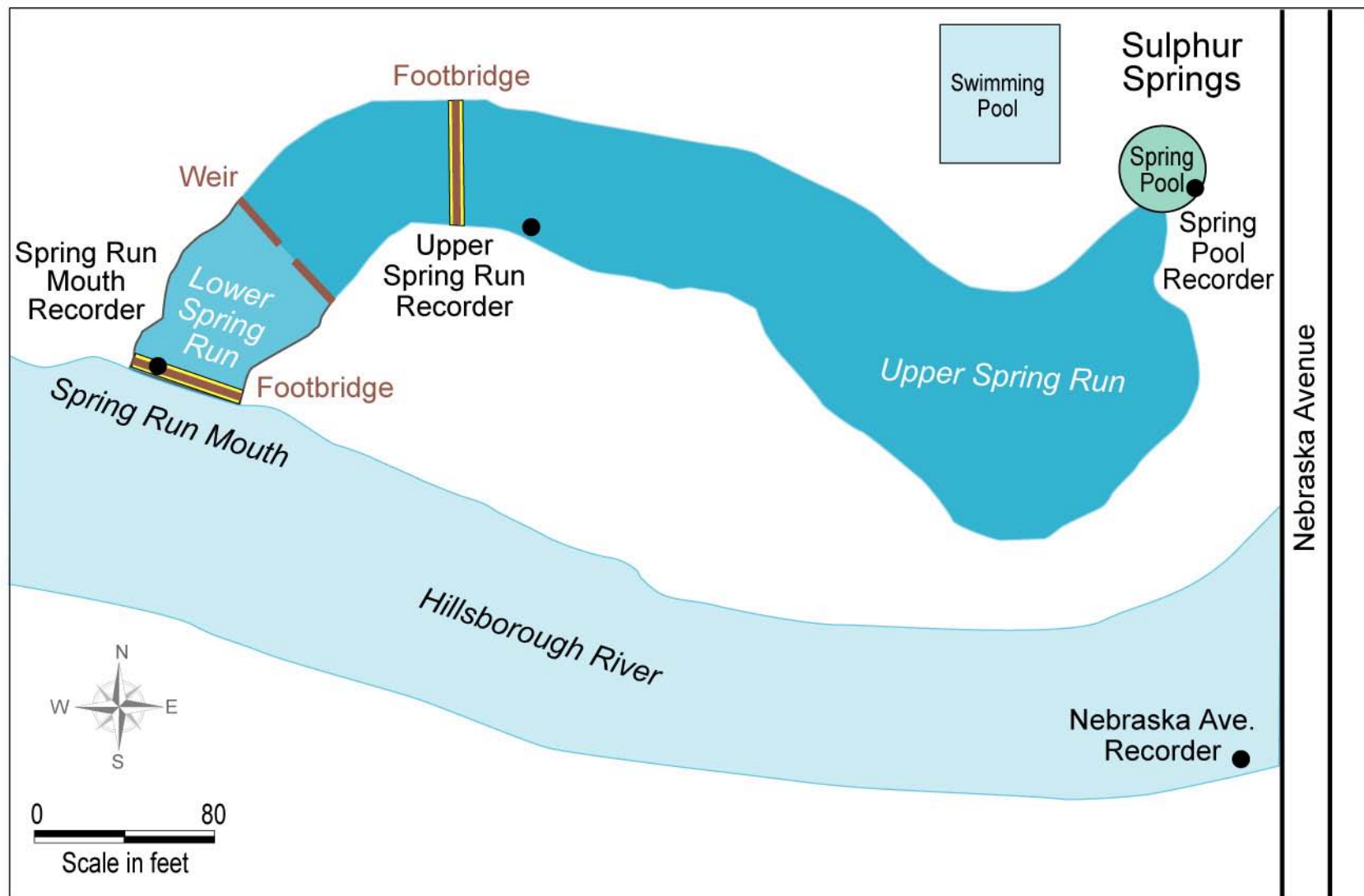
Figure 2-5. Diagram of Sulphur Springs showing the shoreline and structural features associated with the spring pool, spring run, and Lower Hillsborough River. Also shown are the locations of four recording gages operated by the U.S. Geological Survey.
