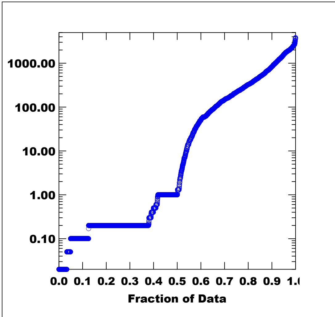
Figure 3-10. Flow Duration curve for daily flow values from the Hillsborough River Reservoir.
