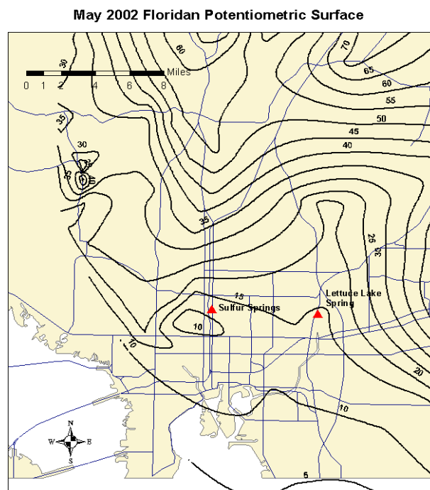
Figure 2-18 . Potentiometric surface of the Upper Florida aquifer near Sulphur Springs for May, 2002.
