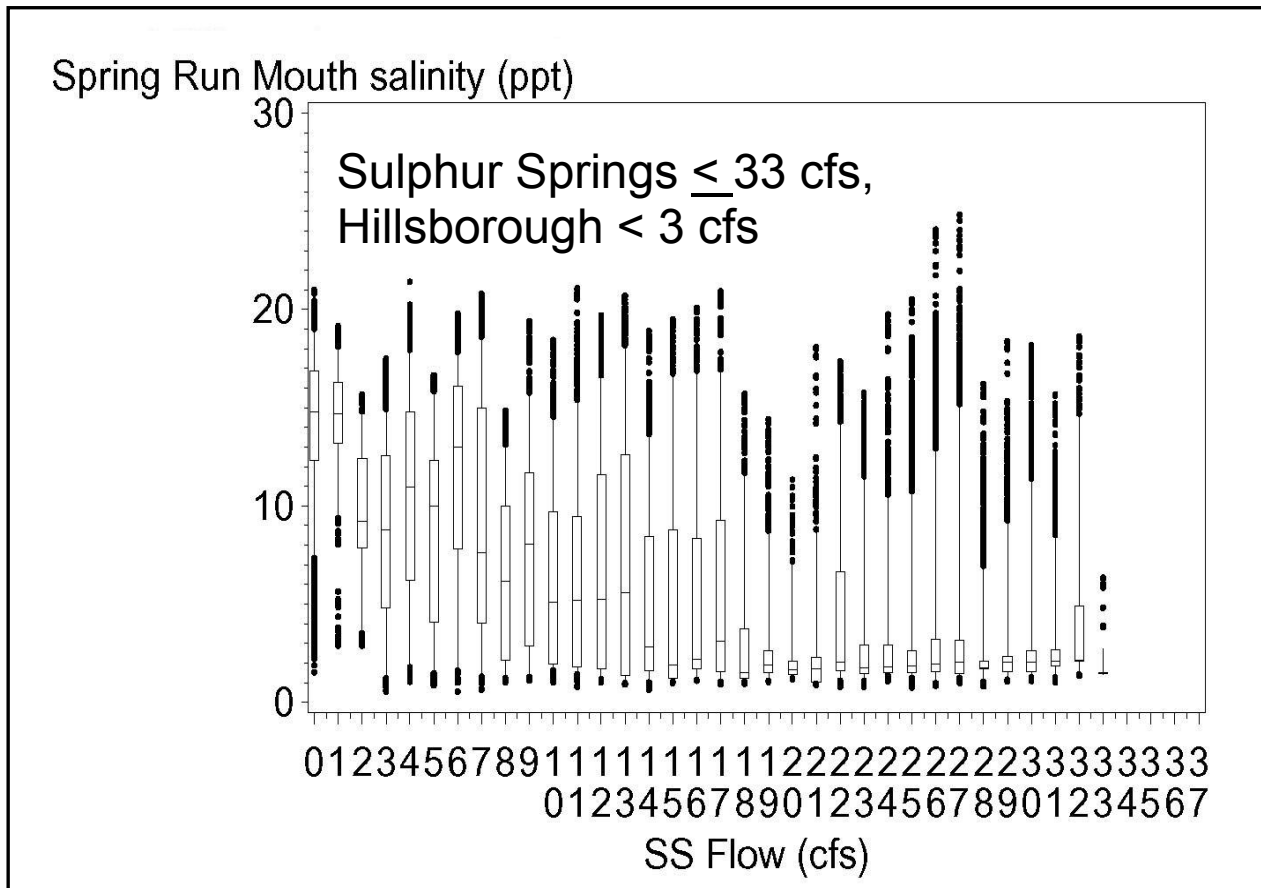
Figure 5-11. Box and whisker plot of 15 minute salinity measurements at the data recorder at the mouth of the spring run. Data restricted to periods when there was no flow to the lower river from the Hillsborough River reservoir.
