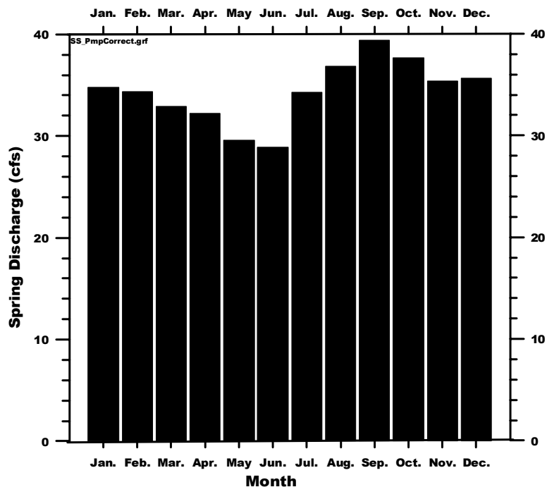
Figure 2-15. Average monthly flows from Sulphur Springs corrected for withdrawals for 1991 – 2002.
