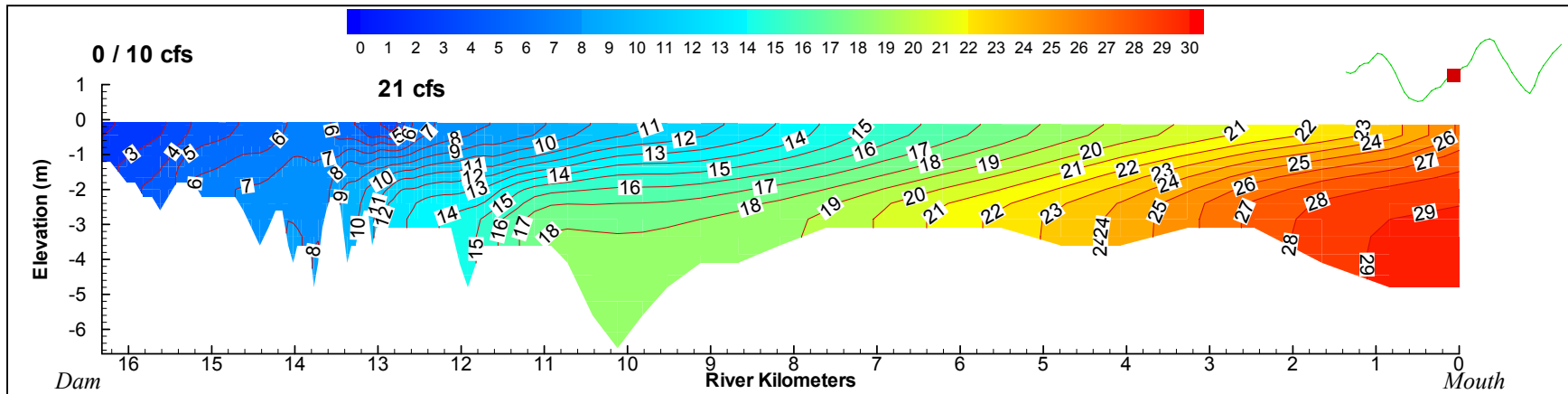
Figure 5-13. Two-dimensional plot of salinity distributions for inflows of 10 cfs of springwater at the dam and 21 cfs of springflow at Sulphur Springs.
