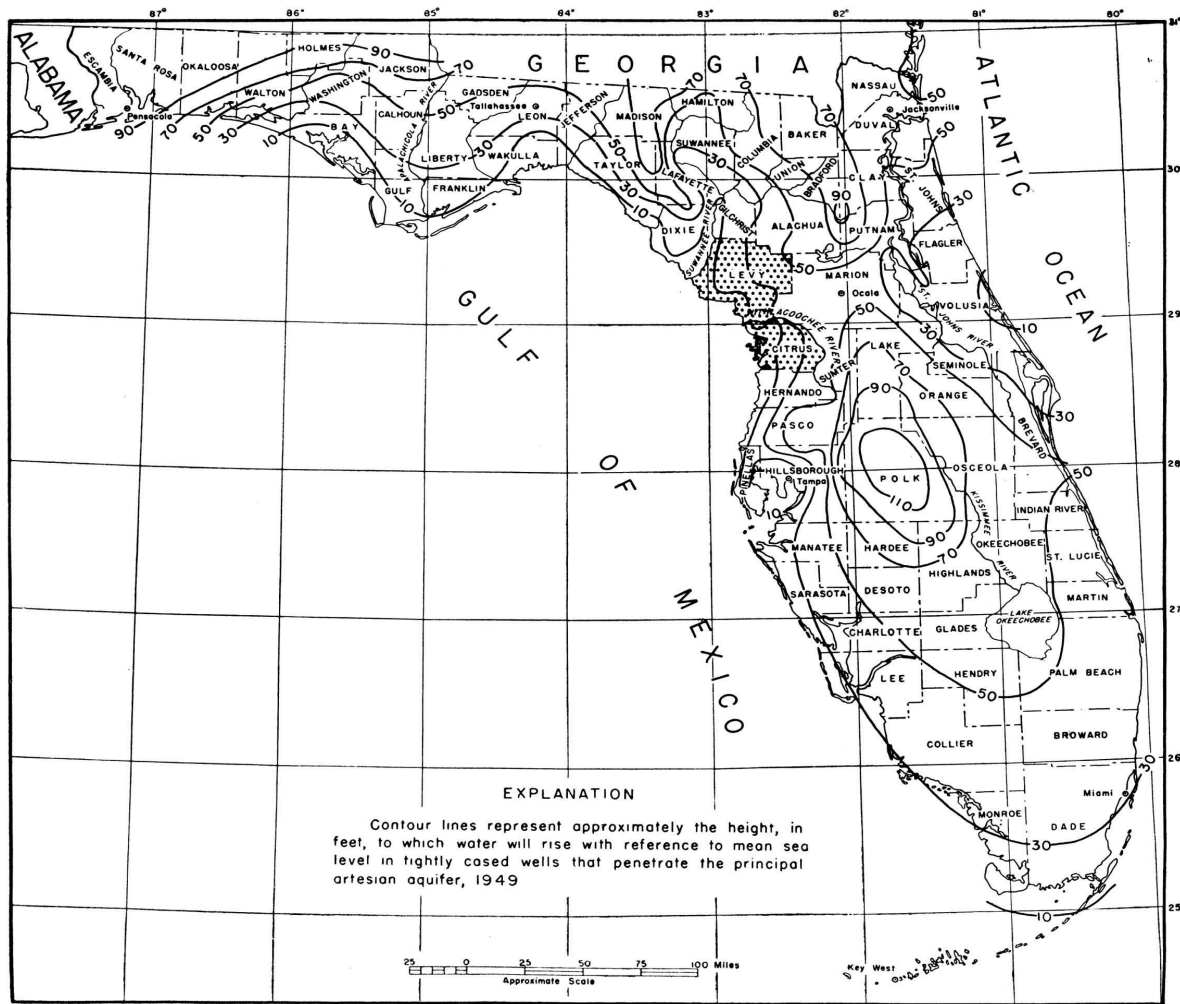
Piezometric Surface of Florida, 1951
