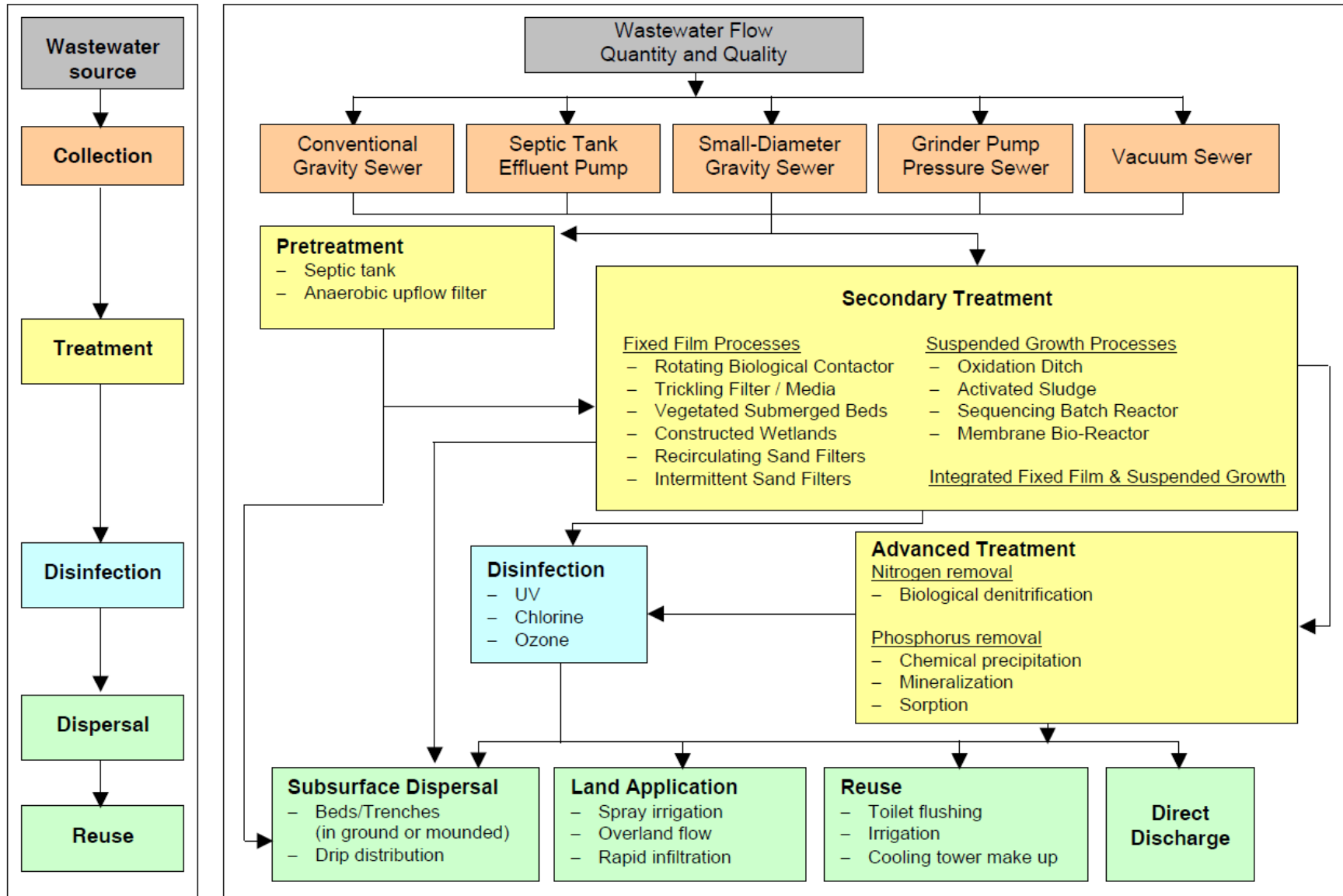
Figure 1-2. Universe of Cluster Collection, Treatment and Disposal Options
