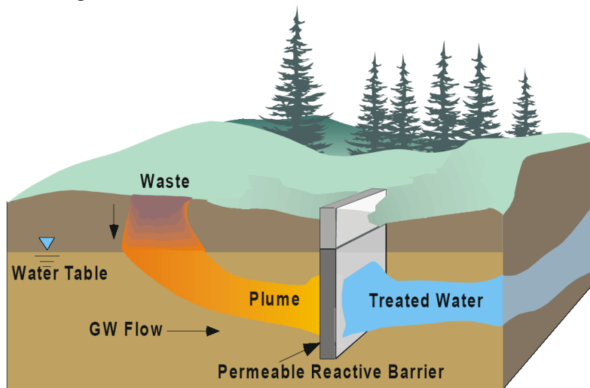
Figure 2-1. EPA Schematic of Groundwater Barrier
