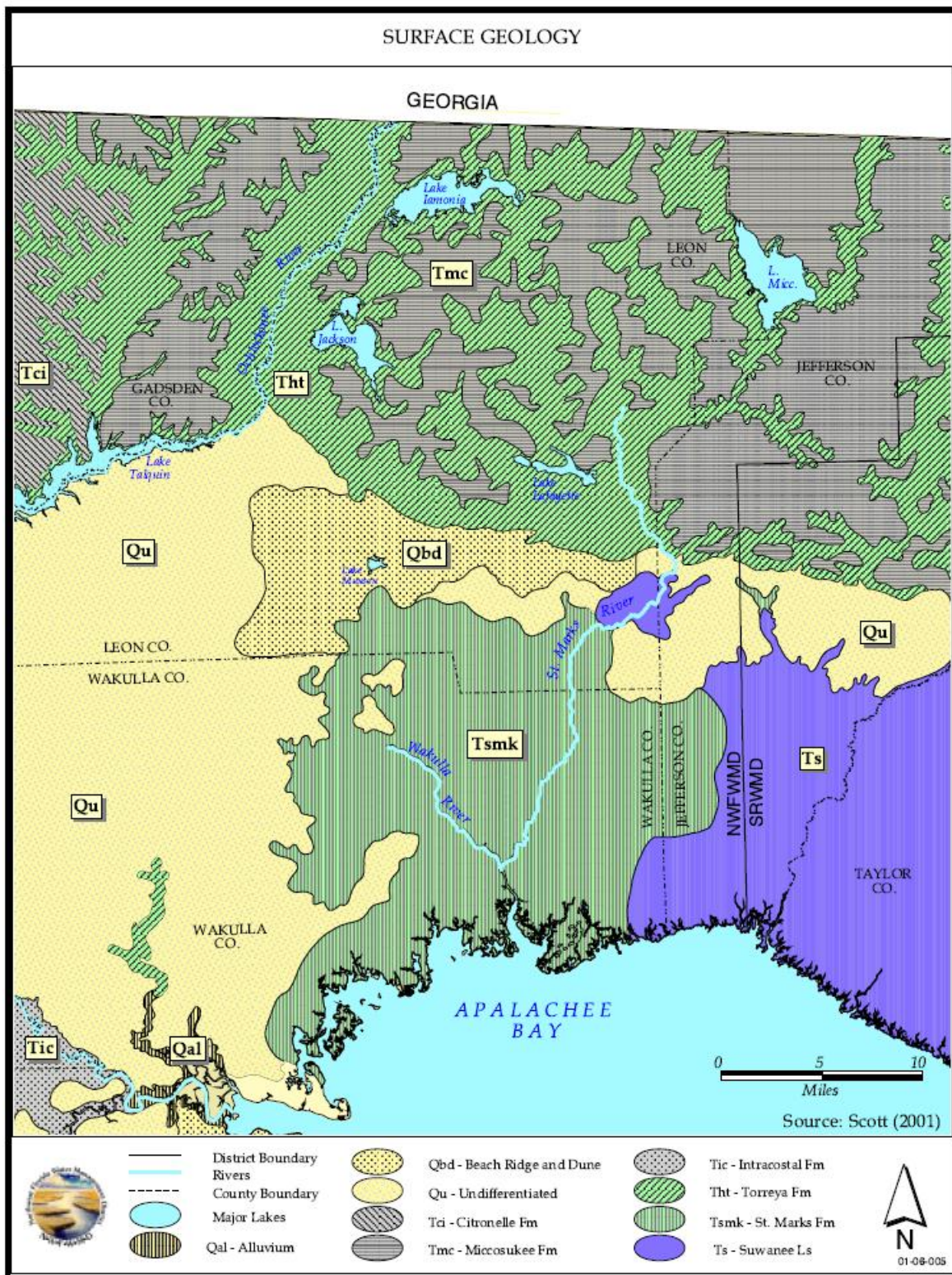
Figure 2-7. Surficial Geology
