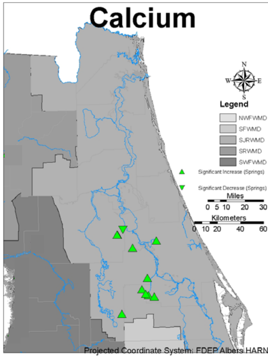
Figure L49. Calcium trends in SJRWMD Springs.
