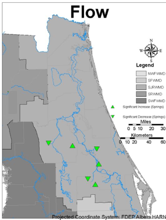
Figure L51. Flow trends in SJRWMD springs.
