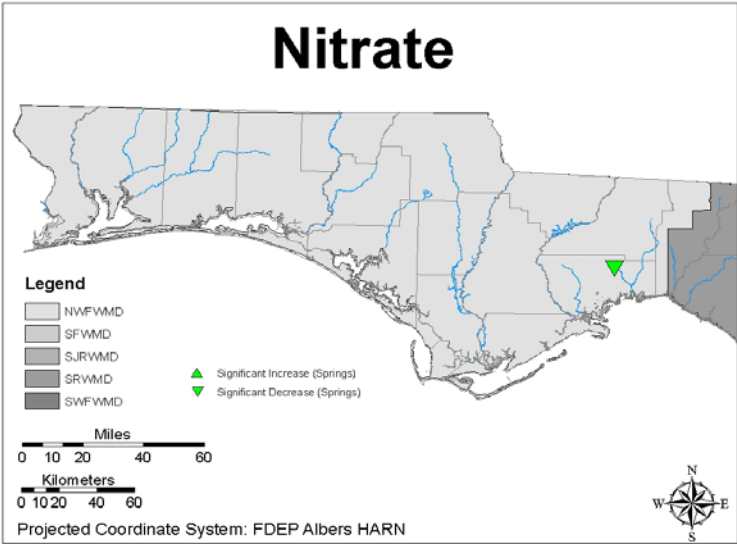
Figure L2. Nitrate trend in NFWFMD spring
