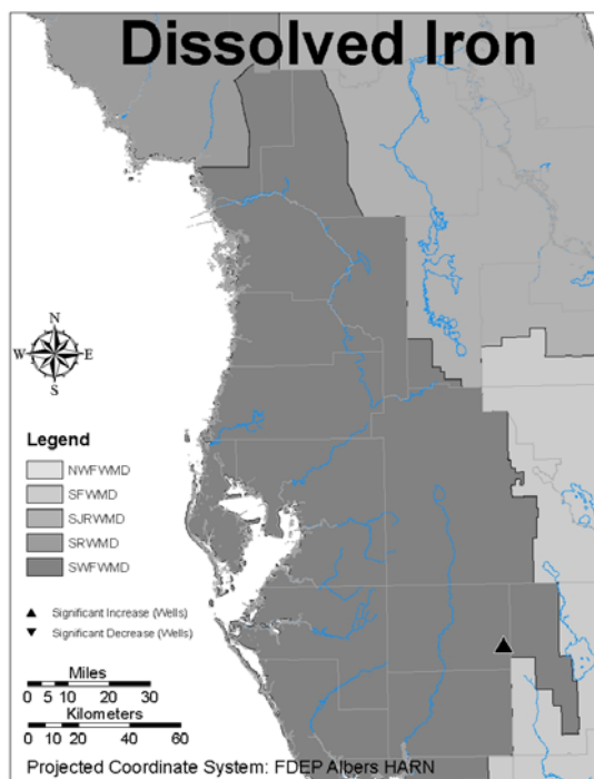
Figure L95. Dissolved iron trends in SWFWMD wells.
