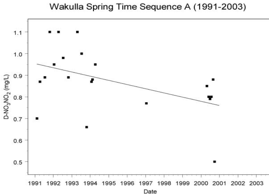
Figure 10. Example of sporadic, unsystematic, and incomplete sampling. Only seven points were collected in the final eight years of this Wakulla Spring study. Sparse, inconsistent sampling after 1994 meant the trend seen here was dependent on relatively few points collected in 2000. Though the trend is statistically valid, this is an excellent illustration of the need for consistent long-term data collection. Ironically, though budget issues are often responsible for gaps in sampling, note that missing data greatly reduces the value of points remaining. Note no data were obtained after 2001 even though Sequence A continued through 2003.
