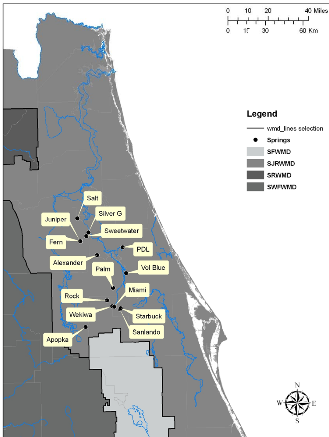
Figure L48. SJRWMD springs.
