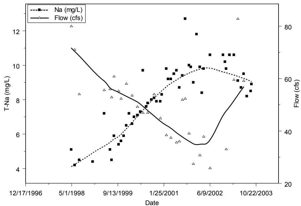
Figure A5. Poe Spring – Sodium versus flow.
