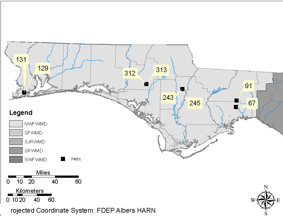
Figure L3. NFWFMD Wells
