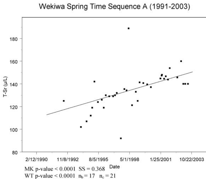
Figure 30. Increasing rock analytes at Wekiwa Spring. Alkalinity (top) and strontium (bottom) increased significantly over Sequence A. Tests ( p < 0.05 ) included MK for trend, WT on sequences B and C, plus an SS calculation. Beginning dates for these springs were not the same.
