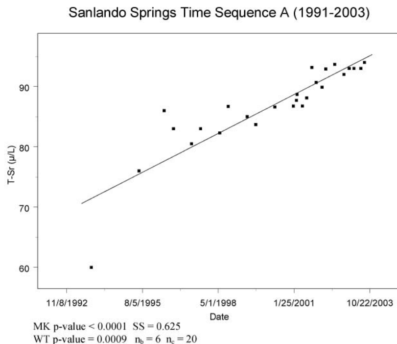
Figure 29. Increasing rock analytes at Sanlando Springs. Alkalinity (top) and strontium (bottom) increased significantly over Sequence A. Tests ( p < 0.05 ) included MK for trend, WT on sequences B and C, plus an SS calculation on rate of change. Beginning and ending sampling dates for these springs were not the same.
