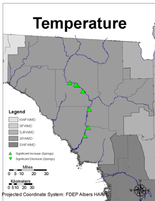
Figure L28. Temperature trends in SRWMD Springs.
