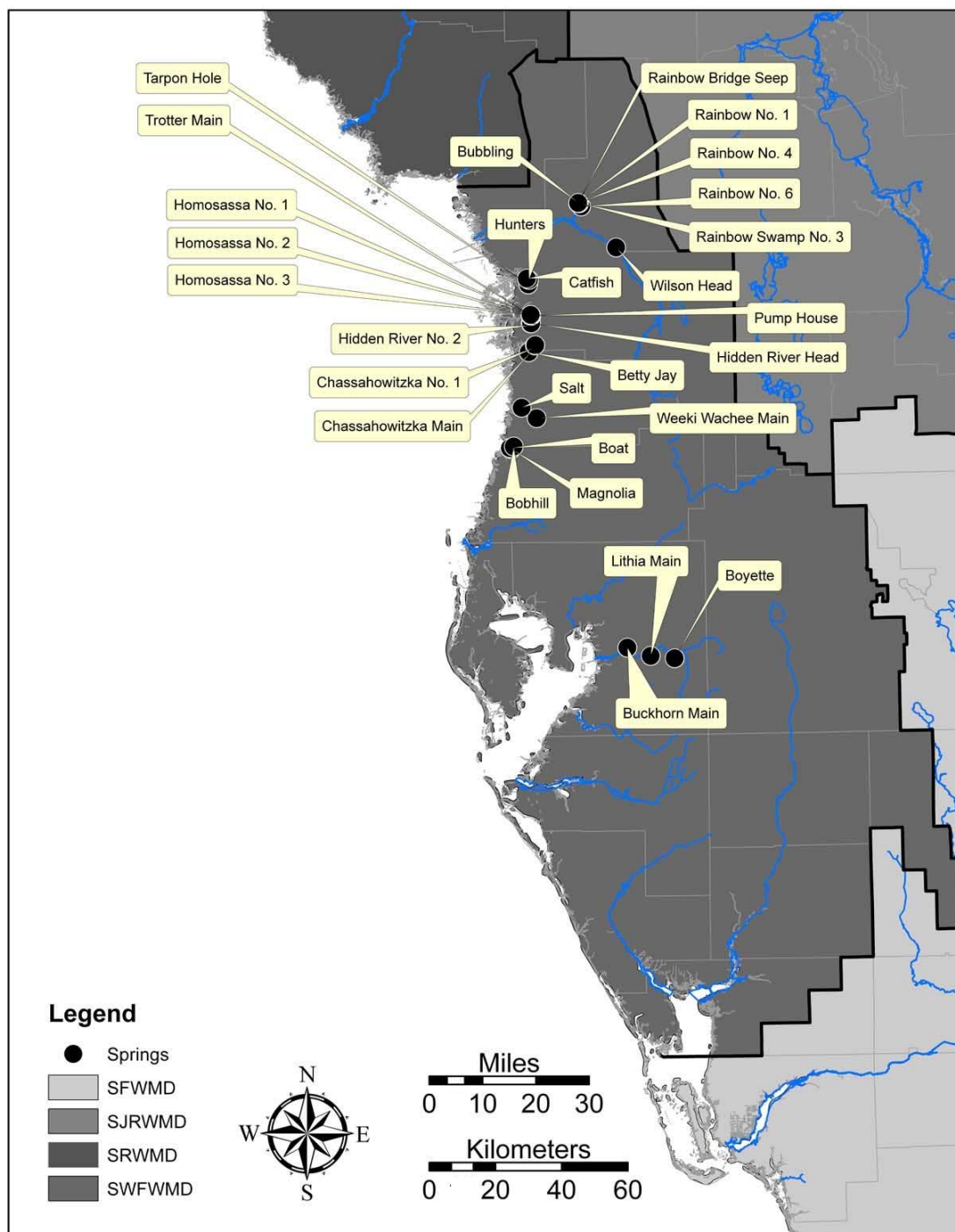
Figure 73. SWFWMD springs.
