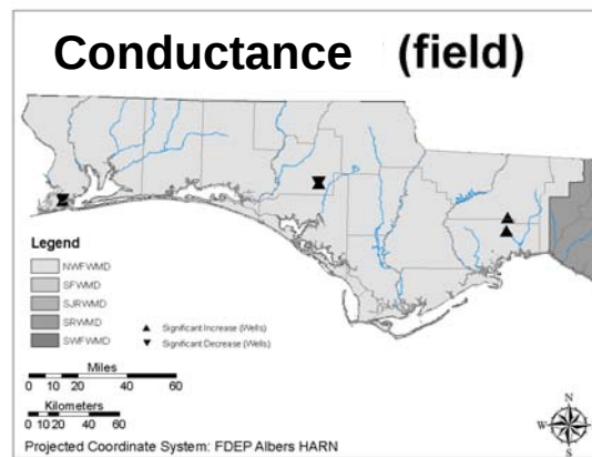
Figure L6. Conductance (field) trends in NFWMD wells.
