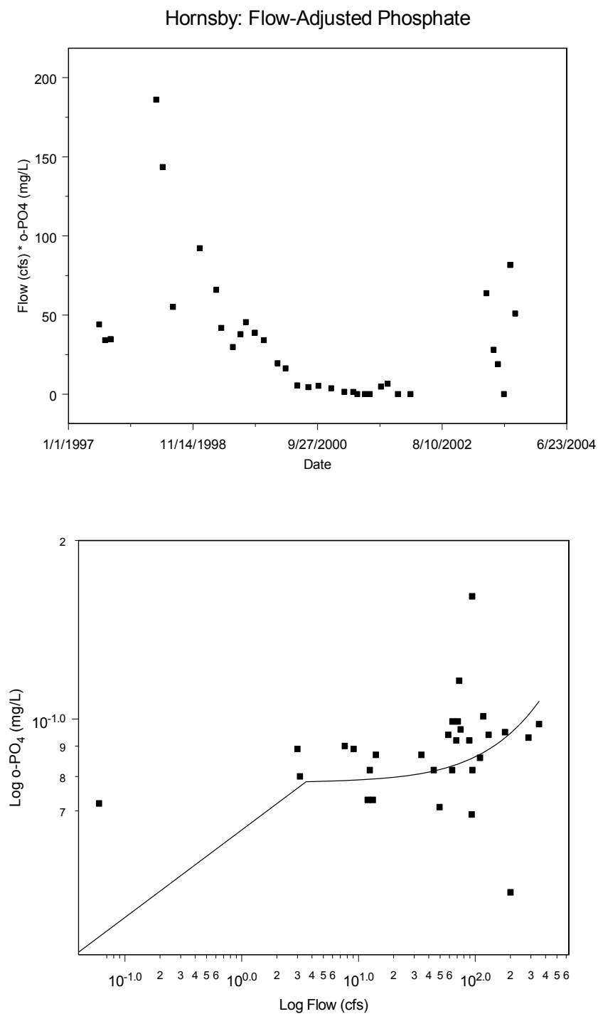
Figure 75. Flow adjustment for phosphate in Hornsby Spring. One of the few examples of a decreasing phosphate trend in the SRWMD. Flow-adjusted phosphate shows a pronounced decline over time with a large increase at the end (top). The log of phosphate as a function of the log of flow (bottom) shows an association. This pattern is the opposite of what is seen with the majority of the SRWMD springs where increasing phosphate trends correspond to a negative relationship with the log of flow.
