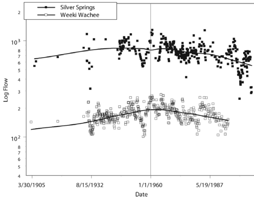
Figure 76. Atlantic Multidecadal Oscillation and Florida spring flow. The Atlantic Multidecadal Oscillation (AMO, top panels) compared to long-term changes in Florida's spring flow (bottom). Top shows North Atlantic sea surface temperature (SST, °C) since 1900. Top lower panel shows effects of the positive AMO on the rainfall and corresponding flow into Lake Okeechobee. Bottom chart is the log of flow against time for two large Florida springs: Silver Springs and Weeki Wachee Springs. The lines (smoothed spring flow) increase until 1960 (marked) and decline thereafter. Flow from the springs align with AMO patterns during past century. (National Oceanic and Atmospheric Administration [2006b]).
