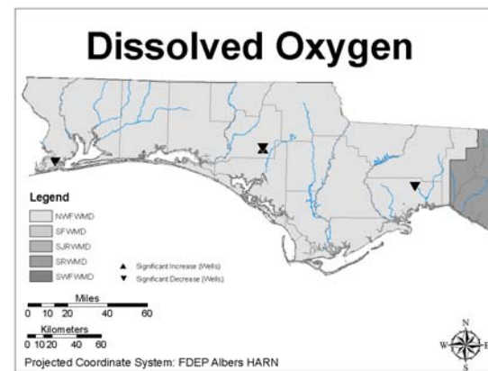
Figure L7. Dissolved oxygen trends in NFWMD wells.
