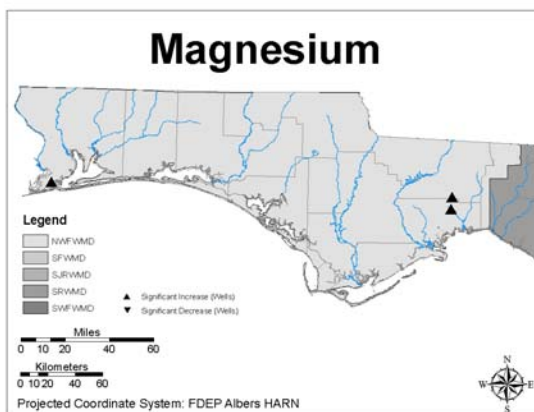
Figure L8. Magnesium trends in NFWMD wells.
