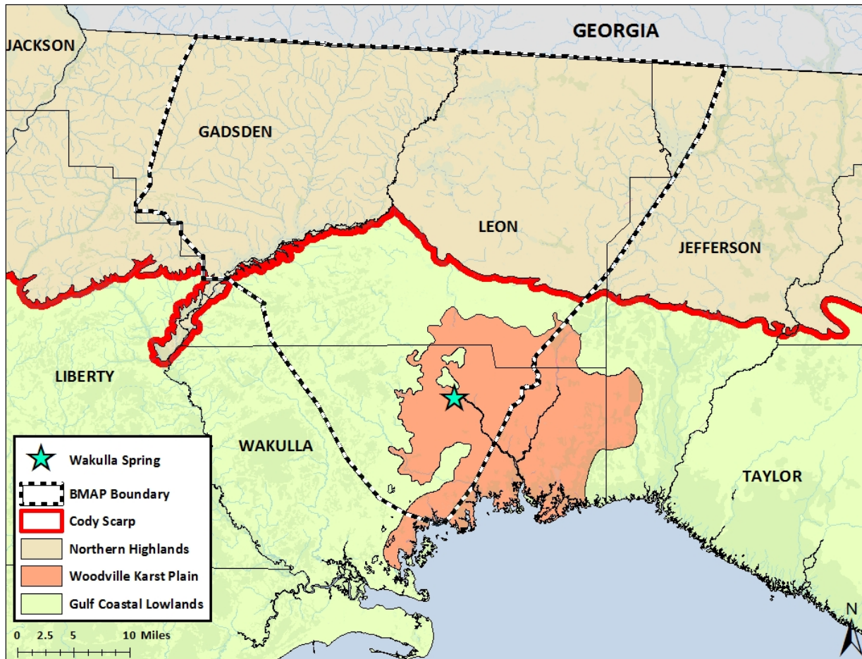
Figure 2: Physiographic regions in and around the Wakulla Spring and River BMAP area
