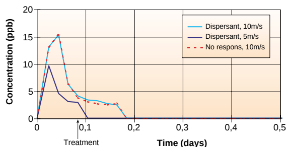
Calculated concentration profile of BTEX-components below an oil spill, at 5 and 10 m/s wind, respectively, and where the dispersant has been added after 2 hours in one of the scenarios.
