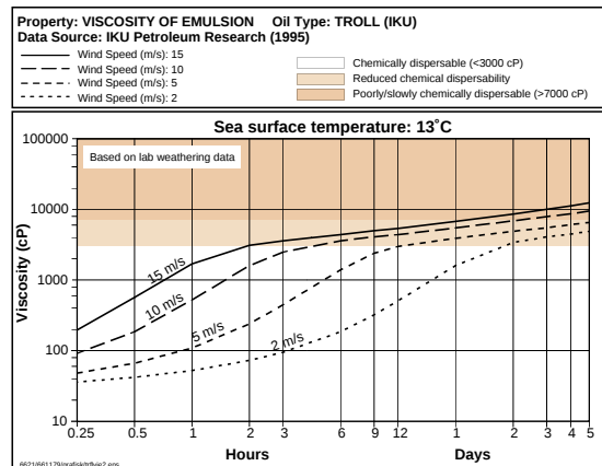
Caculation of "time-window" for effective use of dispersants on Troll Crude (North Sea) under various wind/sea-state conditions
