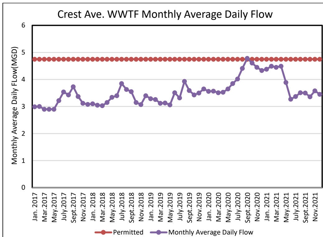
Figure 2-1. Monthly Average Daily Flow
