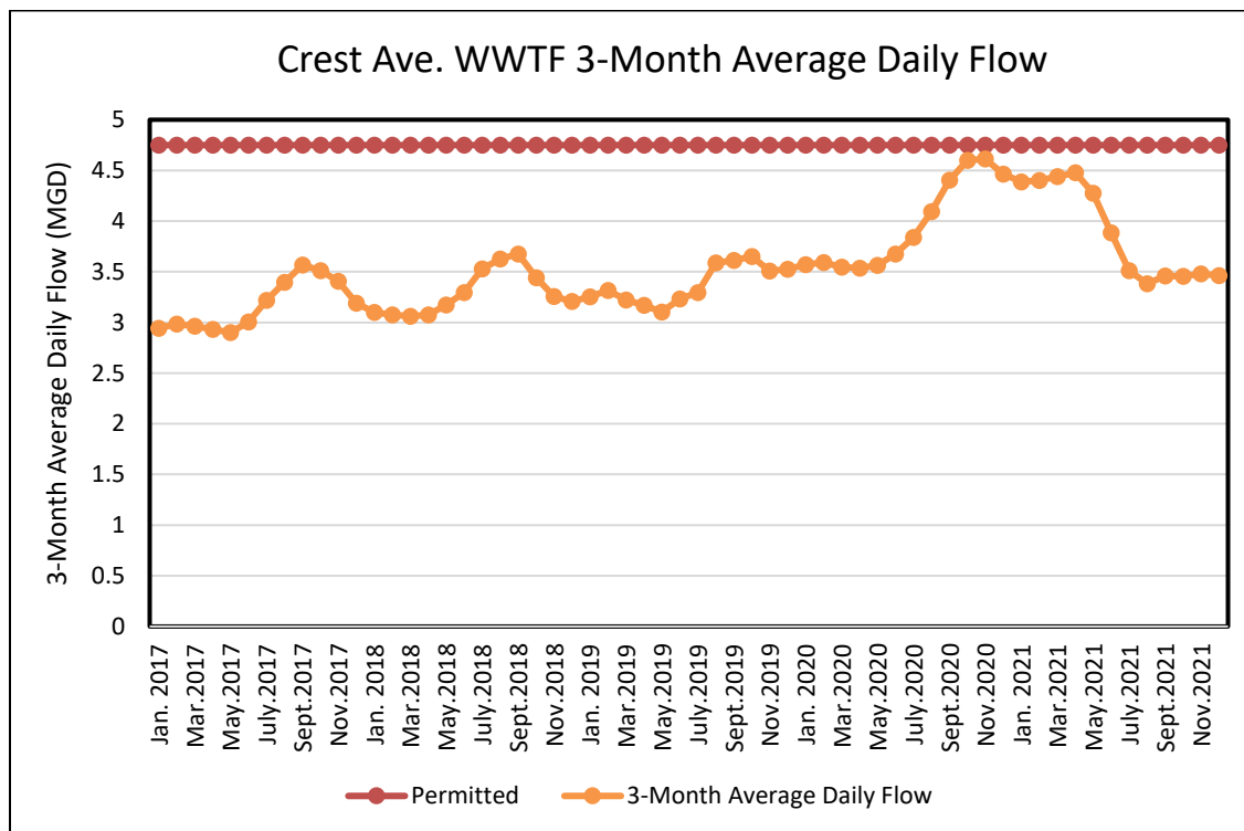
Figure 2-2. Three-Month Average Daily Flow for 2017–2021
