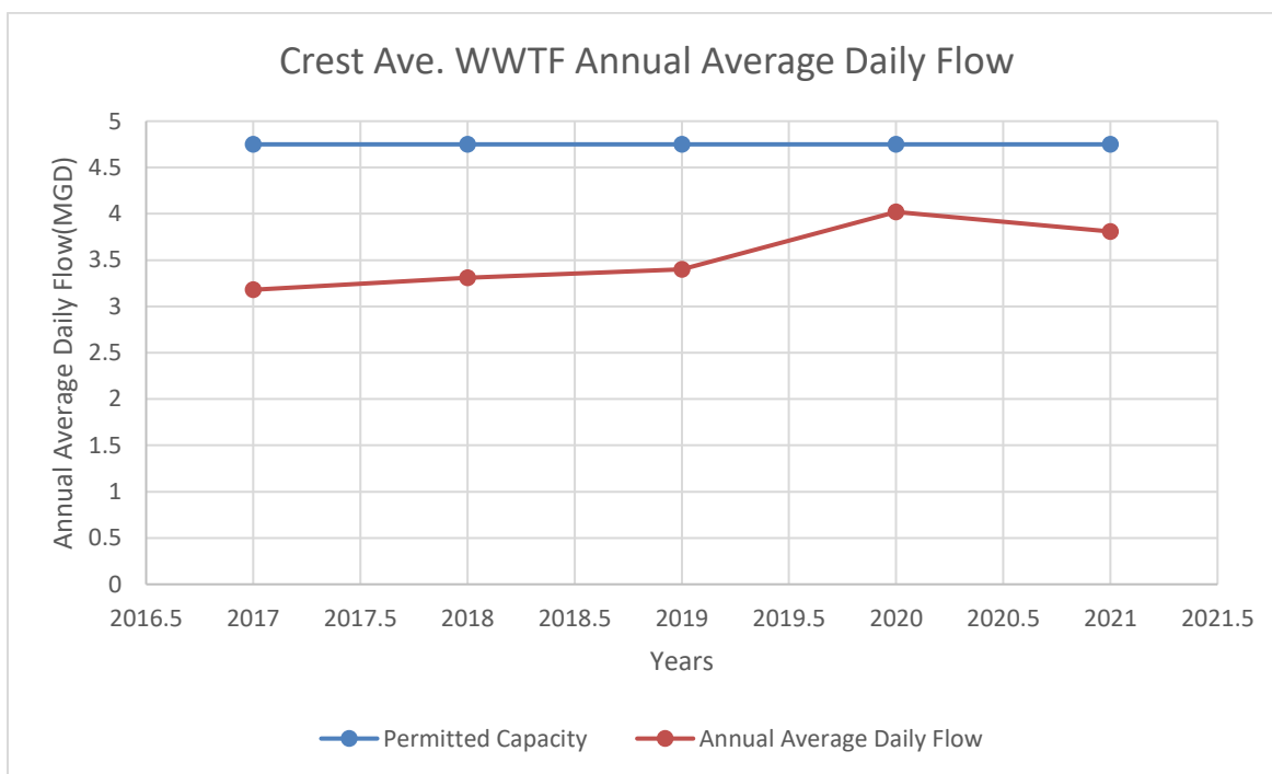
Figure 2-3. Annual Average Daily Flow for 2017–2021
