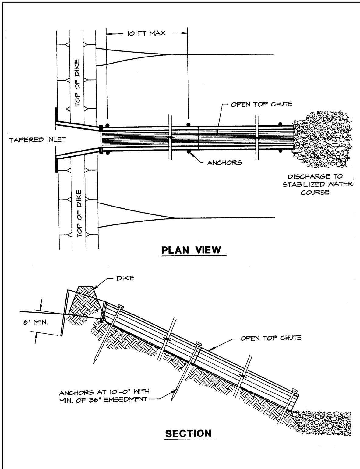
Figure 4.4g. Overside Drain
