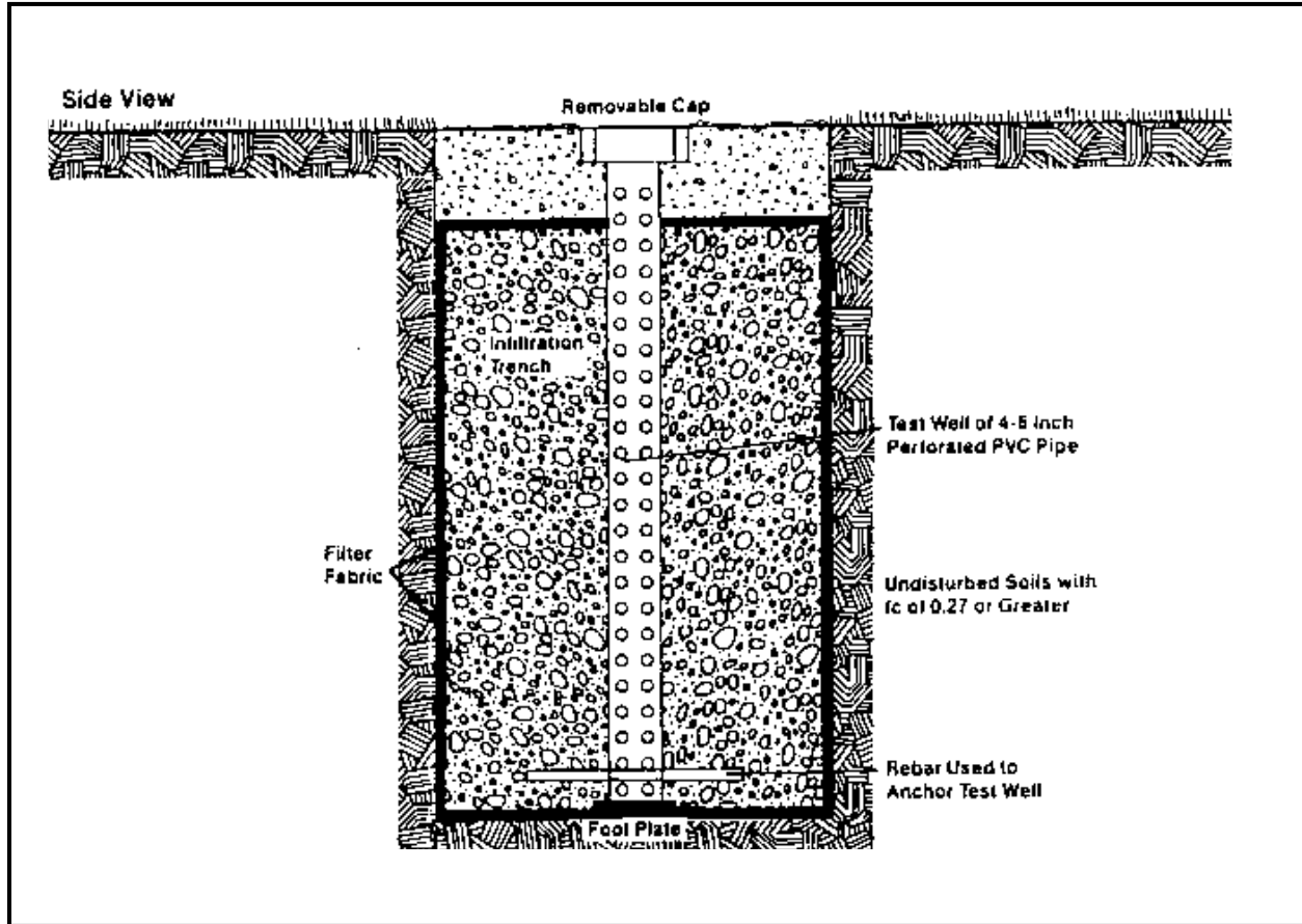
Figure 6.4d. Detailed Schematic of a Typical Observation Well
