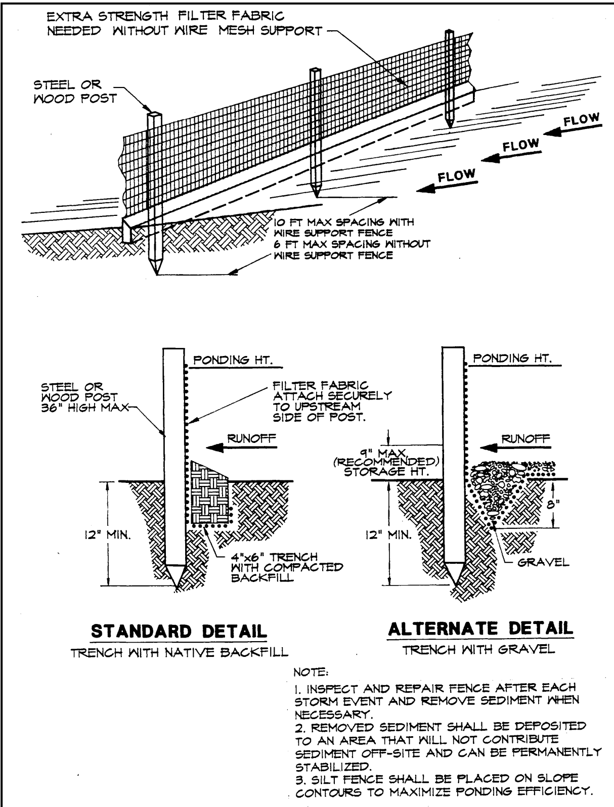
Figure 4.4a. Silt Fence
