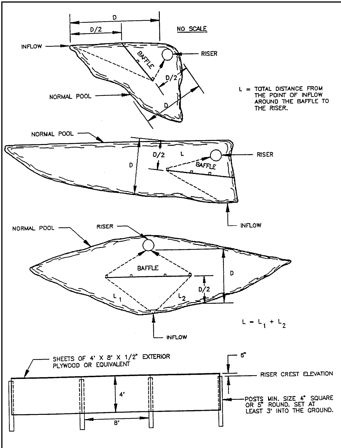
Figure 4.7b. Sample Plan View of Baffle Locations in Sediment Basins
