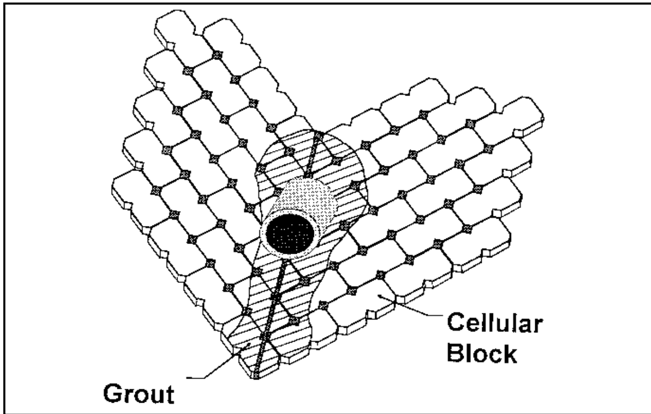
Figure 6.17c. Grout Illustration
