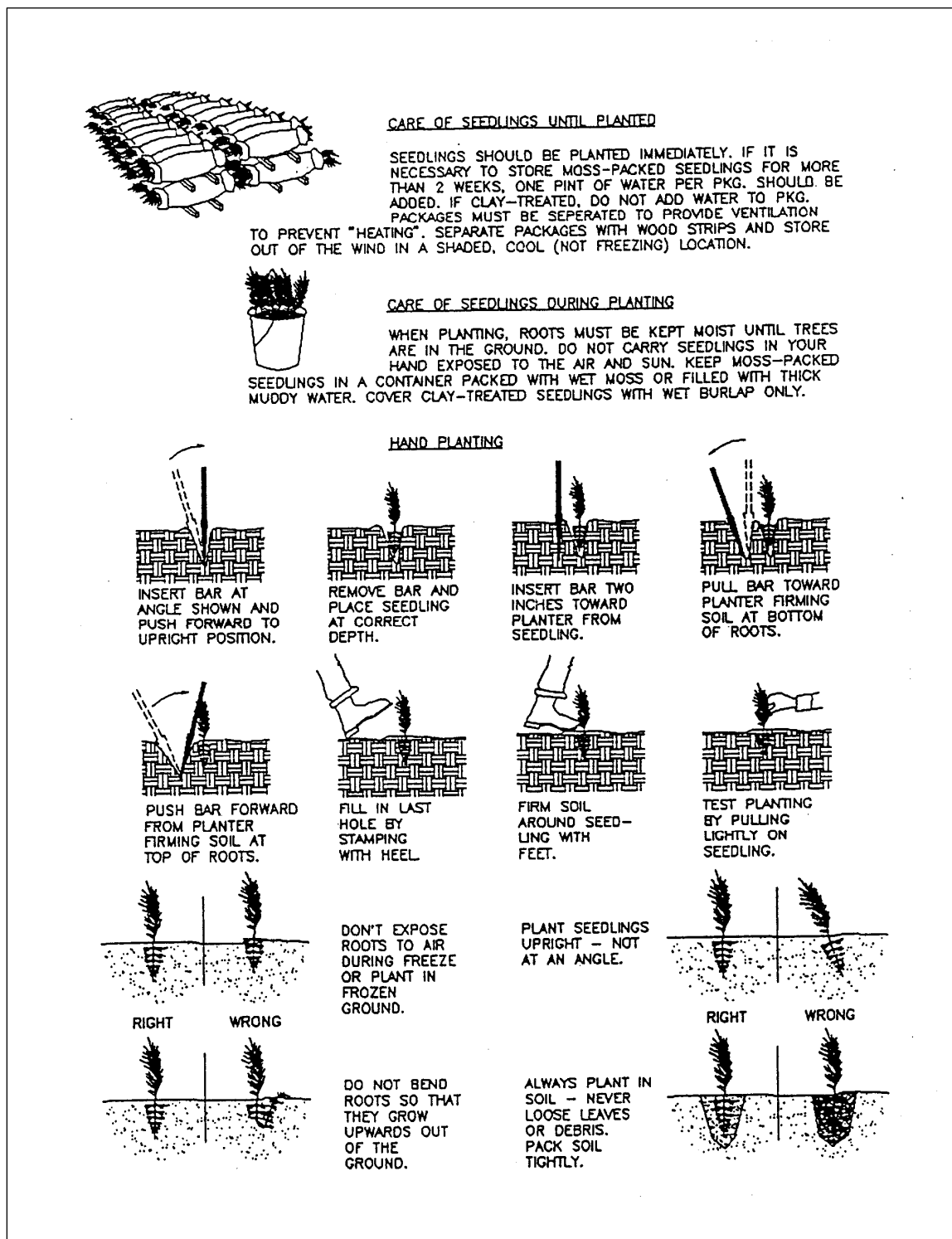
Figure 7.8b. Planting Bare Root Seedlings
