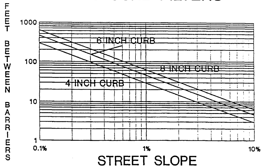
Figure 4.5I. Gravel Bag Curb Sediment Filters
