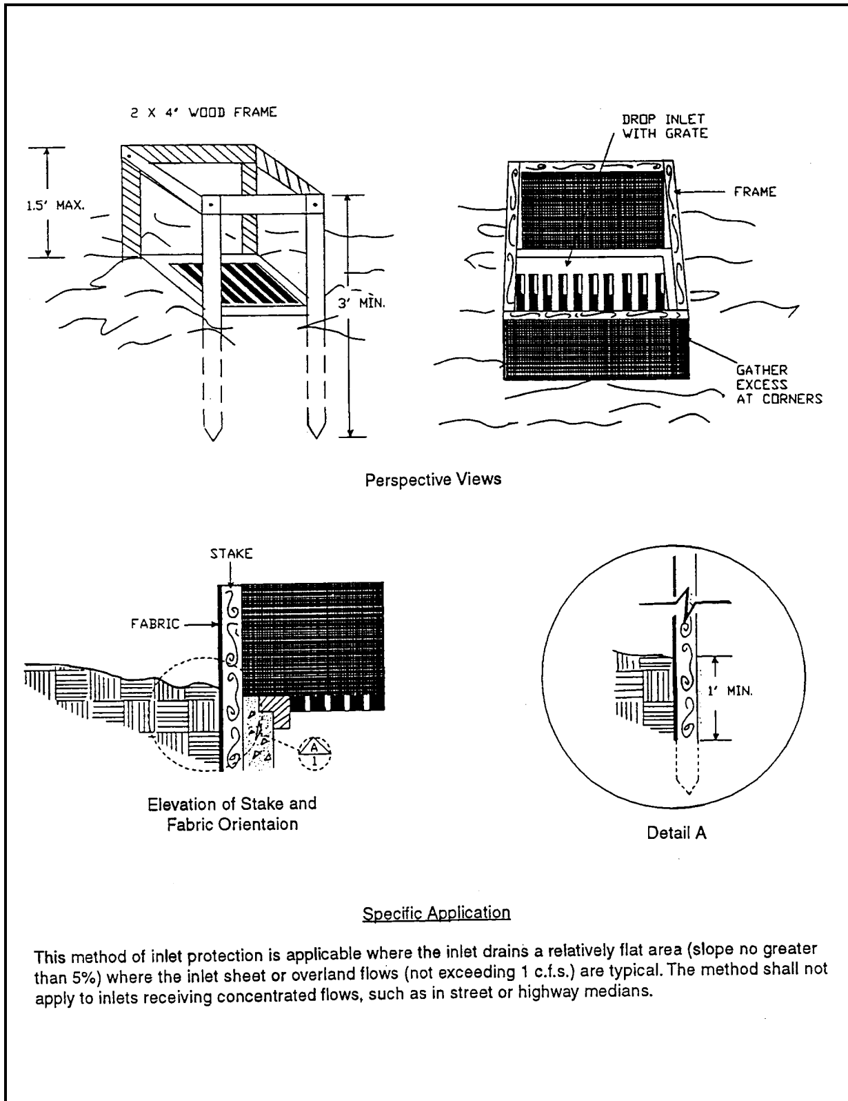
Figure 4.5b. Filter Fabric Drop Inlet Sediment Filter
