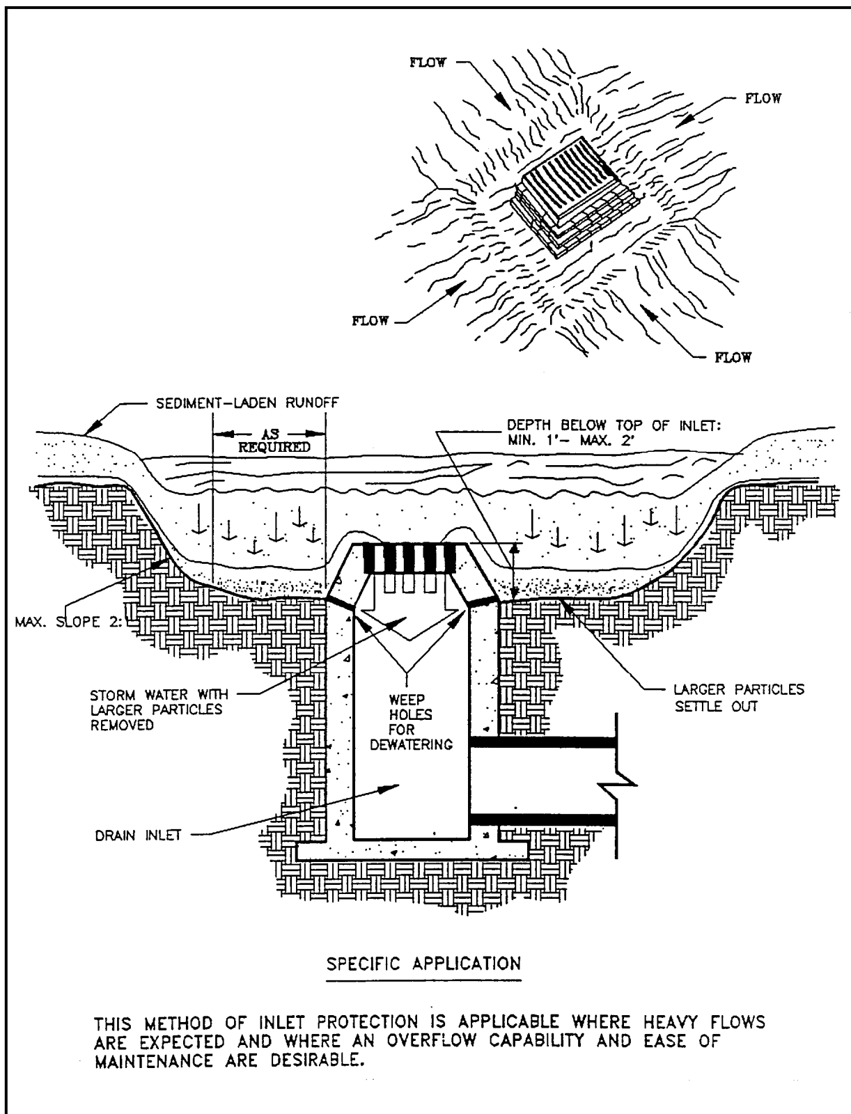
Figure 4.6e. Excavated Drop Inlet Sediment Trap
