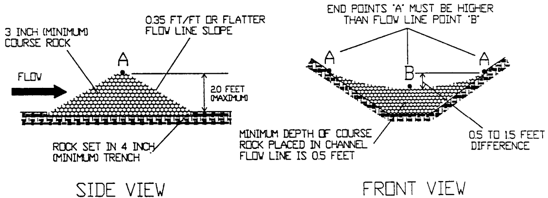
RECOMMENDED ROCK SIZE & FLOW DEPTHS
