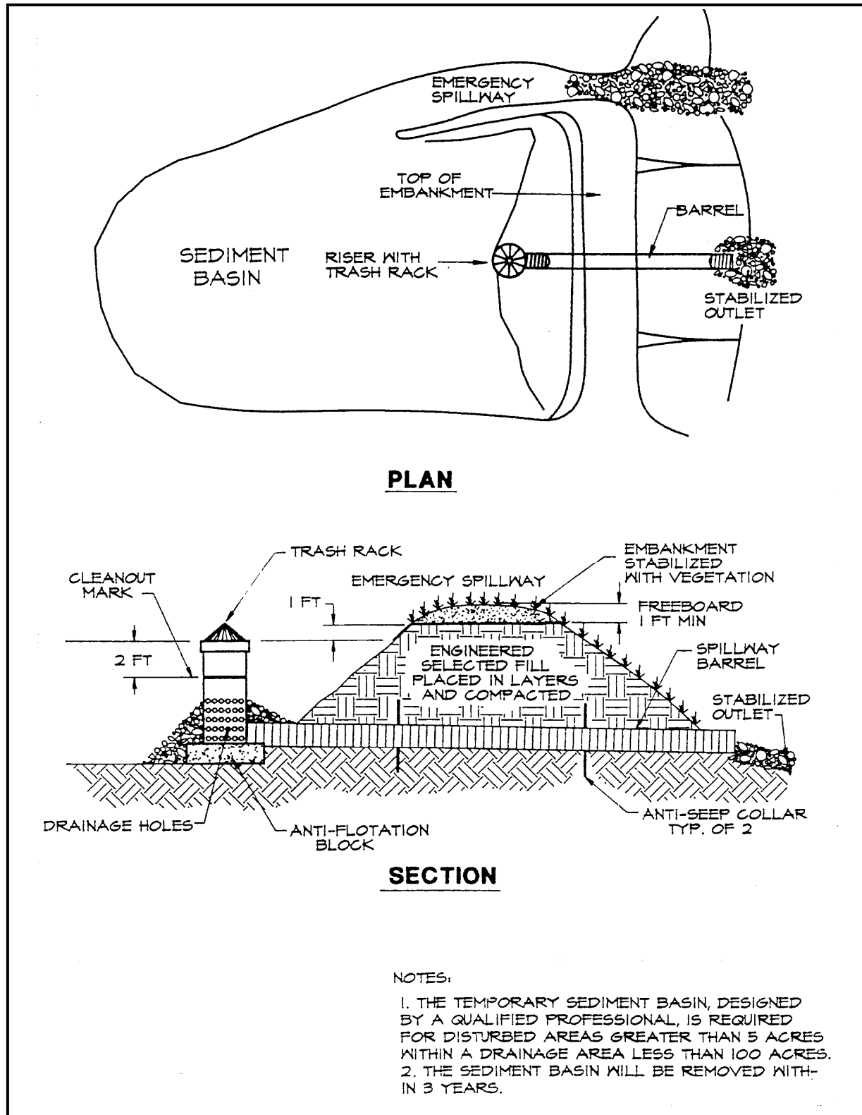
Figure 4.7h. Sediment Basin
