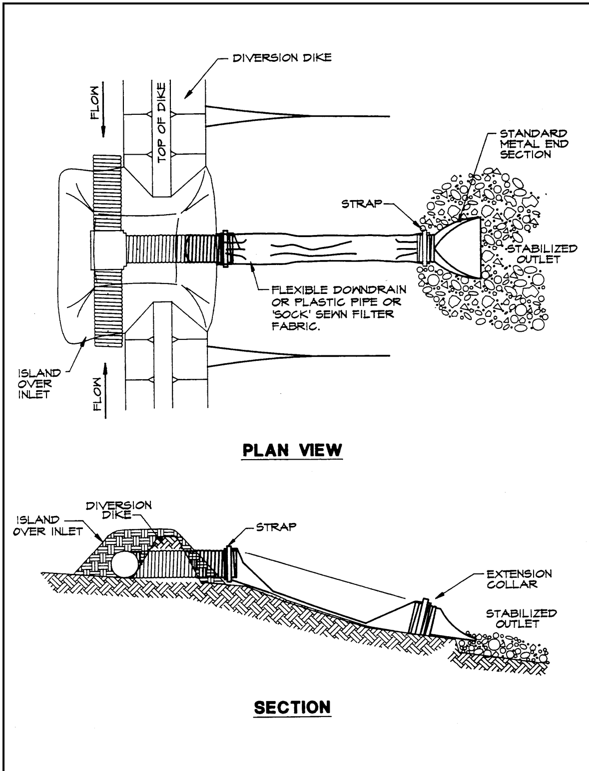
Figure 4.4k. Slope Drain
