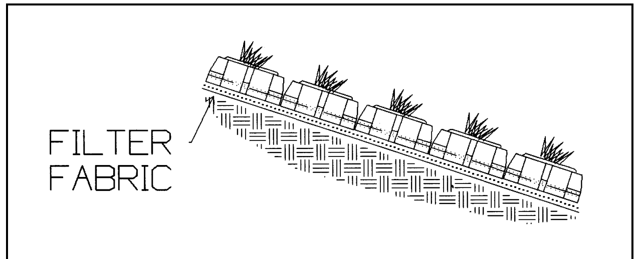
Figure 6.17d. Revegetation
