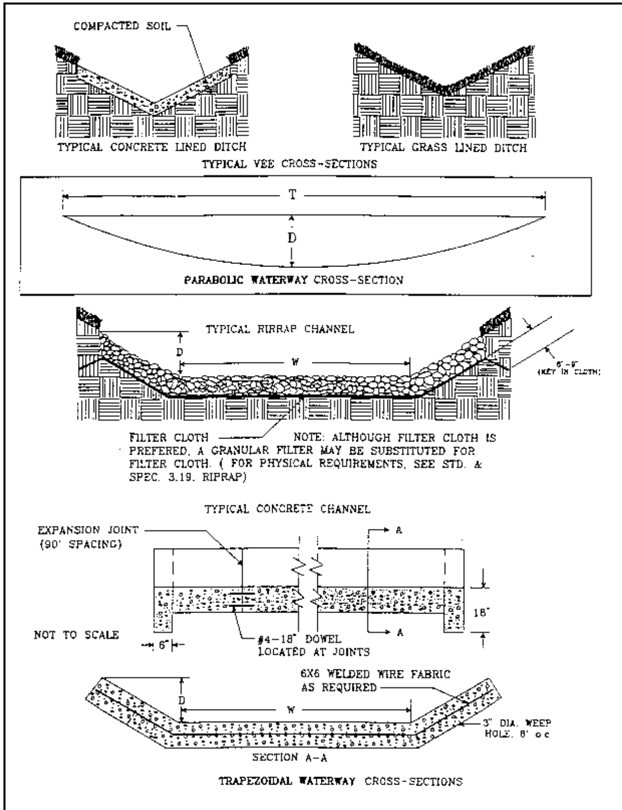
Figure 6.10a. Typical Waterway Cross-Sections
