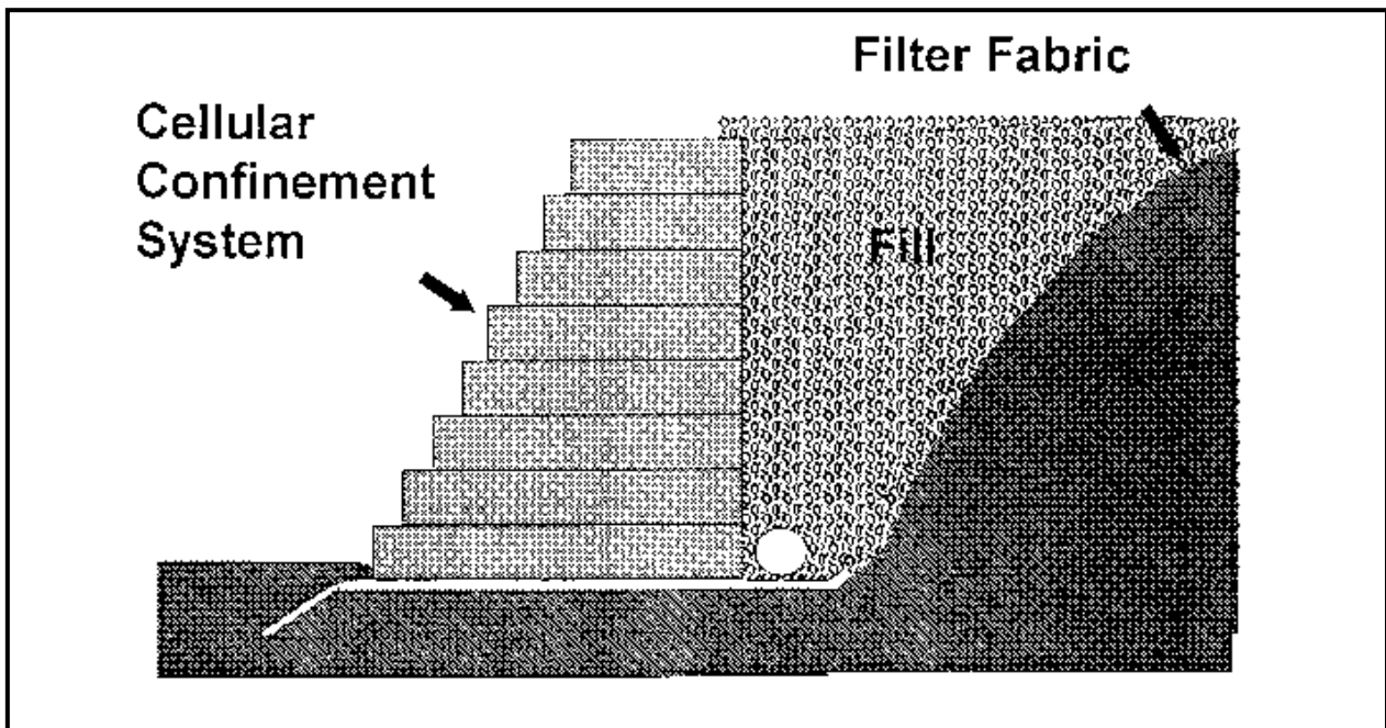
Figure 6.16c. Gravity Retaining Wall Source: NRCS
