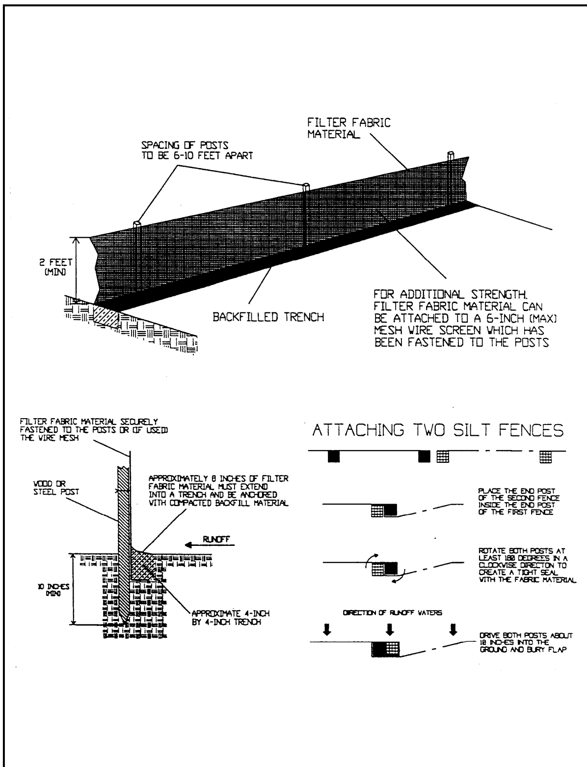
Figure 4.4b. Installing a Filter Fabric Silt Fence
