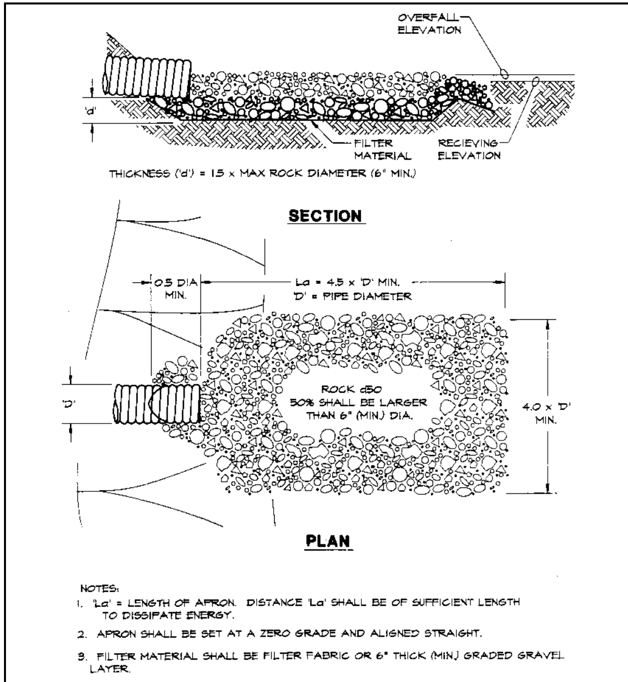
Figure 6.14b. Energy Dissipator
