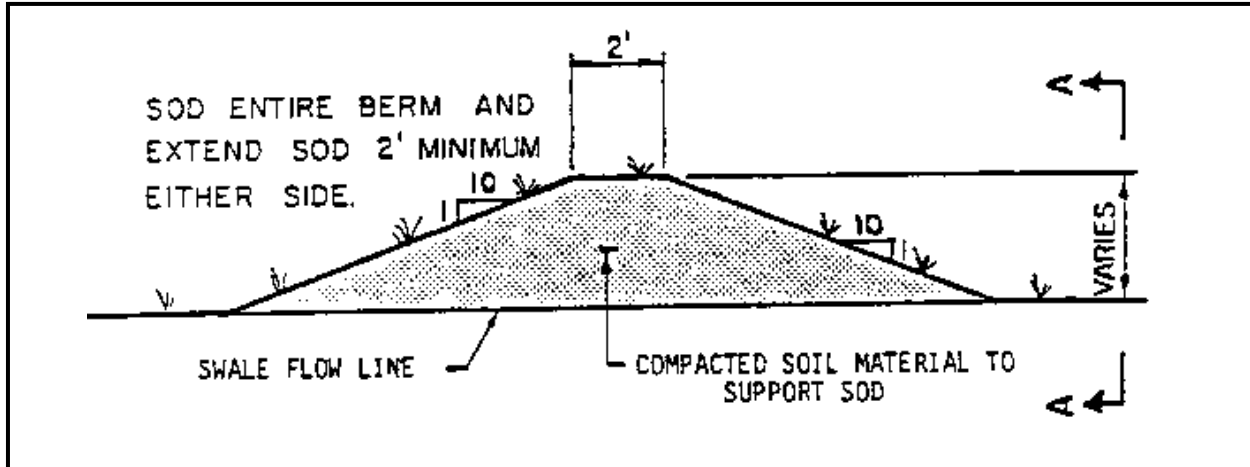
Figure 6.9a. Typical Swale Block Cross-Section
