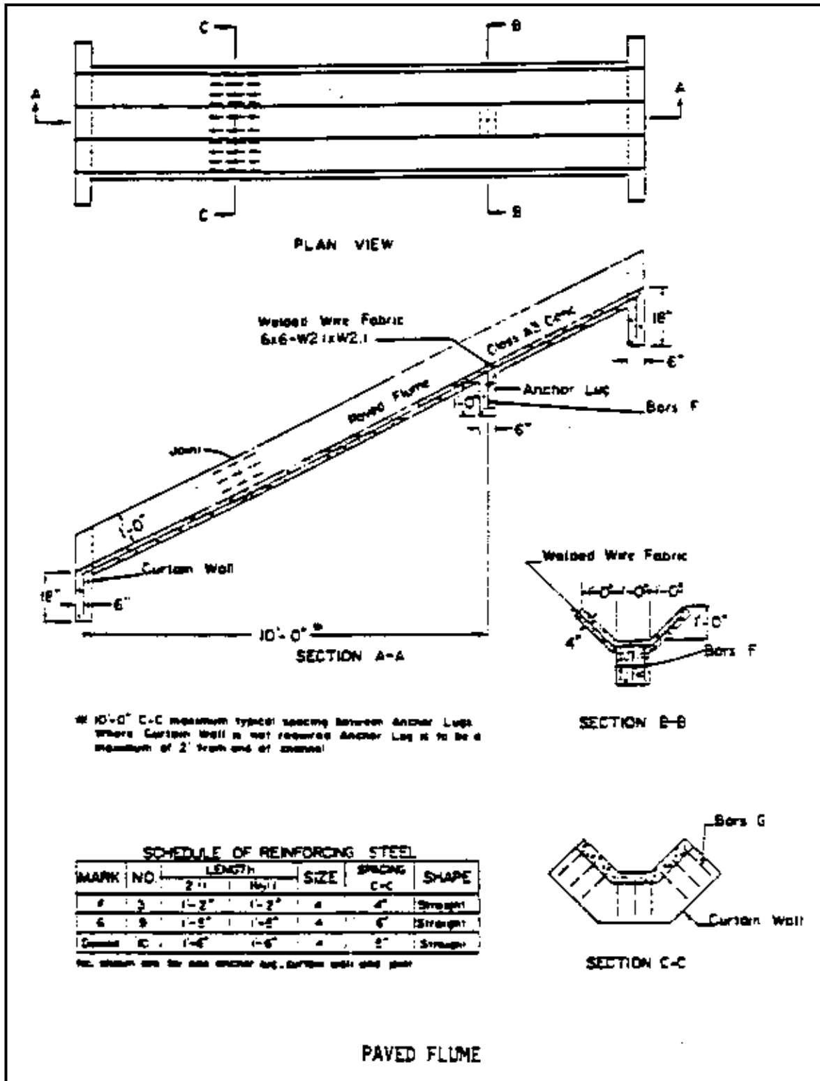
Figure 6.11. Paved Flume
