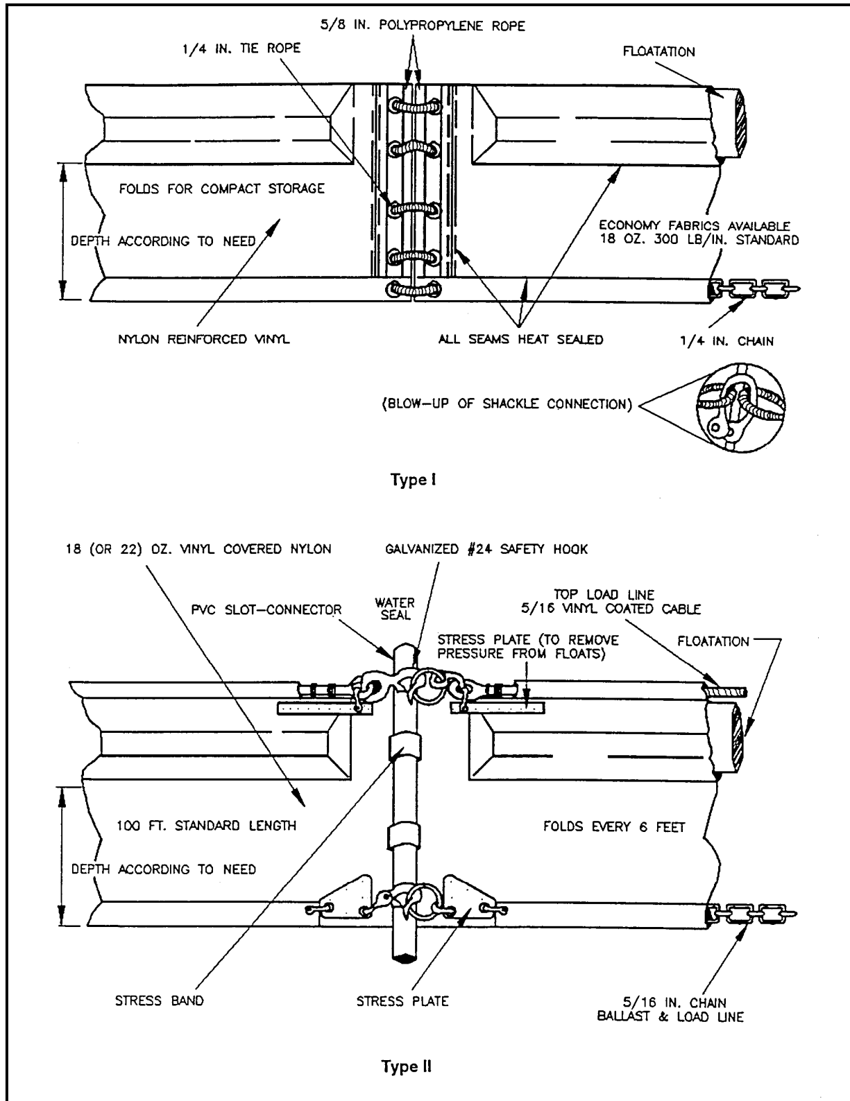
Figure 4.4I. Type I and II Floating Turbidity Barriers
