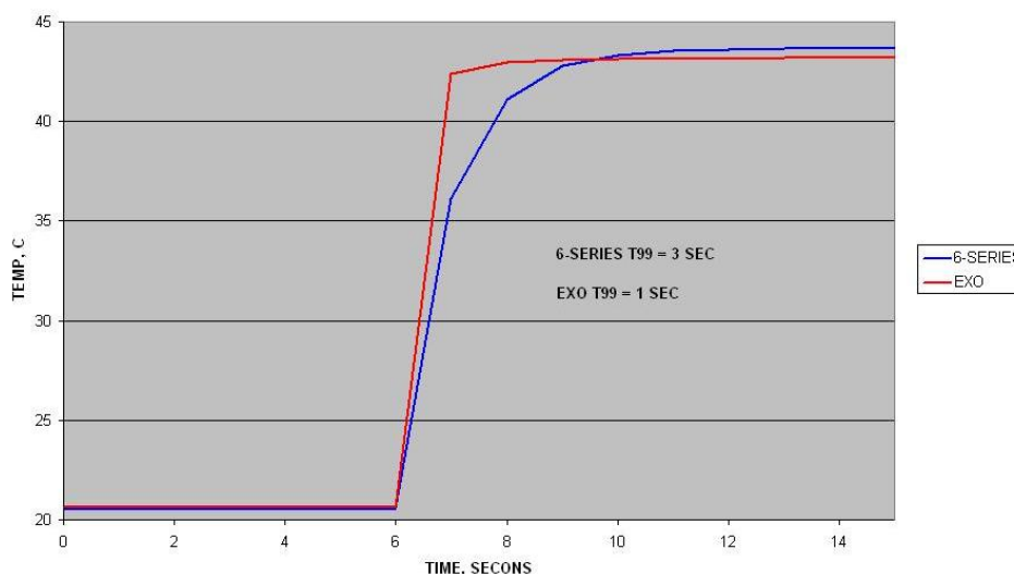
Figure 1: Comparison of response time between EXO and 6-Series temperature sensors. Transfer from ambient temperature water to hot water with rapid stirring.
