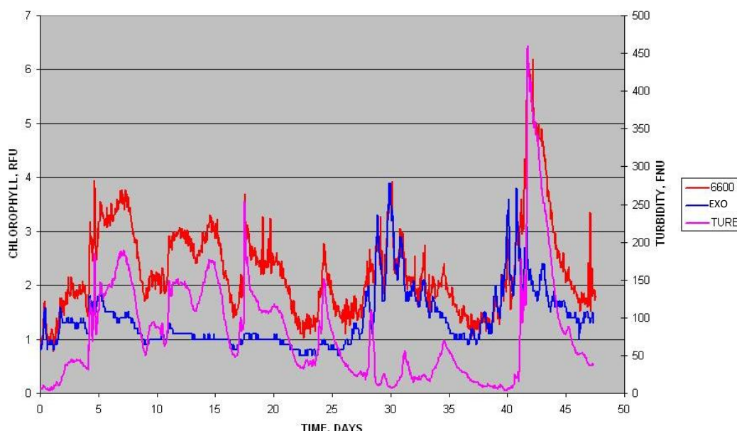
Figure 6: Comparison of chlorophyll sensors of EXO and 6-Series in Miami River, OH over 48-day deployment. The turbidity data demonstrates EXO's decreased sensitivity to turbidity interference from the 6-Series and other commercially available chlorophyll sensors.
