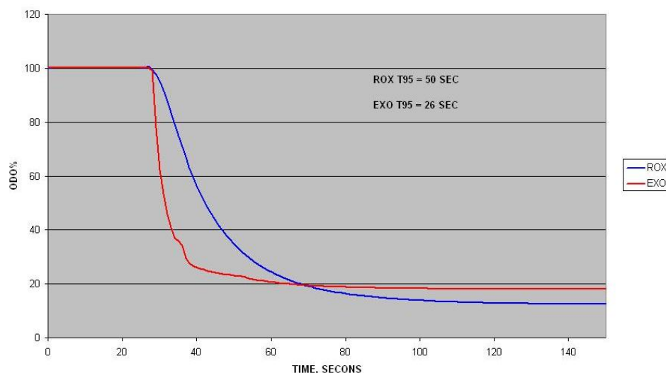
Figure 3: Comparison of response times between the 6-Series ROX DO sensor and the EXO Optical Dissolved Oxygen Sensor. Transfer from air-saturated water to deaerated water with rapid stirring.
