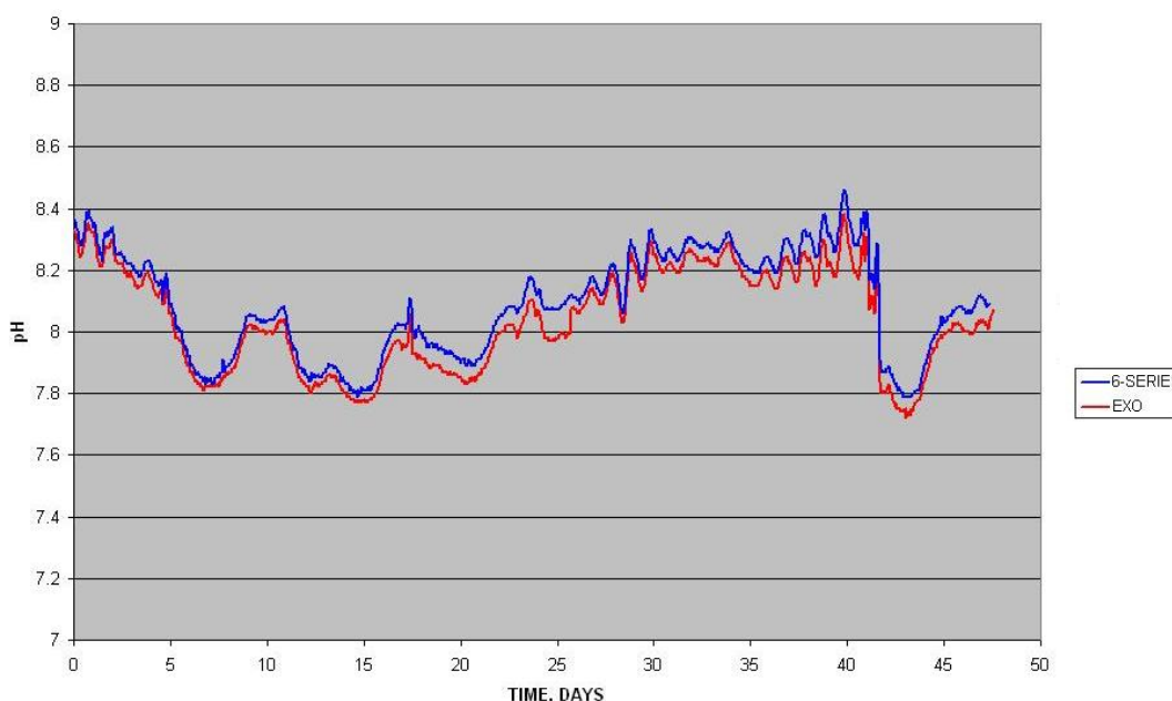
Figure 4: Comparison of pH for EXO and 6-Series pH sensors over 48-day deployment in Miami River, OH.
