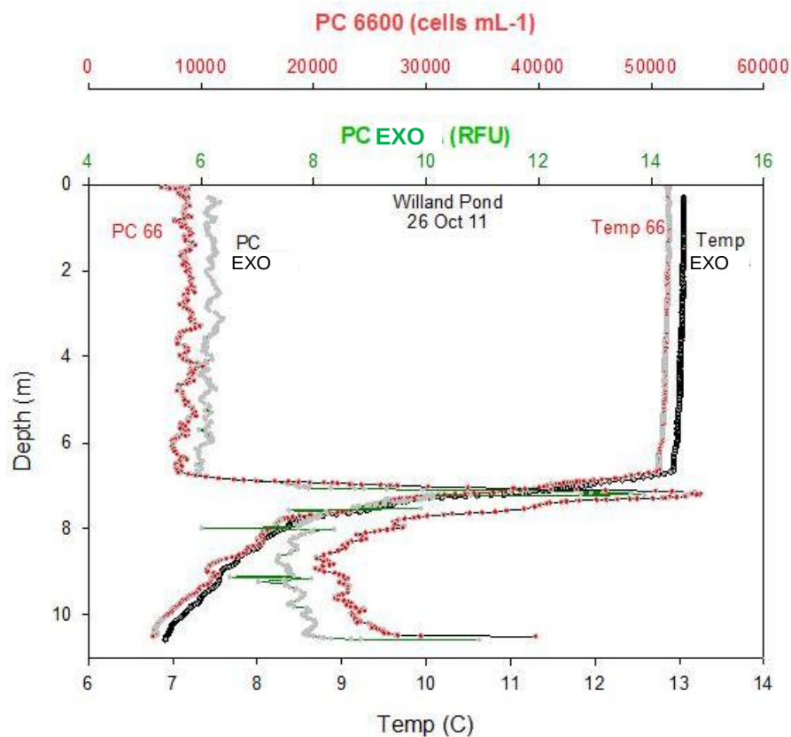
Figure 7: Comparison of blue-green algae (PC) sensors of EXO and 6-Series in vertical profile in Willand Pond, NH. Data shows faster response in the detecting sub-surface maxima and lower sensitivity to dissolved organic interference in region of high DOM below 7 m.
