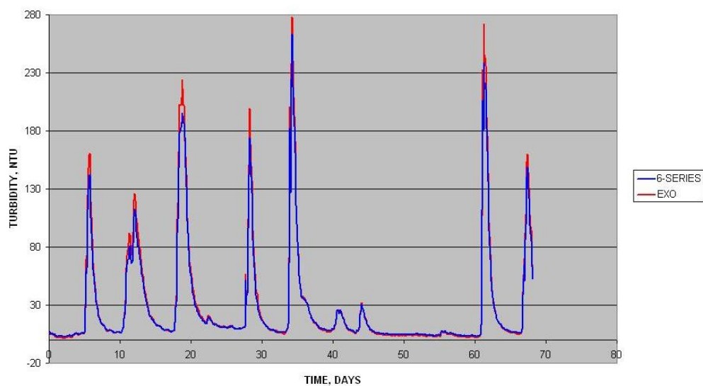
Figure 5: Comparison of turbidity sensors between 6-Series and EXO over a 68-day deployment at Miami River, OH.
