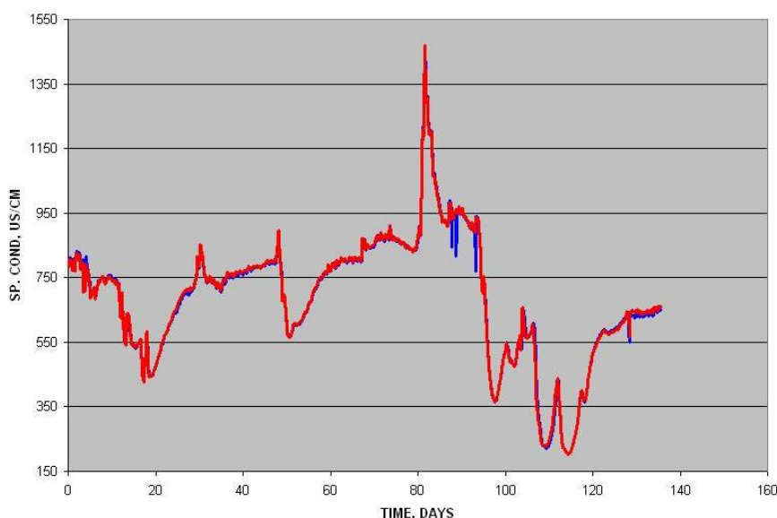
Figure 2: Comparison of specific conductance between EXO and 6-Series in Miami River, OH over 140 days.
