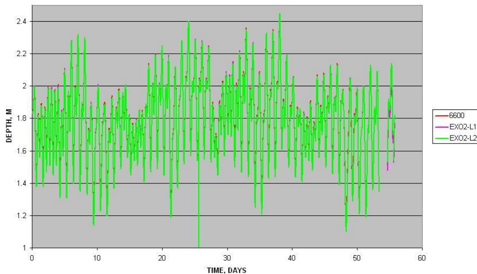
Figure 9: Comparison of depth data between 6-Series and two EXO sondes during a 57-day deployment monitoring tidal fluctuations in Tampa Bay, FL. Data shows excellent agreement between 6-Series and EXO.
