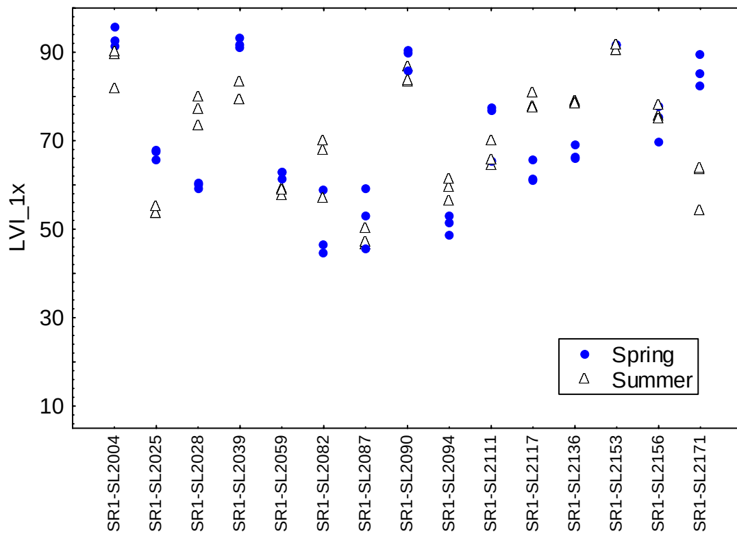
Figure 13. LVI for repeat visits to 15 lakes during the spring (closed circles) and summer (open triangles) of 2004. Each point represents the average LVI from four lake sections. Each lake-visit had three replicate samples of four sections each (4 x 3 = 12 lake sections).
