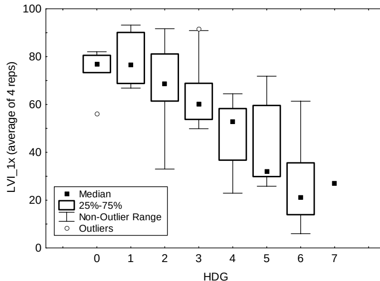
Figure 11. For the validation data set, LVI declined significantly as human disturbance increased (Spearman's r = -0.73 , p < 0.01 , N = 63 ). LVI for each lake was calculated as the average LVI from four lake sections.
