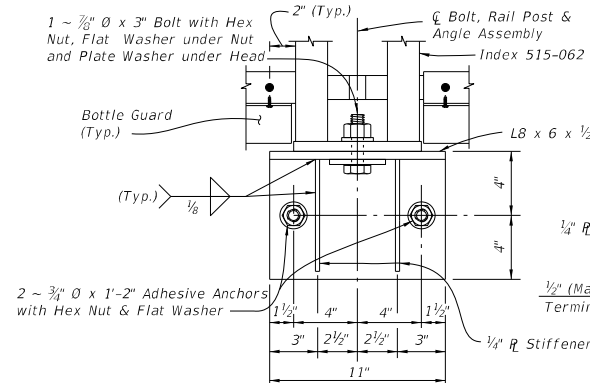
ELEVATION VIEW
