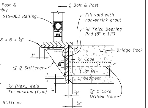
TYPICAL SECTION
