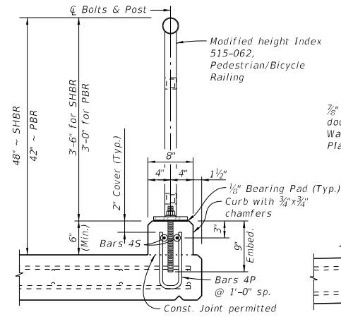
SCHEME 2 - TYPICAL SECTION THROUGH CURB MOUNTED RAILING
