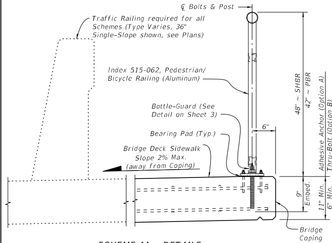
SCHEME 1A - DETAILS (Adhesive Anchor Option)
