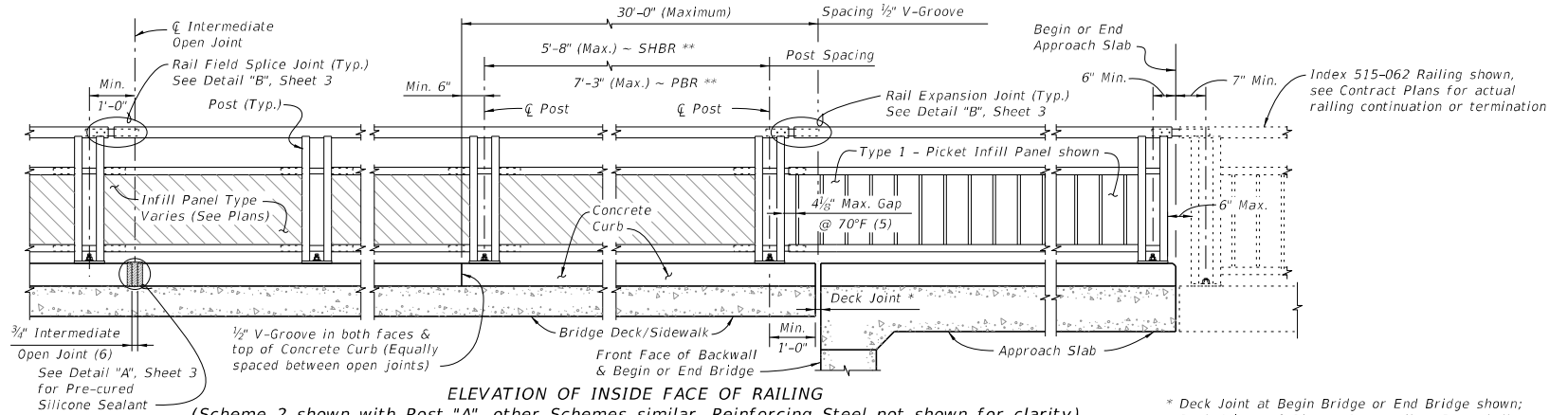
(Scheme 2 shown with Post "A", other Schemes similar, Reinforcing Steel not shown for clarity)
