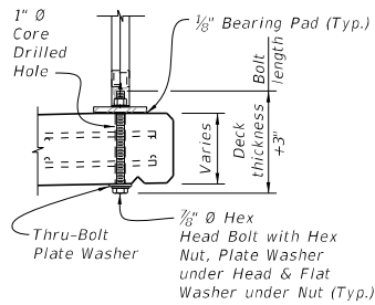
SCHEME 1B - DETAILS (Thru-Bolt Option)
