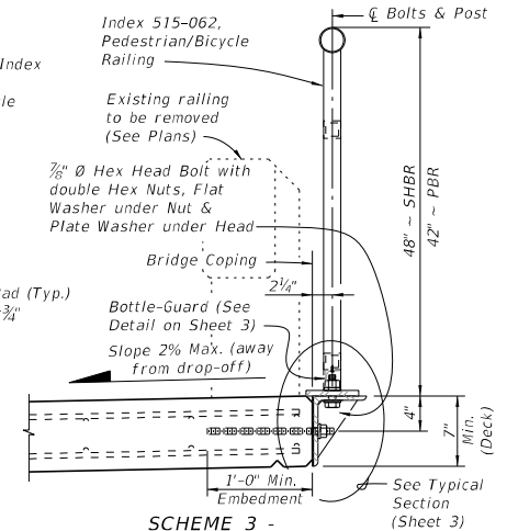
SCHEME 3 - TYPICAL SECTION THROUGH SIDE MOUNTED RAILING (RETROFIT)
