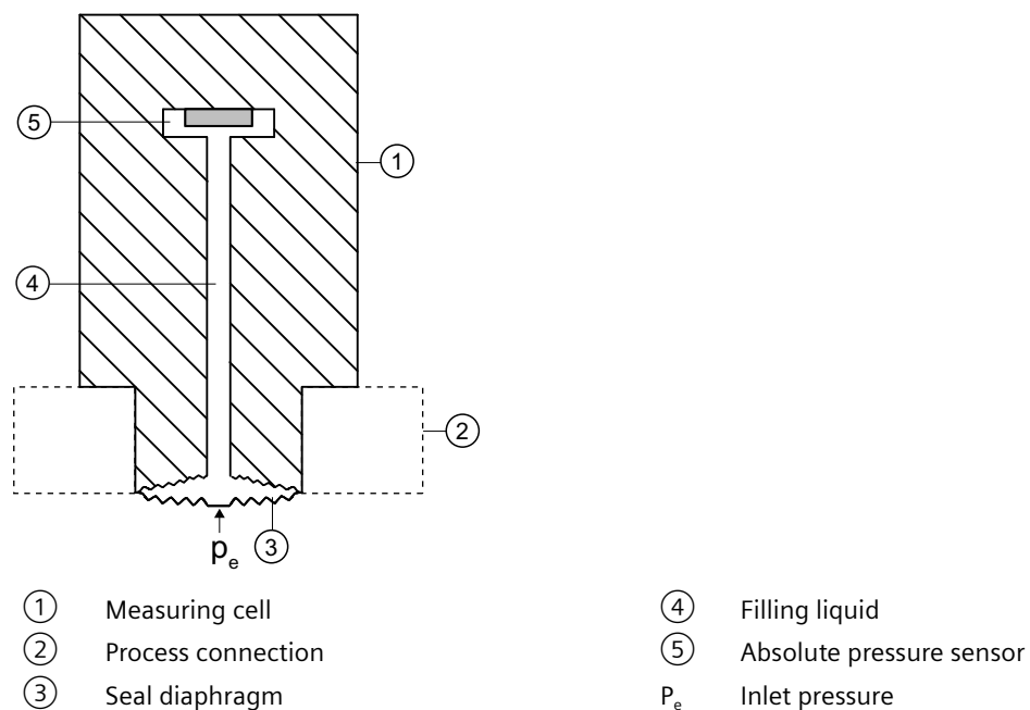
Figure 4-7 Function chart of measuring cell for absolute pressure
