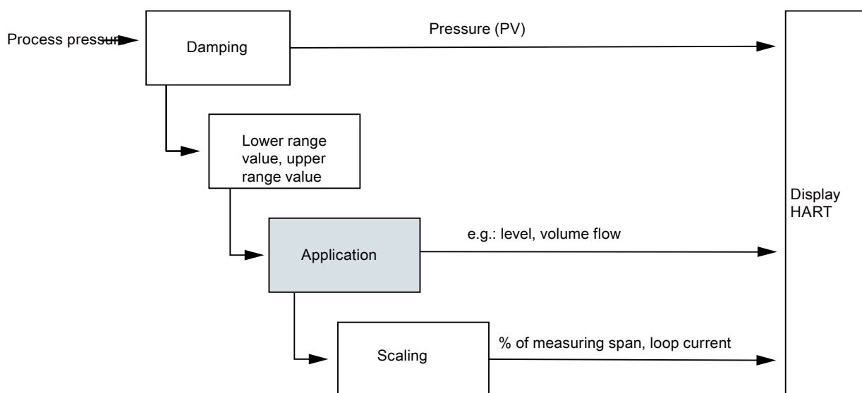
Figure 9-1 Flow diagram
