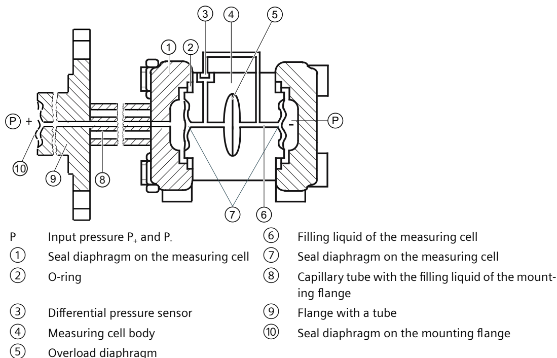
Figure 4-11 Function chart of the measuring cell for level
