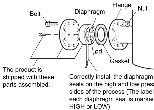
Figure 3.9 Mounting the Diaphragm Seals
