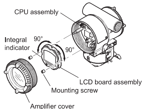
Figure 3.17 Rotating Integral Indicator
