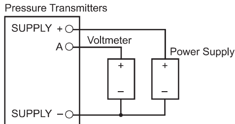
Three-Wire Connection
