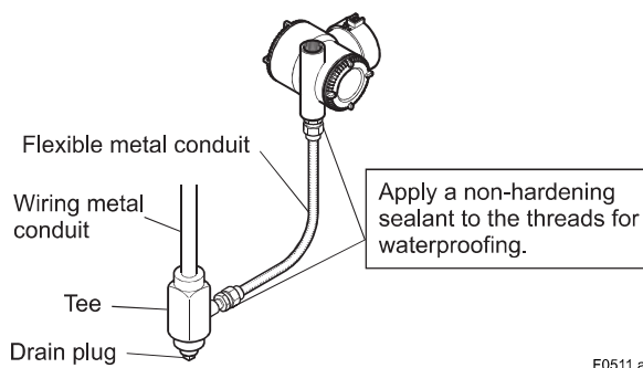
Figure 5.15 Typical Wiring Using Flexible Metal Conduit
