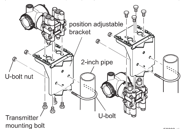
Figure 3.3 Transmitter Mounting (Vertical Impulse Piping Type)
