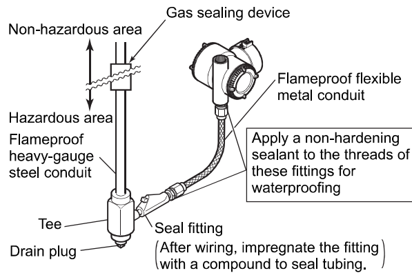
Figure 5.17 Typical Wiring Using Flameproof Metal Conduit
