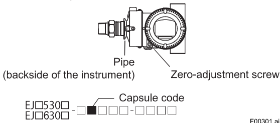
Figure 3.1 EJ□530□ and EJX630A Horizontal Mounting Position
