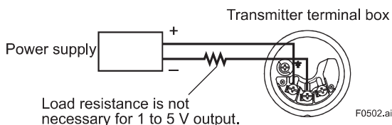
Figure 5.3 Power Supply Wiring Connection
