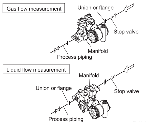
Figure 4.10 Process Piping Connection Examples (EJ□115□)
