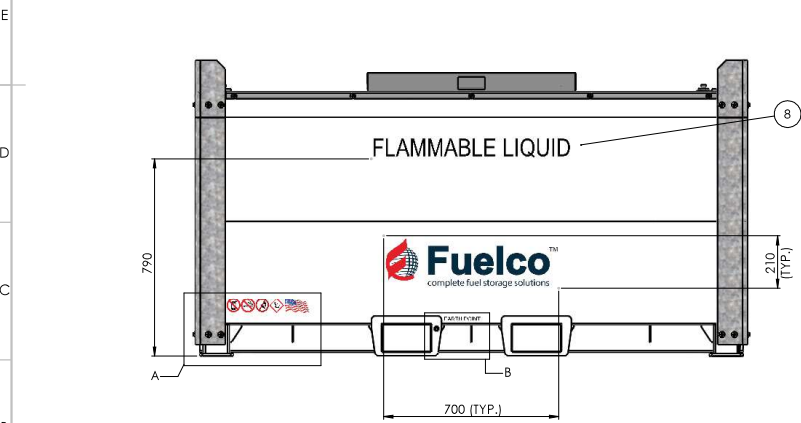
LTSK-1902 - FRONT & REAR - DECAL MAP
