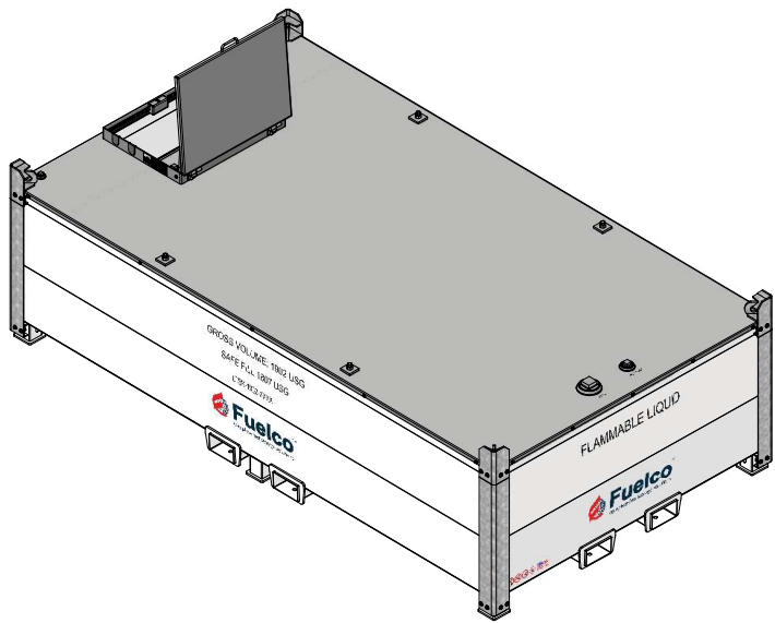
VIEW #1: - REAR NOZZLE ARRANGEMENT
