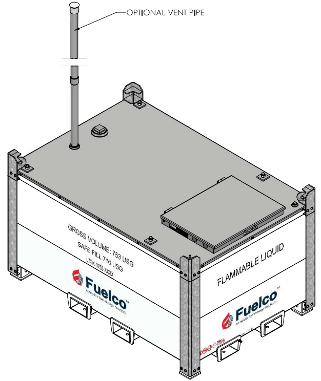
VIEW #2: - OPTIONAL VENT PIPE
