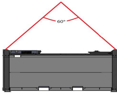
Figure 2 – Tank Lifting Diagram
