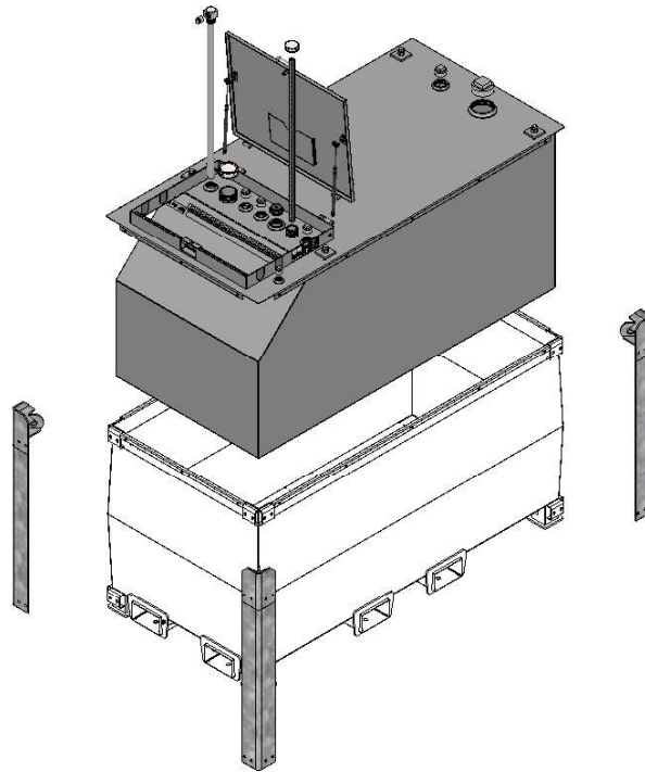
Figure 10 – Tank Separation Diagram
