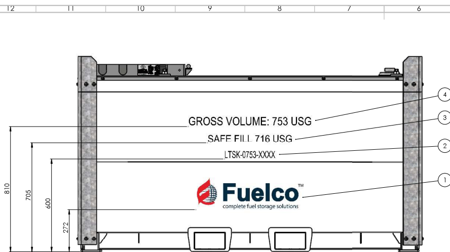
LTSK-0753 - LHS & RHS - DECAL MAP
