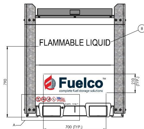
LTSC-0545 - FRONT & REAR - DECAL MAP
