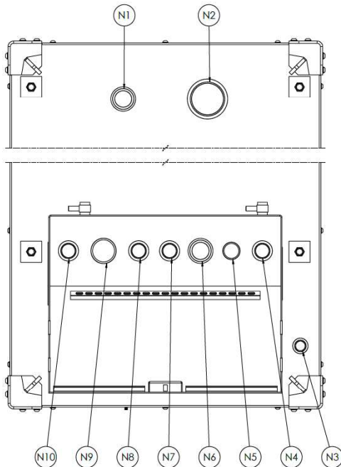
Figure 7 Nozzle Diagram
