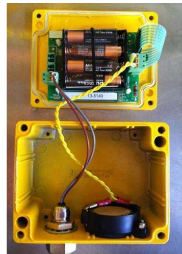
Figure 9 - Overfill Alarm Battery Replacement
