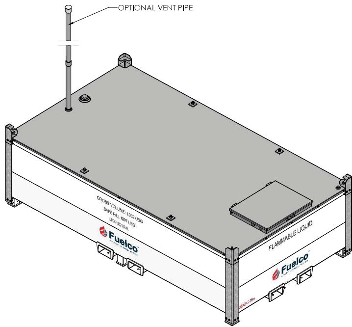
VIEW #2: - OPTIONAL VENT PIPE
