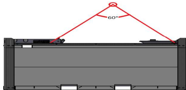
Figure 11 – Primary Tank Lifting Diagram
