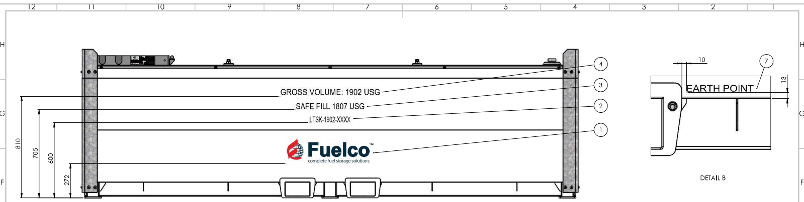
LTSK-1902 - LHS & RHS - DECAL MAP
