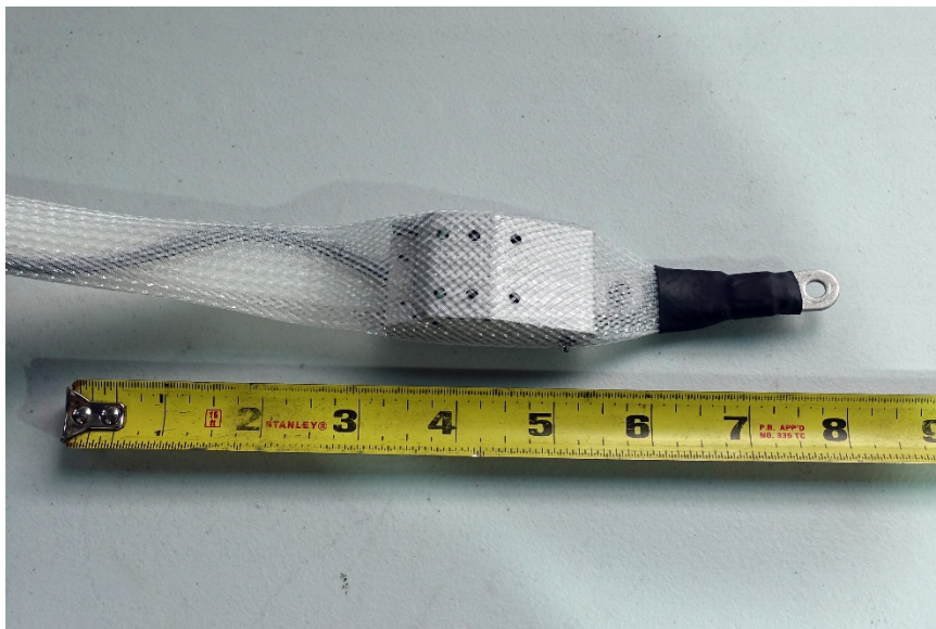
Photo #3: Sensor Type 63409 for Fiberglass Tanks
