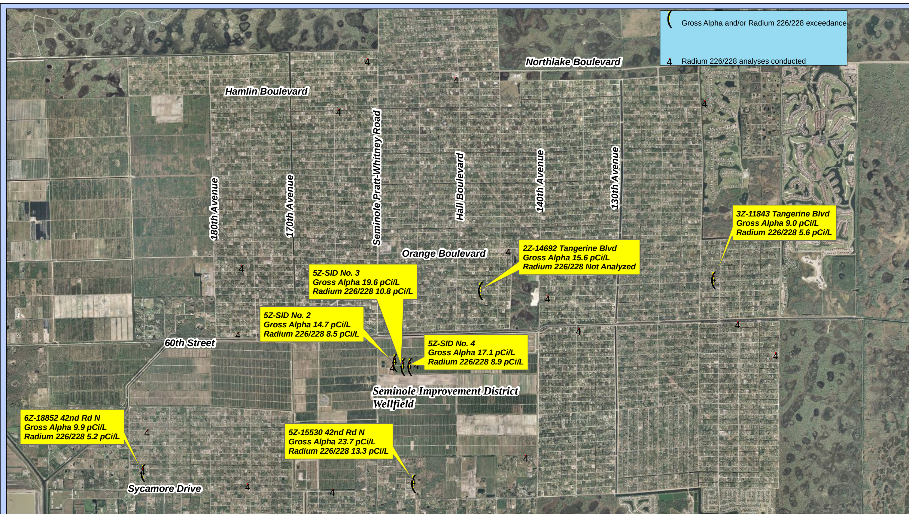
Figure 2: Gross Alpha and/or Radium 226/228 Exceedances in Ground Water Site # 618 The Acreage Loxahatchee, Palm Beach County, Florida FDEP-Site Investigation Section
