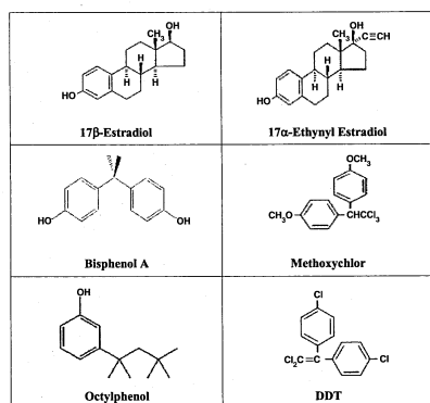
Figure 1. Structures of estrogenic compounds.
