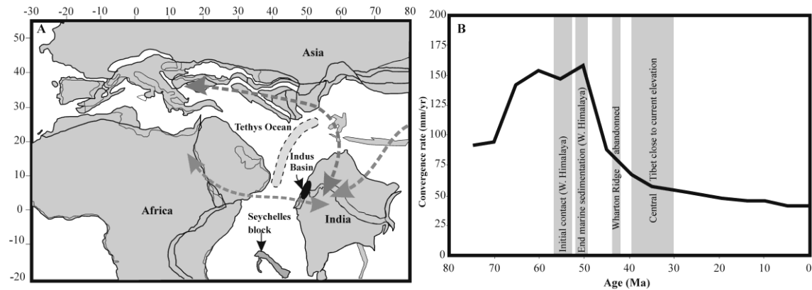
Figure 11. Palaeogeography and collision history of the Indian sub-continent. A, Earliest Eocene (SBZ5/6 biozones) reconstruction (based on Smith et al. 1994 with data from Gaetani & Garzanti 1991; Gingerich et al. 1997). Dark grey dashed line with arrow heads show possible routes (through land masses) for rodent mammal migration between India and other continents. These land masses likely acted as geographic barriers for LBFs to reach shallow marine habitats of the Indian subcontinent. A postulated oceanographic barrier (possibly larger distances and/or eutrophic waters) is shown as a grey band between east and west Tethys, which may also have prevented LBFs migrating from west to east. B, Depicts the rate of convergence (black line) between India and Asia from 75 Ma (after Copley et al. 2010). The grey bands show the timings of notable events in the history of collision. The collision is thought to have begun at the western edge of the plate boundary during P-E boundary times (Rowley 1996; Copley et al. 2010).
