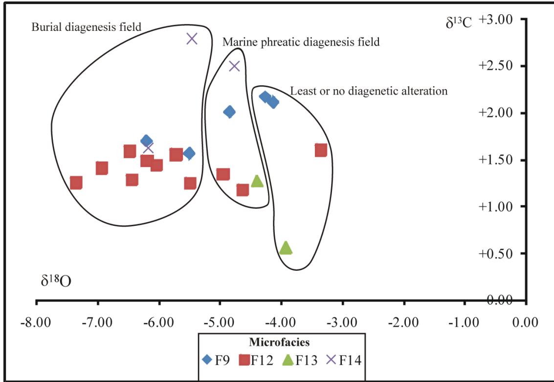
Figure 8. \delta^{18}\text{O} and \delta^{13}\text{C} values for diagenetic fields for carbonate microfacies of the Dungan Formation in the Hanna Lake section. Diagenetic fields are determined from petrographic (and not isotope) analysis.
