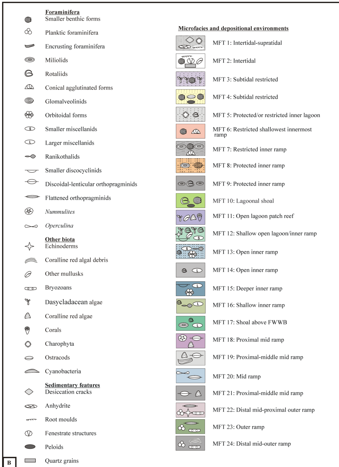
Figure 7A-B. Palaeoenvironmental evolution of major facies and biota of the Indus Basin through the Late Paleocene-Early Eocene. Not to scale. SL, sea level; FWWB, fair weather wave base; SWB, storm wave base.
