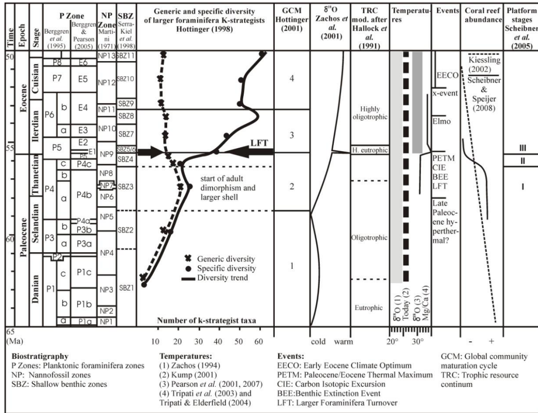
Figure 1. The Tethyan Paleocene to Early Eocene biostratigraphy, and comparison of trends in evolution of larger benthic foraminifera, \delta^{18}O isotopes, coral reef abundance, and trophic resource continuum (TRC: level of nutrients in ocean water) (after Scheibner & Speijer 2008a).
