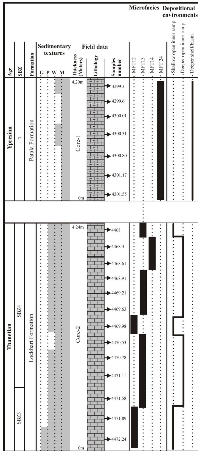
Figure 3. Lithological log of the Lockhart and Patala formations in the Shakardara Well-1 showing distribution of microfacies and depositional environments. LBF biozones (SBZ) after Afzal et al. (in press).
