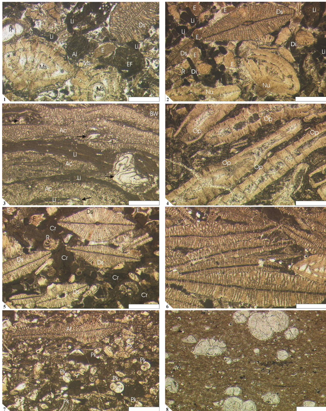
Plate 3. Early Eocene microfacies and palaeoecological assemblages. 1. Large miscellanid, smaller miliolid and rotraliid foraminifer grainstone (MFT17), showing large megalospheric Miscellanea (Ms), rotraliid (R) and discoidal Discocyclina (Ds) with fragmented Alveolina (Al), echinoderms, Lithothamnion coralline algae (Li) and encrusting foraminifera (EF), sample BD5. 2. Orthopragminid and Nummulites foraminifer packstone to grainstone (MFT18), characterized by Discocyclina (Ds) and Nummulites (Nu) associated with fragmented Lithothamnion (Li) and Distichoplax biserialis (Di) coralline algae and echinoderms (E), sample BD15. 3. Encrusting foraminifer boundstone with bioclastic wackestone (MFT19), note the alternating crusts
