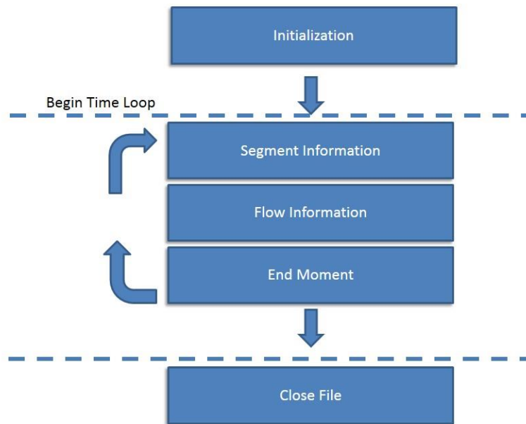
Figure 12 API Components
