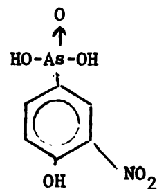
3-Nitro-4-hydroxyphenylarsonic acid
