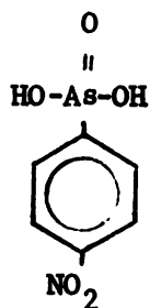
4-Nitrophenylarsonic acid
