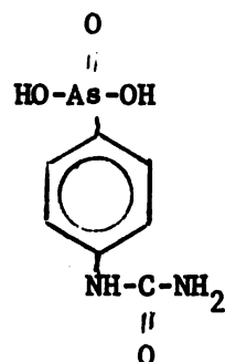
4-Ureido-1-phenylarsonic acid
