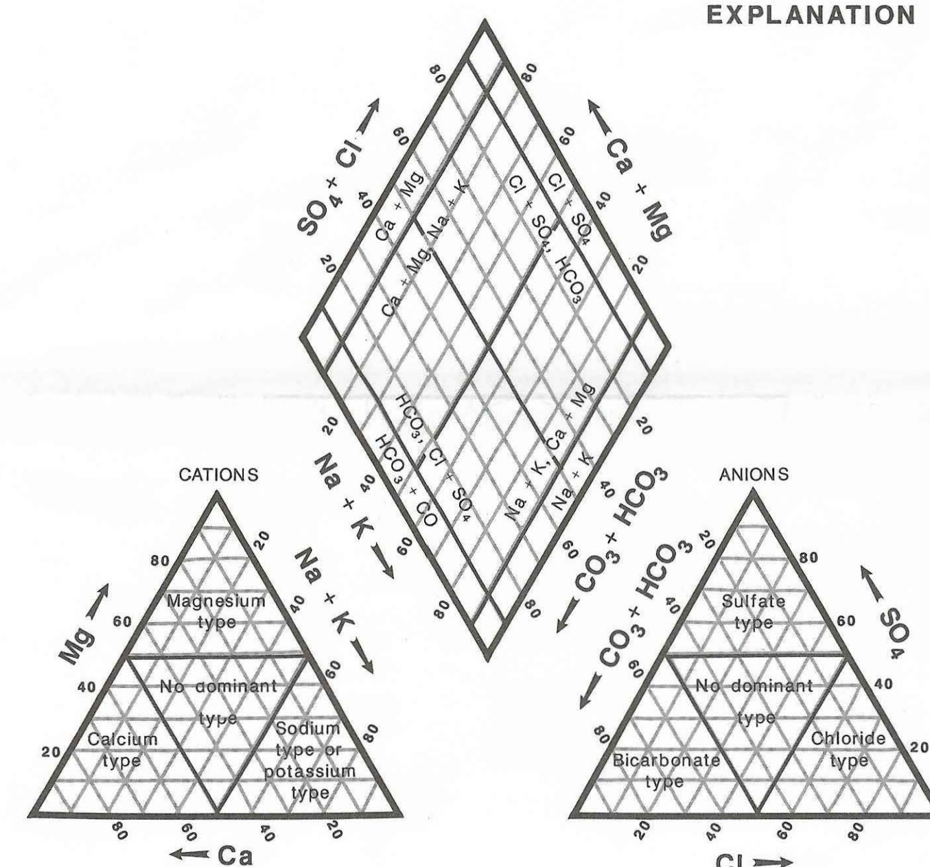
Piper Diagram. Shows relative percentages of major ions.
