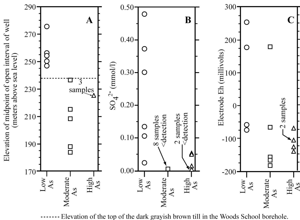
Figure 6. - Chemical and physical characteristics of low-As (<4 µg/l), moderate-As (4 µg/l to 20 µg/l), and high-As (>20 µg/l) samples. (For samples with As <7 µg/l, detection limit = 0.3 µg/l.)
