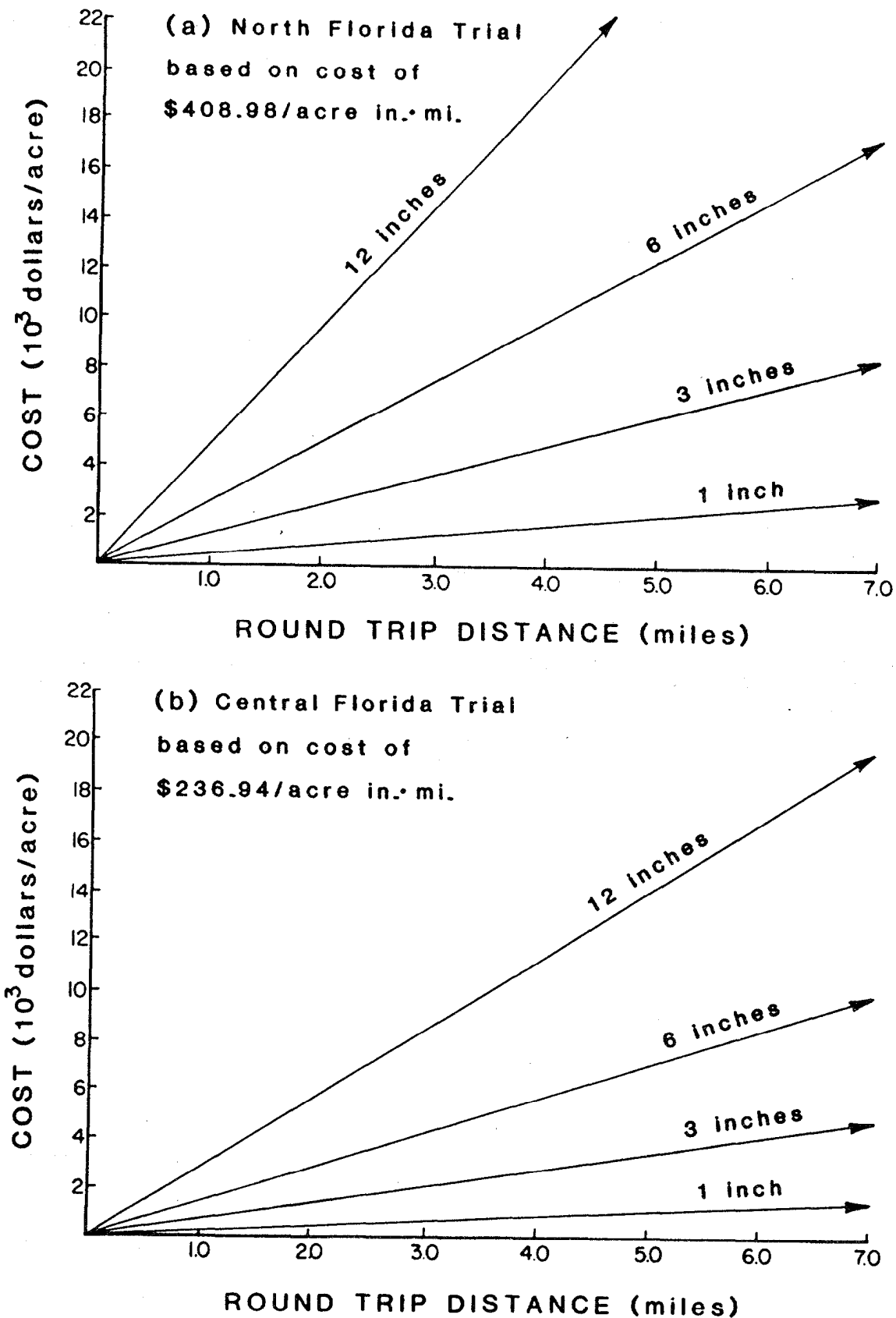
Figure 13. Travel distance and application rate versus cost per acre of applying peat material. a. based on Occidental's reclamation site. b. based on Gardinier's reclamation site.
