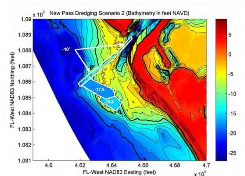
Figure 35. New Pass exterior navigation channel and southern ebb tidal shoal borrow areas used for the 2009 Lido Key Beach Renourishment Project (Spadoni et al., 2008).
