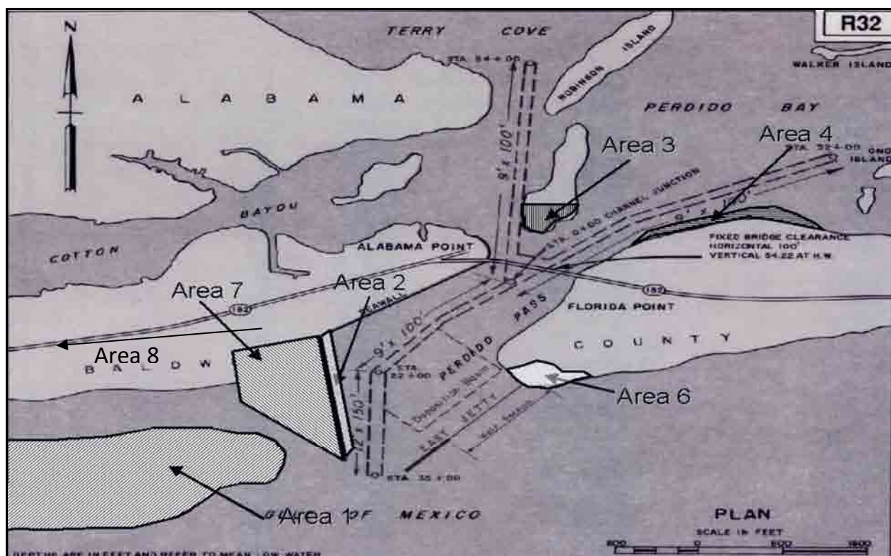
Figure 7. Authorized channel dimensions and disposal sites for the Perdido Pass project (USACE, 2009).
