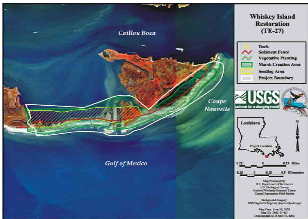
Figure 24. Whiskey Island Restoration Project (TE-27) (CWPPRA, 2002b).
