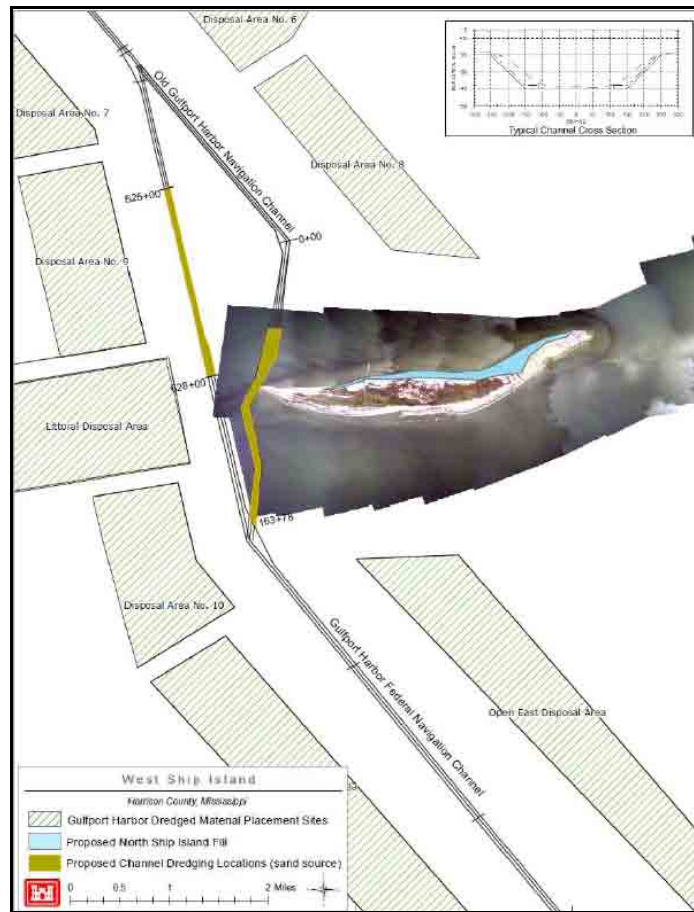
Figure 14. West Ship Island North Shore Restoration and proposed borrow areas (USACE, 2010b).
