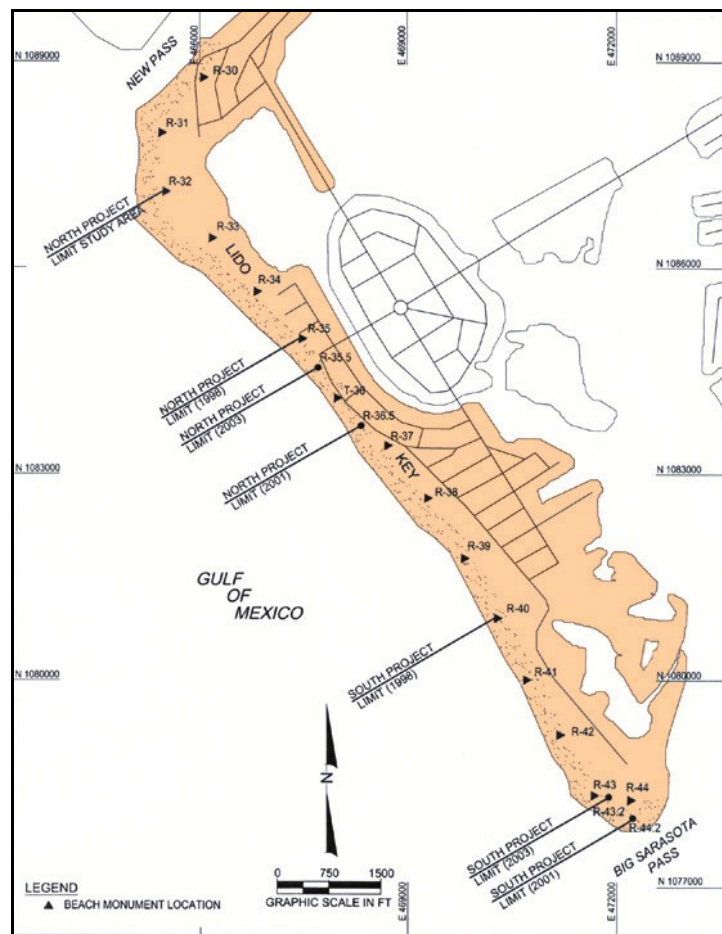
Figure 34. Lido Key beach nourishment performed in 1998, 2001, and 2003 (FSU, 2008).
