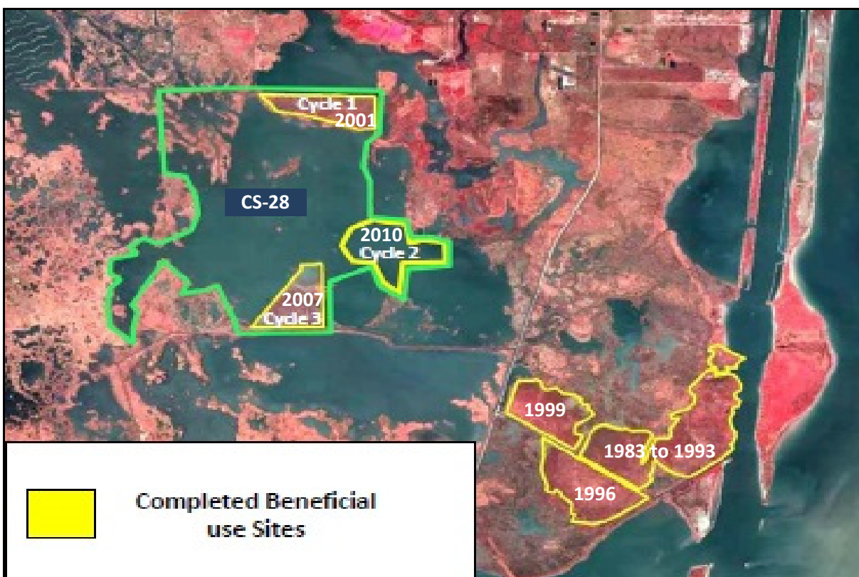
Figure 20. Beneficial use placement areas from 1983 to 2010 in SNWR (Modified from USACE, 2010).
