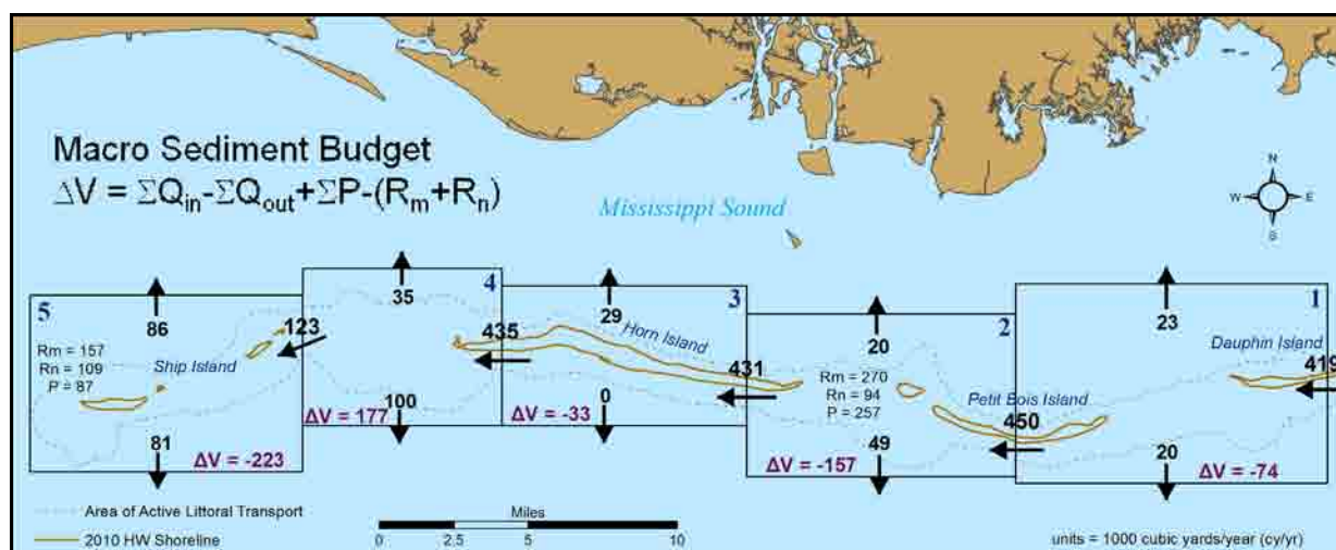
Figure 13. Macro sediment budget for the Mississippi barrier islands (from Byrnes et al., 2011); P is dredged material placement, R_m is sediment removal associated with maintenance dredging, and R_n is sediment removal associated with new work dredging.
