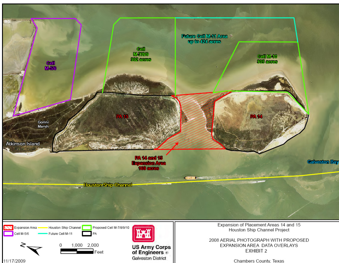
Figure 32. Proposed plan for expansion of Placement Areas 14 and 15 (USACE, 2010).
