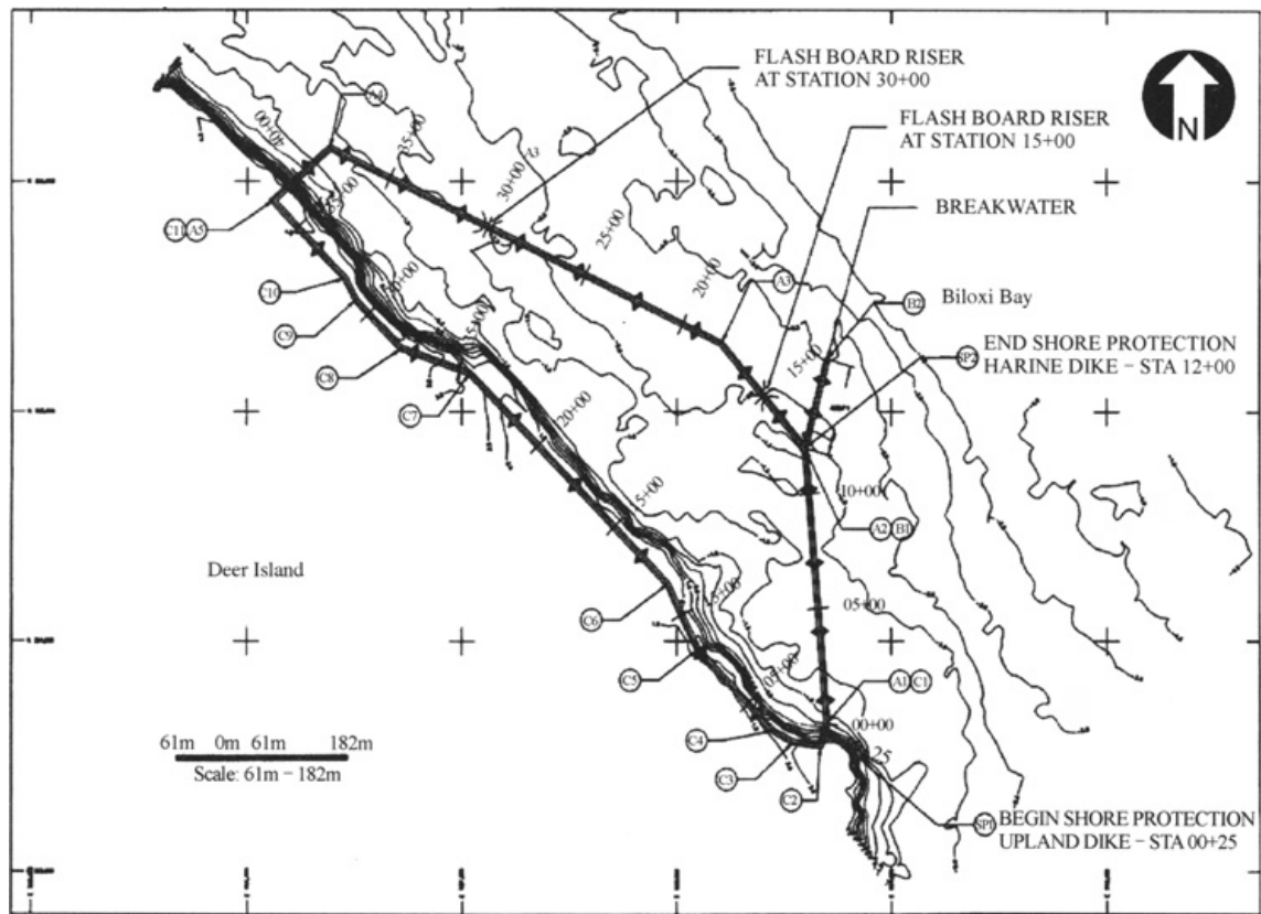
Figure 16. Site design plan for Deer Island Marsh Creation (Knott, 2008).
