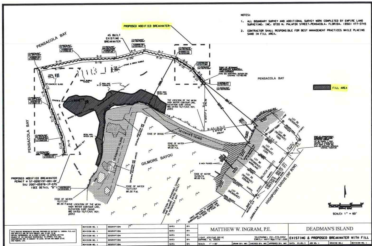
Figure 5. Deadman's Island Restoration Plan (USACE, 2011).
