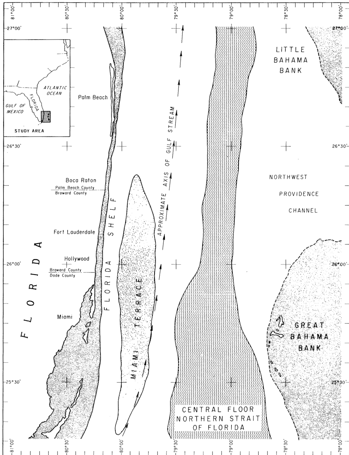
Figure 2. Chart of the northern part of the Straits of Florida.
