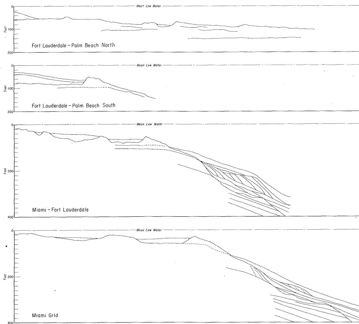
Figure A-4. Reduced seismic reflection profile data.
