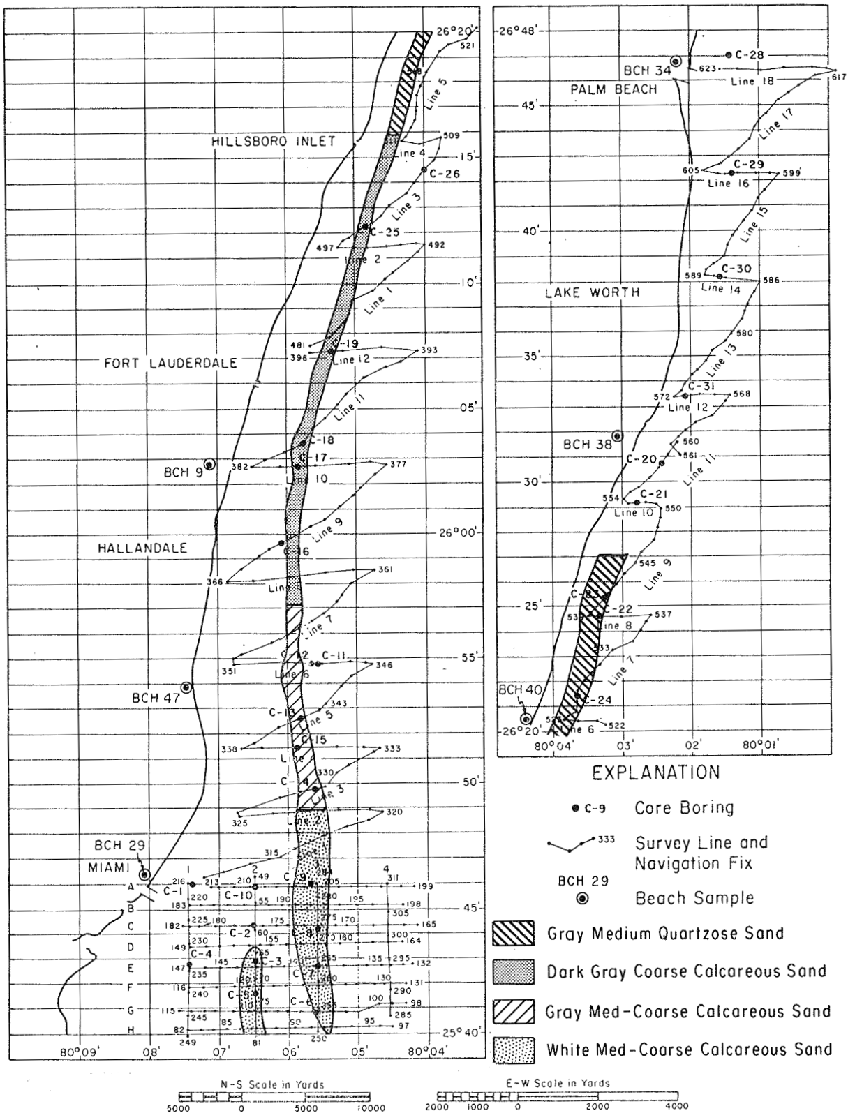
Figure 19. Areas most suitable for sand borrow.
