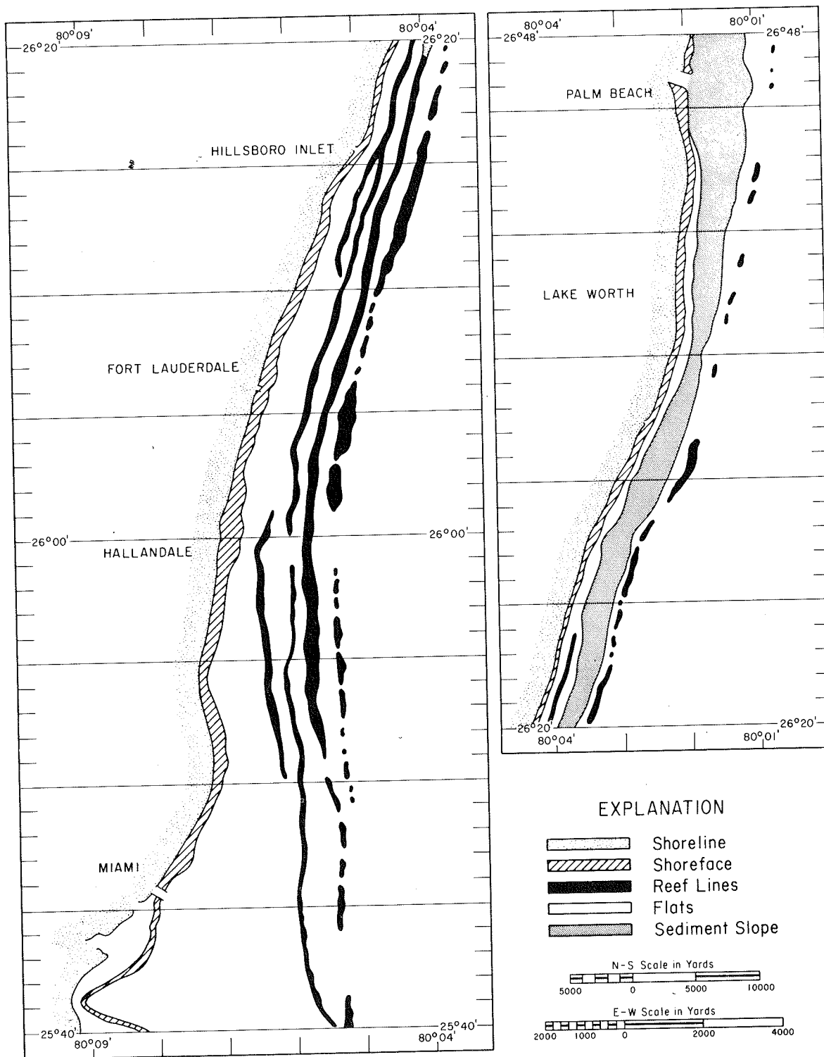
Figure 4. Plan of southeastern Florida shelf morphology.
