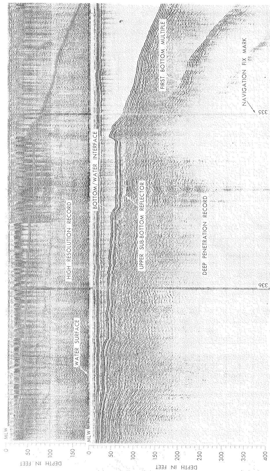
Figure A-1. Typical dual source seismic reflection profile.
