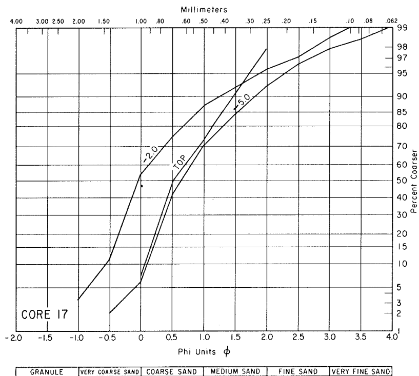
Figure 13. Cumulative curves, representative of offshore sediments in Section A.
