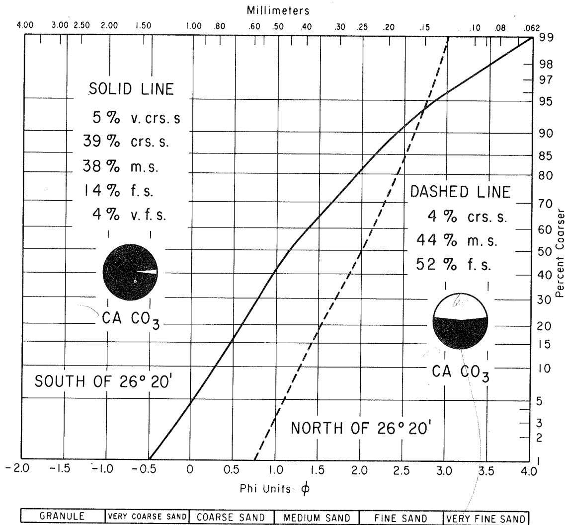
Figure 5. Average size distribution of shelf sediments. Note the difference in grain size and the concomittant difference in carbonate (shell) content.
