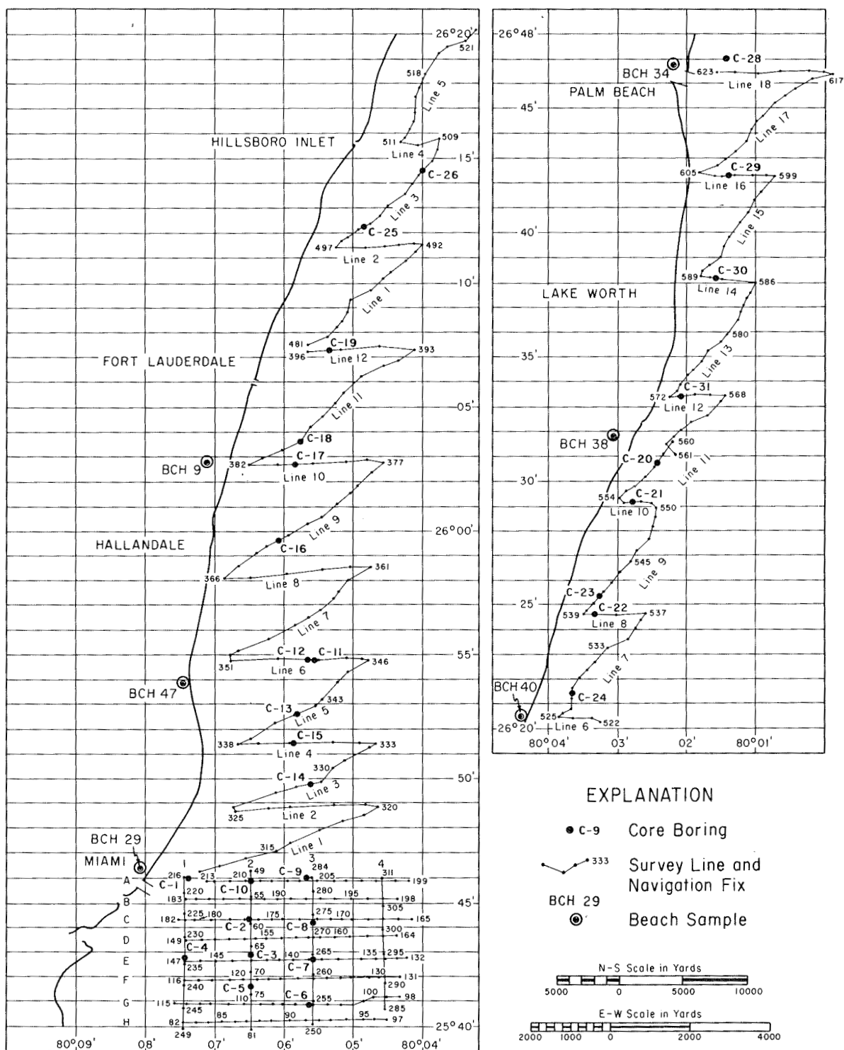
Figure 3. Plot of survey tracklines and core borings. Note change in horizontal scale which was enlarged to facilitate display.
