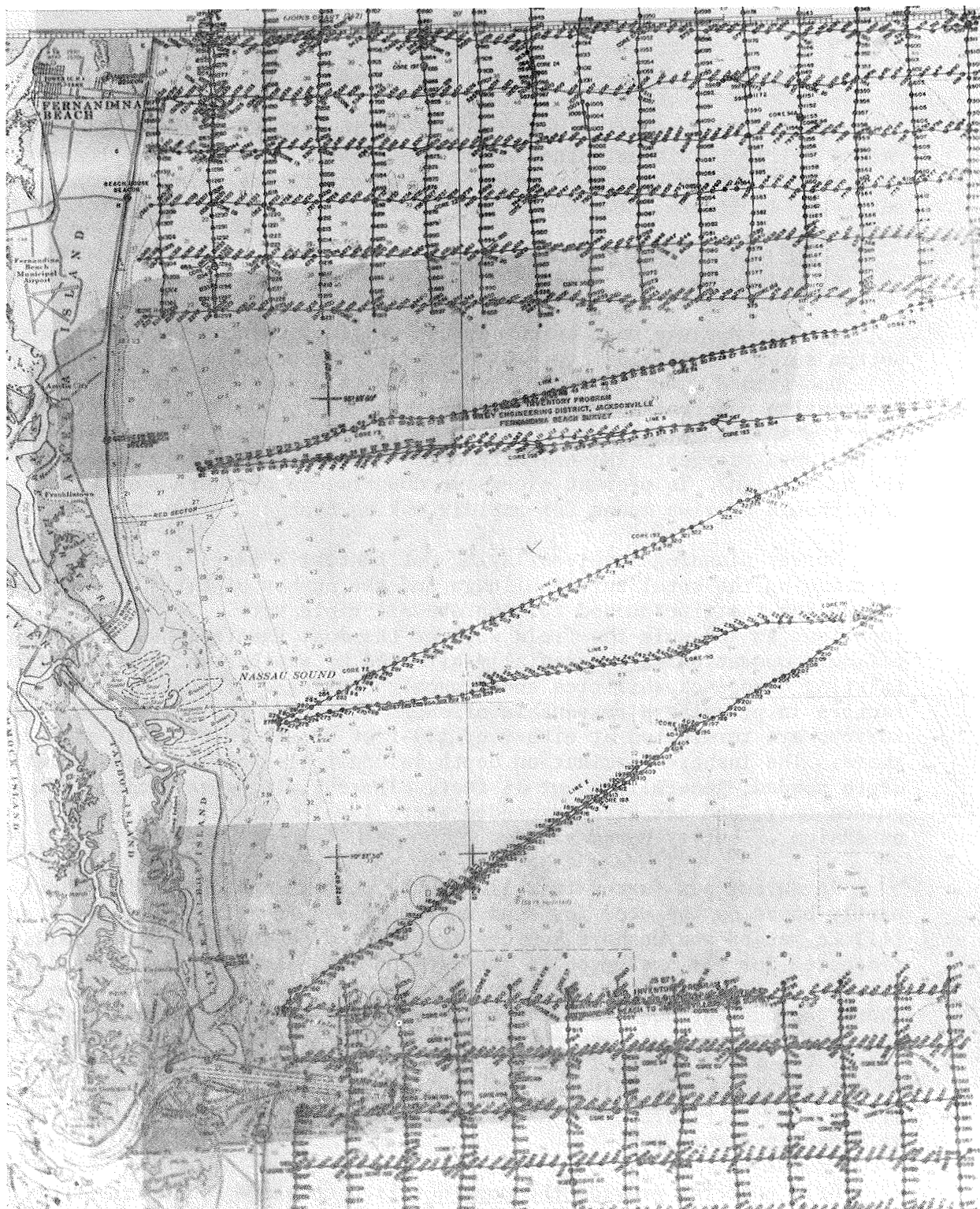
Figure A-2. Navigation chart with trackline overlays.
