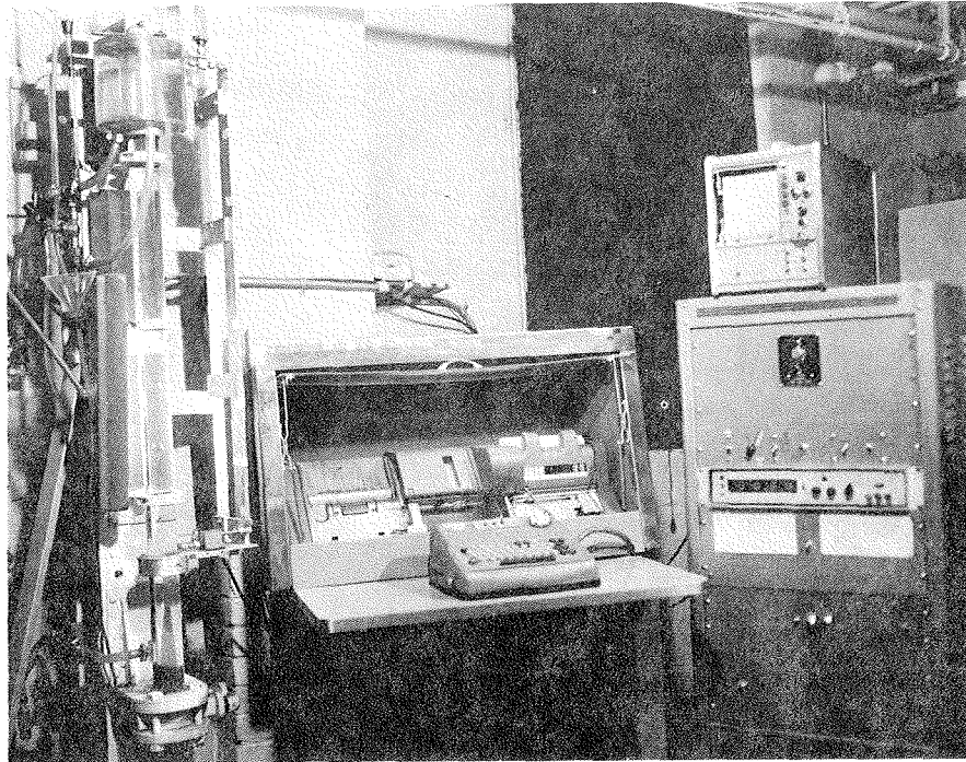
Figure 1. Rapid Sediment Analyzer. Settling tube and pressure tube are shown at left of photo; connecting tubes supply and drain water. At right is console housing digital voltmeter with timing and sampling circuitry; atop console is analog strip chart record for visual recording of pressure-time decay curve. In center is card punch for direct punching of data as sediment falls through metering column.
