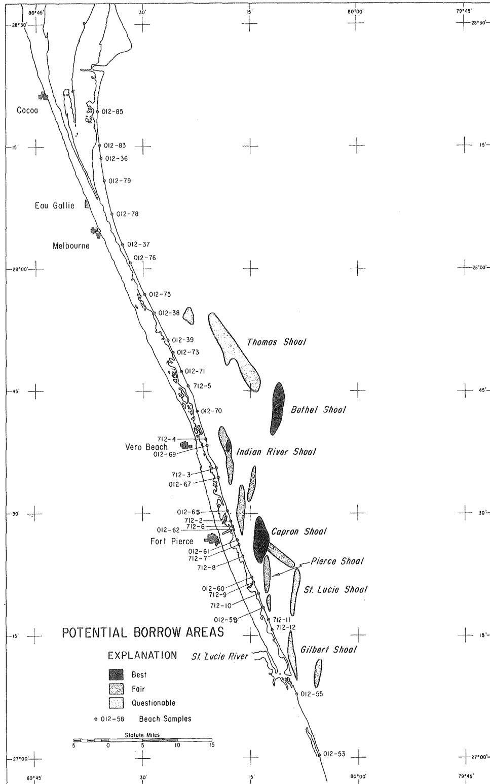
Figure 25. Map of Potential Borrow Sites in Study Area. Note locations of beach samples illustrated in Figures 23 and 24.
