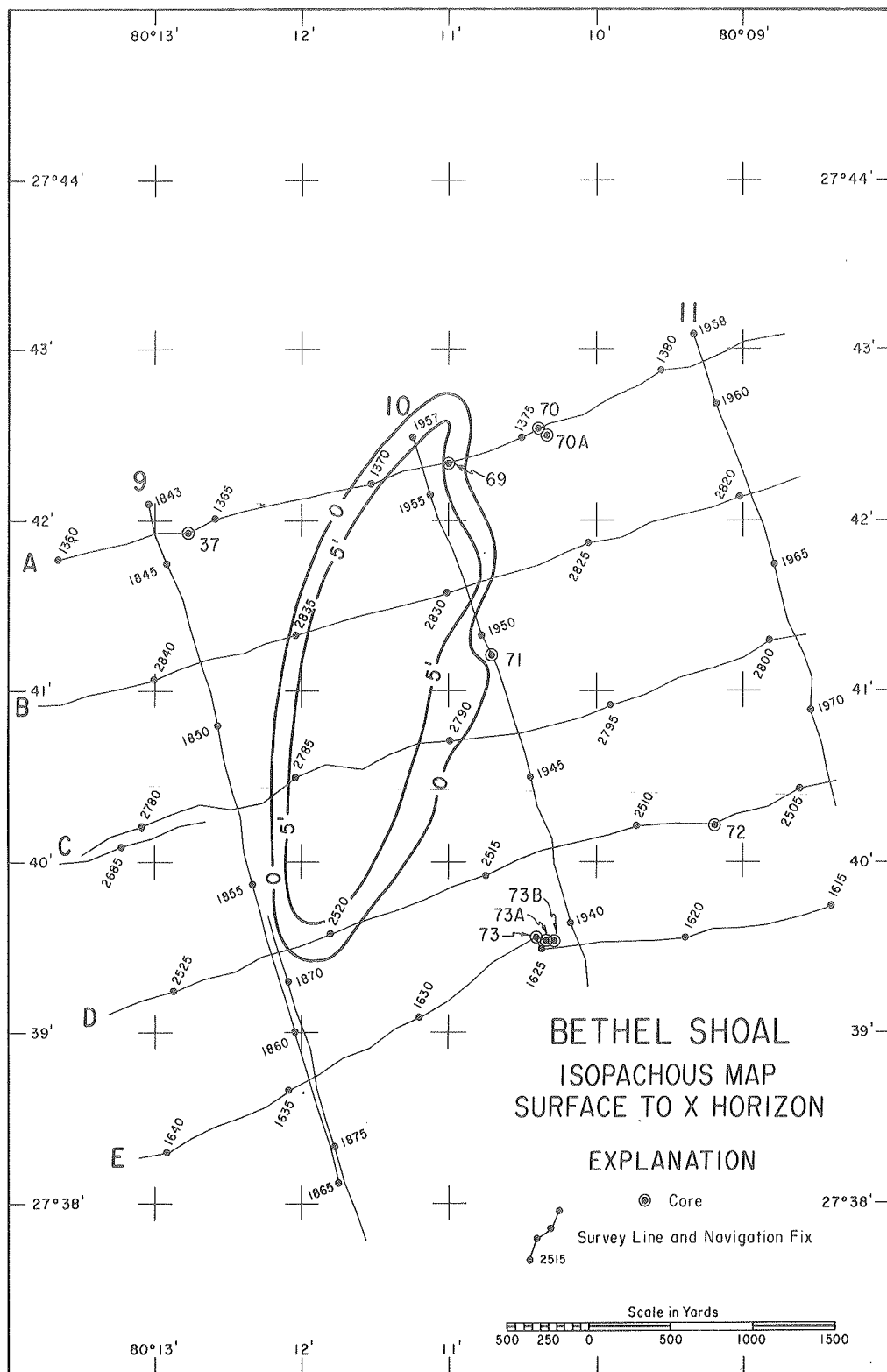
Figure 29. Isopachous Map of Sediment Thickness between the Water-Sediment Interface and the "X" Horizon Underlying Bethel Shoal.
