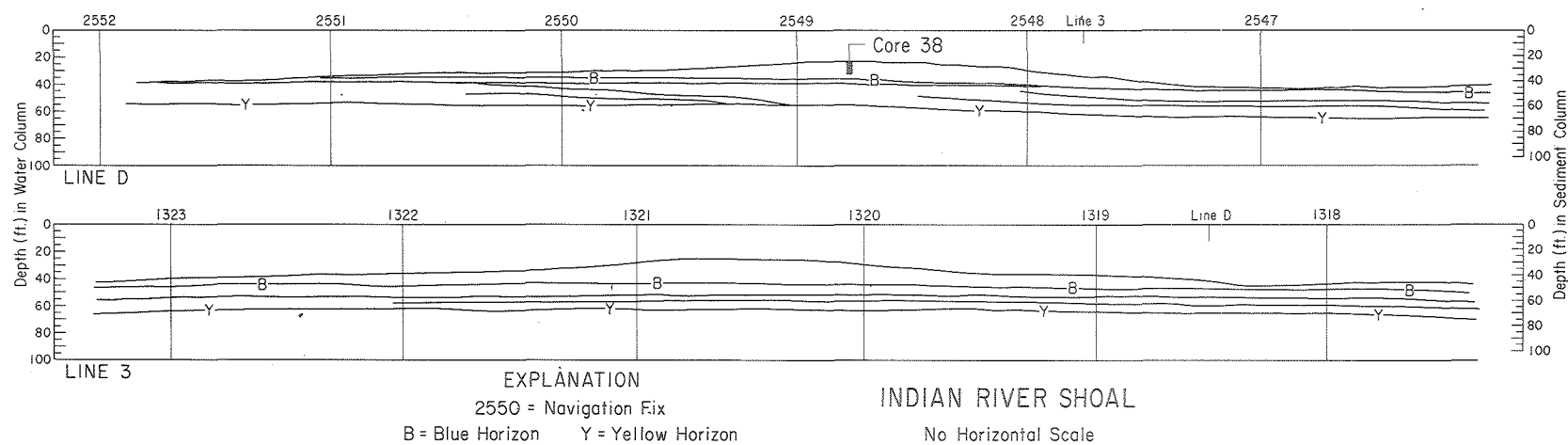
Figure 34. Line Profiles Showing Horizons under the Control Part of Indian River Shoal. See Figure 33 for location of tracklines and Appendix B for granulometric analyses of sediment.
