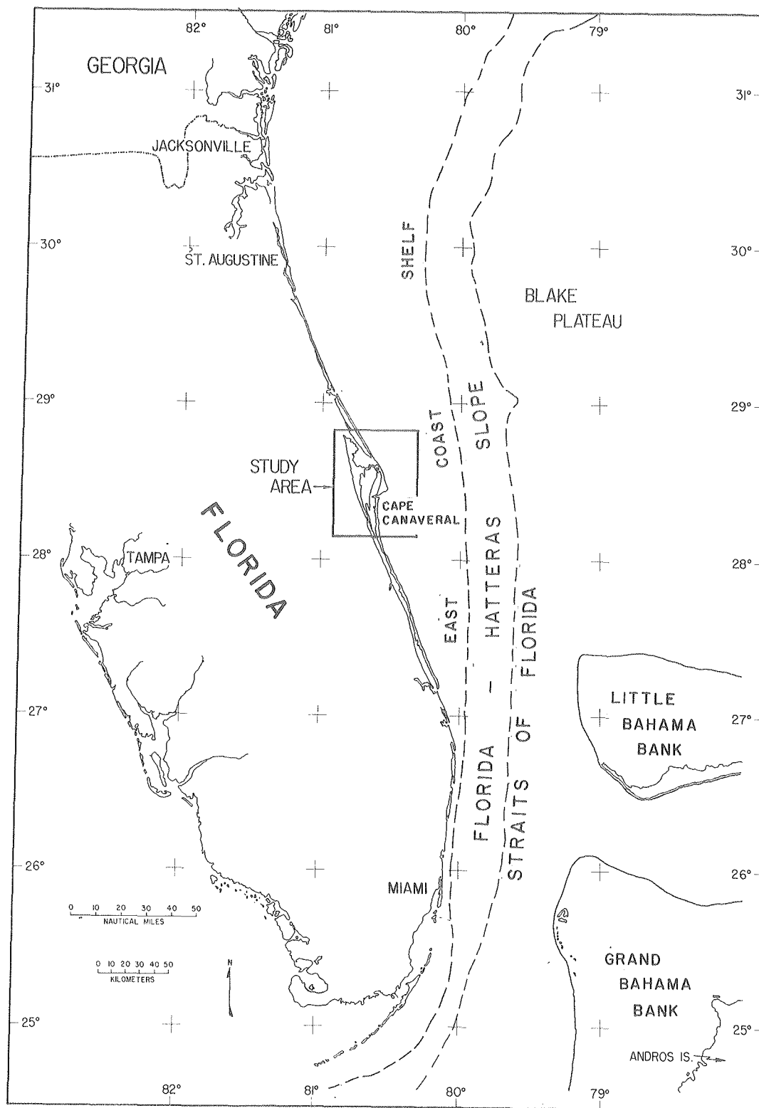
Figure 1. Map of the Major Physiographic Provinces of the Florida Continental Margin. The study area is outlined.
