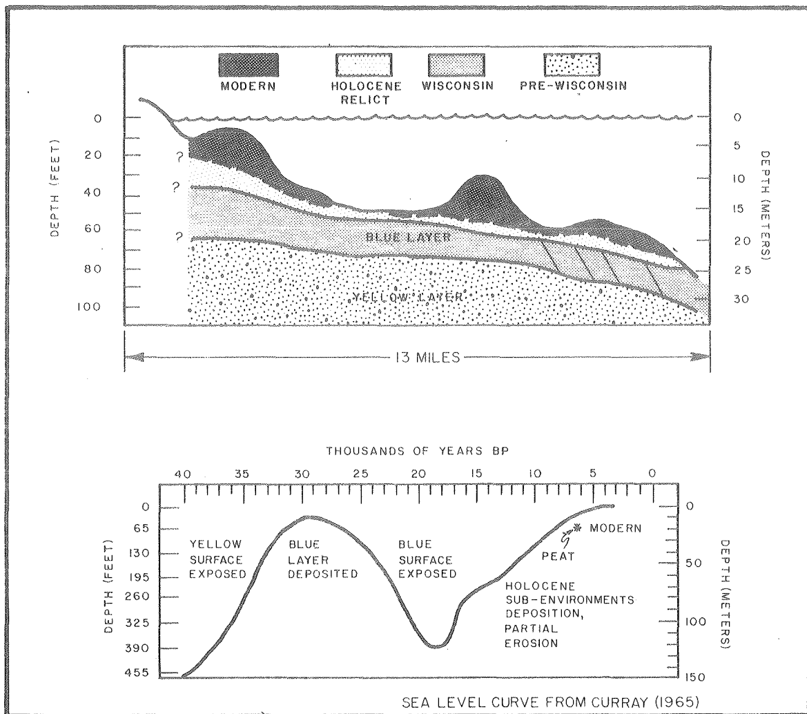
Figure 23. Cross Sectional Profile of the Cape Canaveral Inner Continental Shelf Showing Interpretations of Relative Age and Quaternary History. Major events are plotted on Curry's sea level curve.
