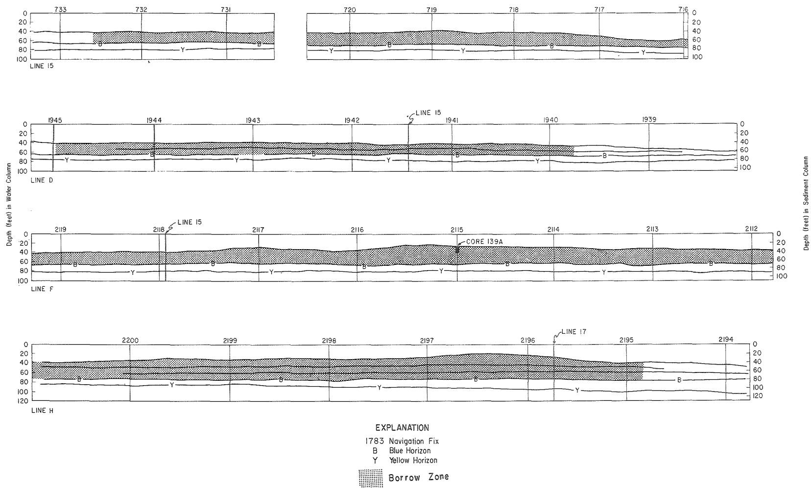
Figure 34. Interpreted Geophysical Profiles Across Representative Sections of Ohio-Hetzel Shoal
