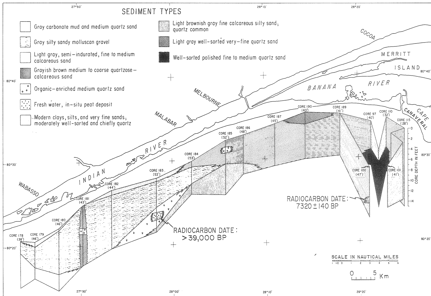
Figure 16. Fence Diagram Illustrating Spatial Distribution of Lithologies South of Cape Canaveral
