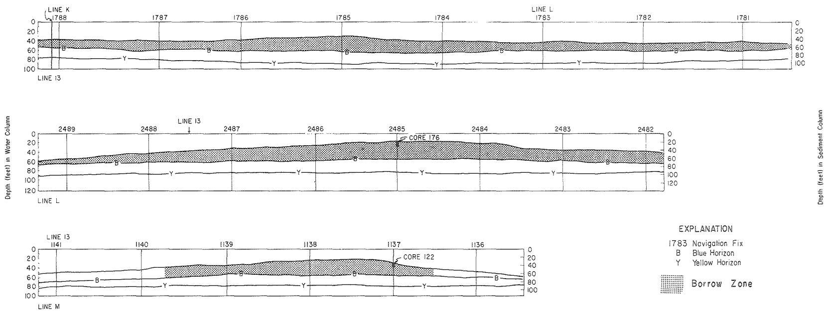
Figure 32. Interpreted Geophysical Profiles Across Representative Sections of The Bull (shoal)
