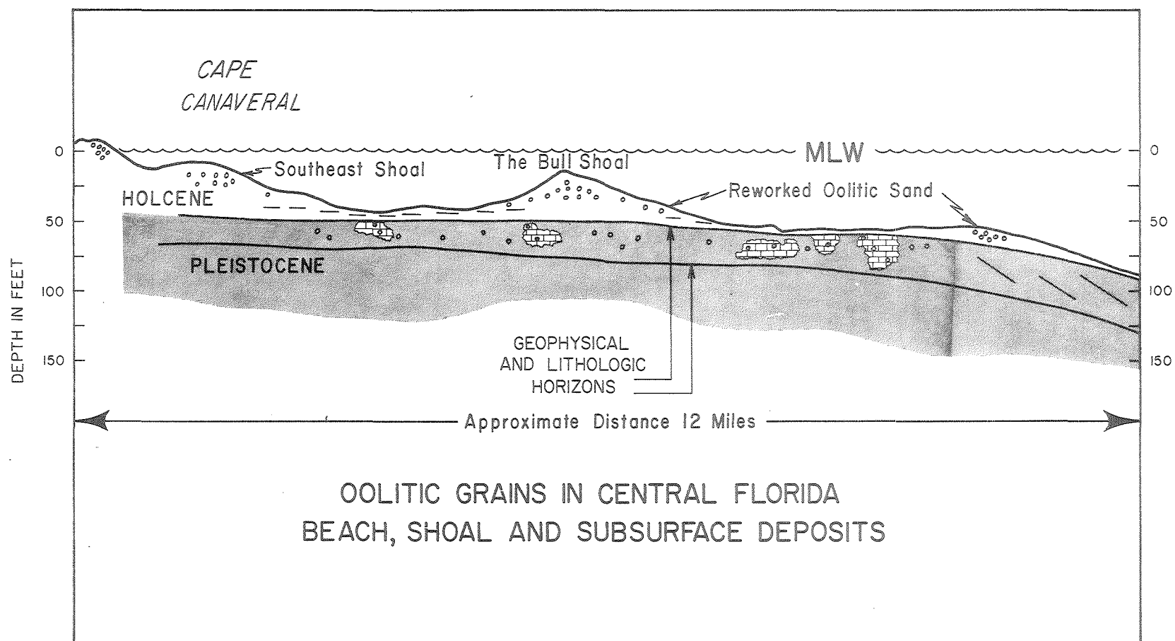
Figure 22. Schematic Diagram Showing the Vertical and Horizontal Occurrence of Ooids. Ooids in surficial deposits show the derivation of some surface sediment from underlying deposits; ooids on beaches suggest an exchange of material is occurring between the beach and the shoals.
