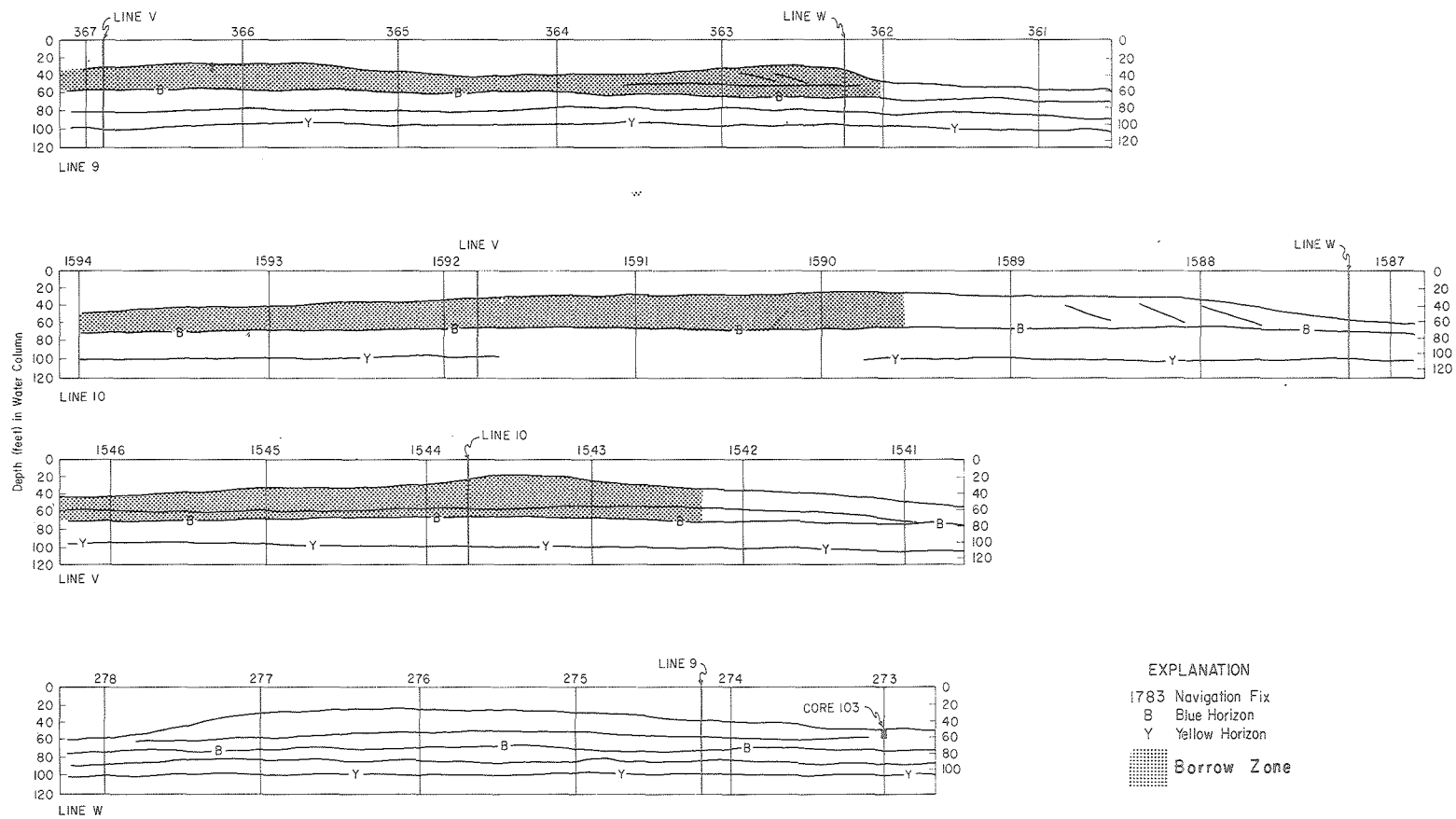
Figure 30. Interpreted Geophysical Profiles Across Representative Sections of Southeast Shoal
