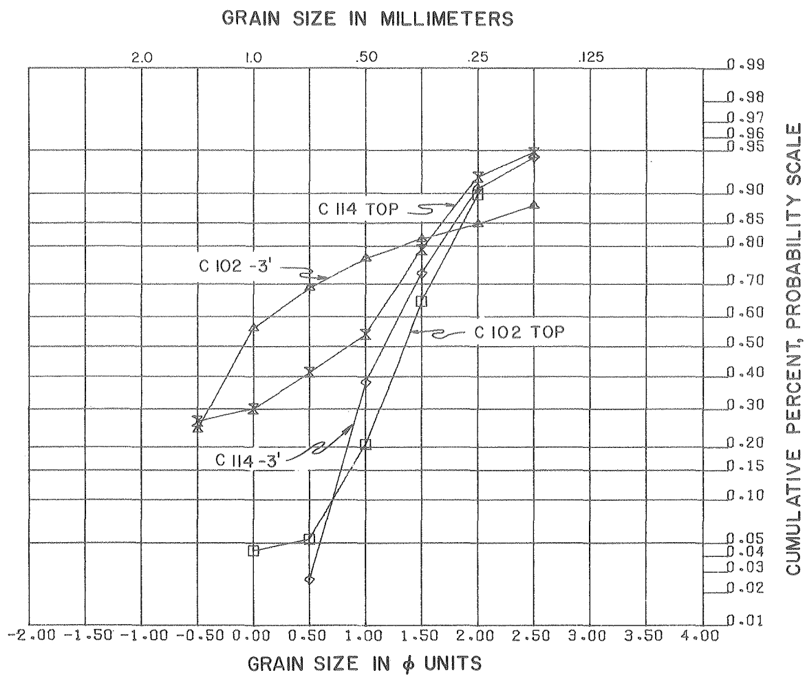
Graphic Size Distribution Curves for Selected Samples from Southeast Shoal. Location of samples is shown in Figures 2 and 29.
