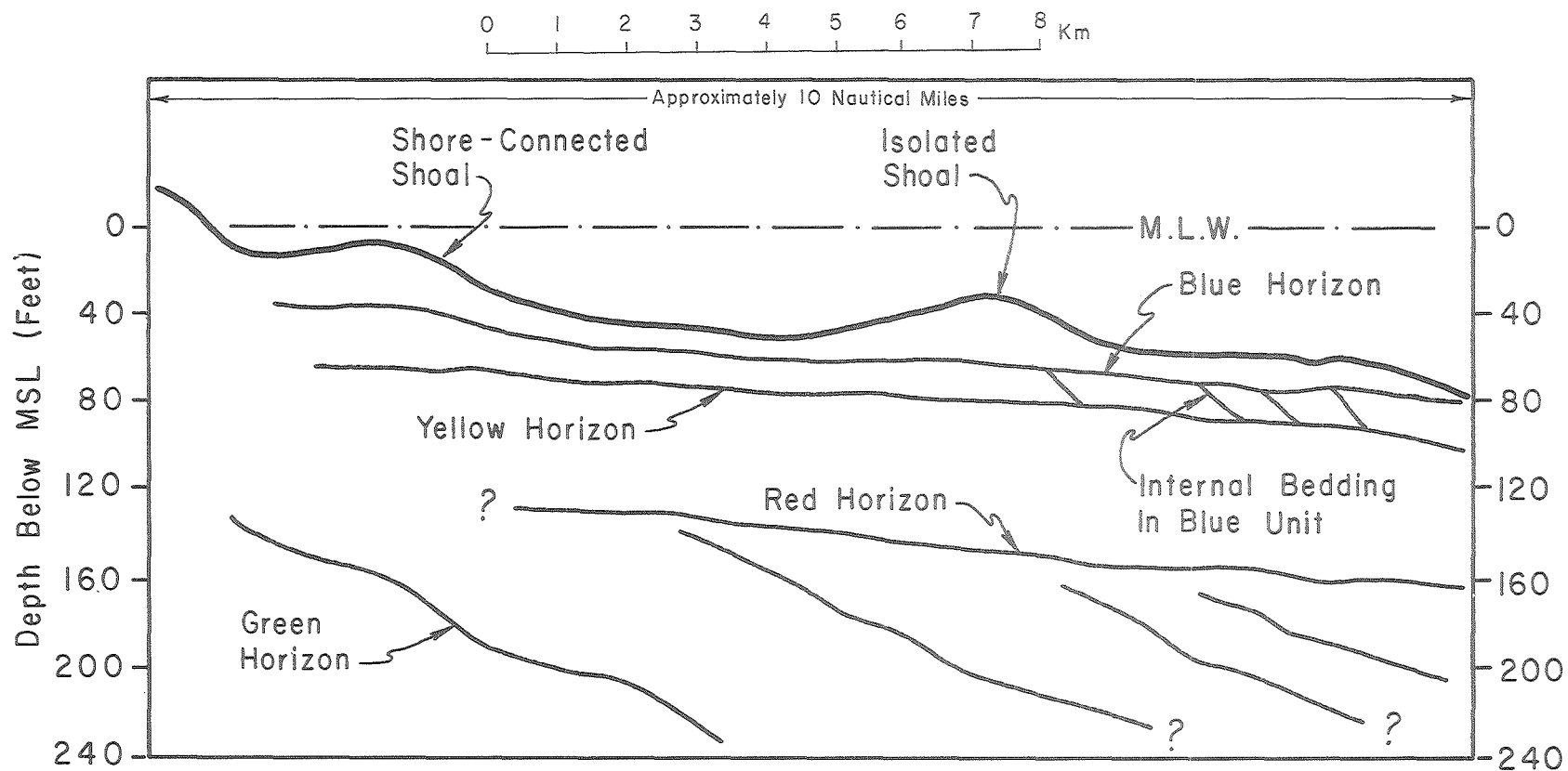
Figure 6. Schematic Profile Across the Cape Canaveral Inner Continental Shelf Showing Characteristics of Bottom Morphology and Major Shallow Acoustical Reflectors
