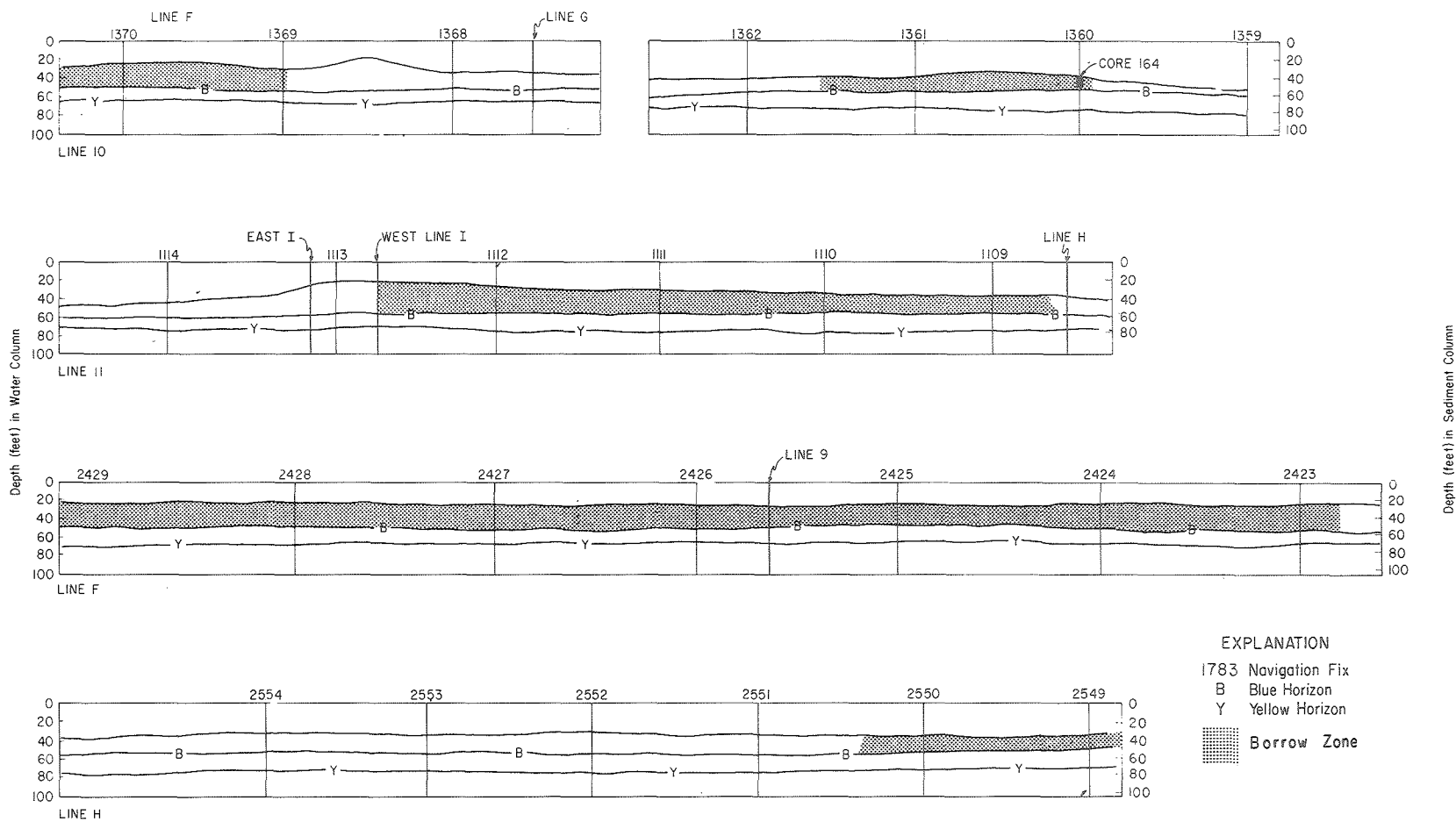
Figure 28. Interpreted Geophysical Profiles Across Representative Sections of Chester Shoal
