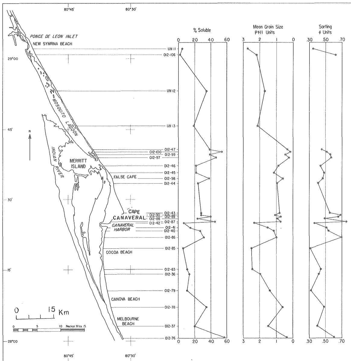
Figure 17. Percent Soluble, Mean Grain Size, and Sorting (Standard Deviation) Plotted for Areal Beach Samples. Note the similarities of the curves indicating the direct influence of shell material on textural parameters.
