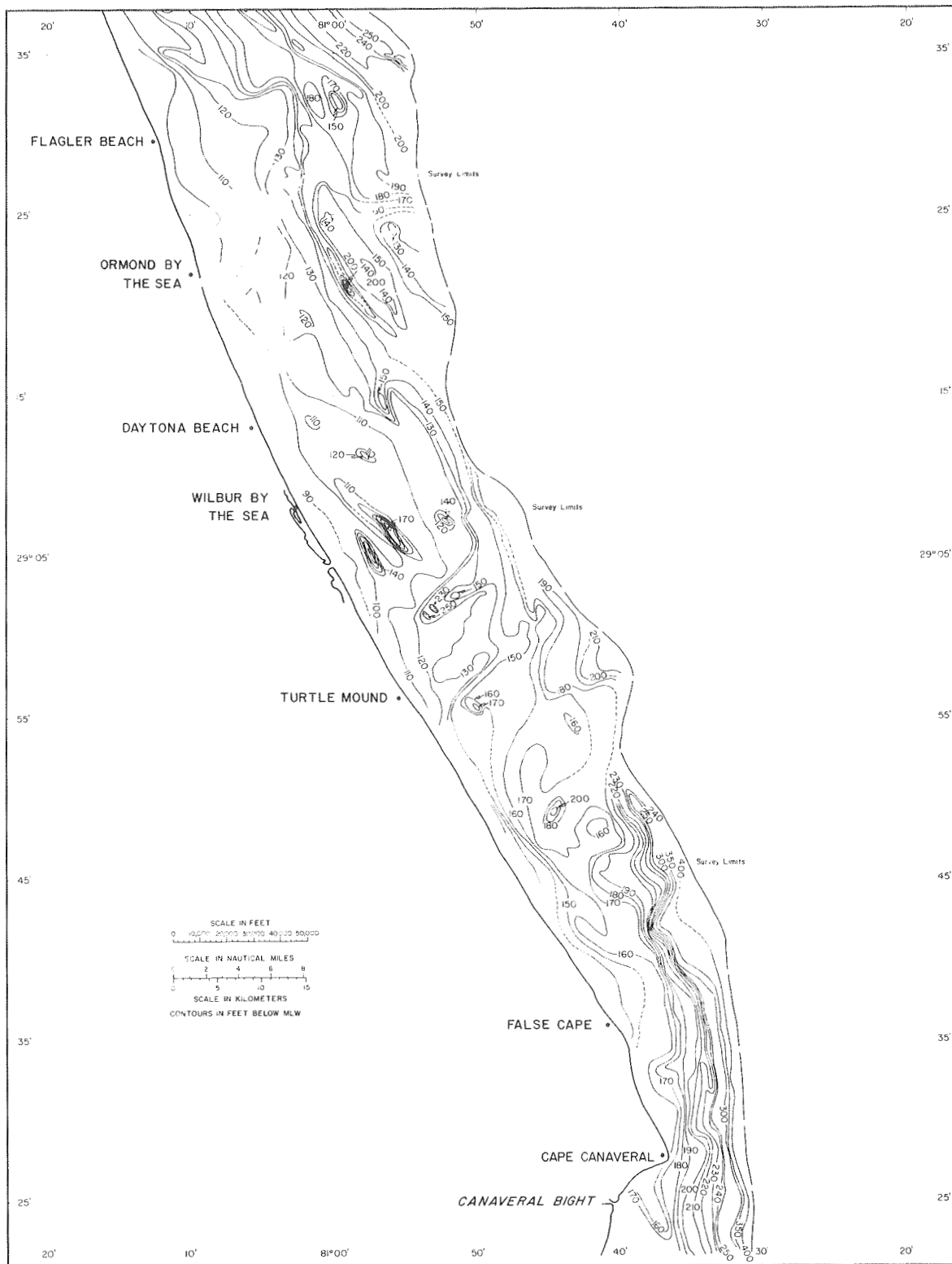
Figure 19. Contour map on the surface at the green reflector (south part).
