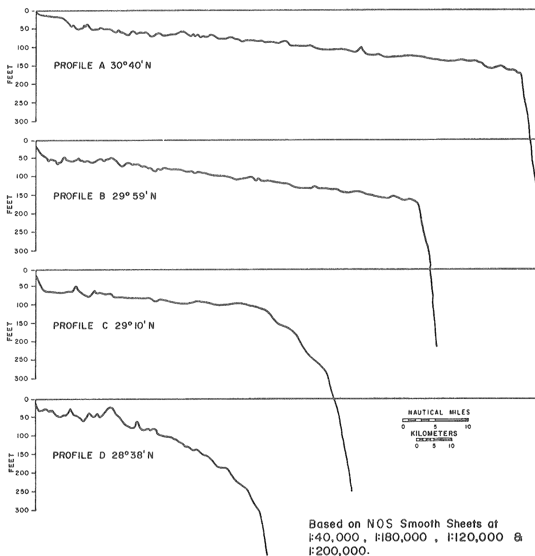
Figure 8. Representative shelf profiles from the north Florida East Coast Shelf. See Figure 6 for location of profiles. Note progressive increase in shelf floor width and decrease in shelf edge width northward.
