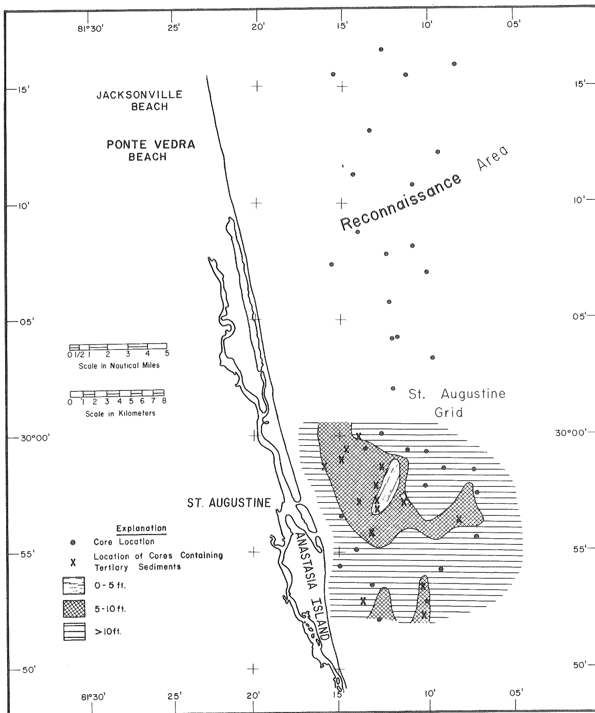
Figure 33. Map of the Jacksonville to St. Augustine area showing relationship between depth to first reflection and locations of cores bearing Tertiary sediments. Depth to first reflector, or overburden thickness, was determined by acoustic data and is indicated by a Zip-a-tone pattern. Note the close association. Acoustic data north of St. Augustine (reconnaissance line) is too sparse to contour. Note the close association in the grid area of cores containing Tertiary material (X's) with acoustic data showing areas of thin (< 10 feet) overburden. Shore-normal lines in the grid area refer to lines in Figure 26. This figure (at same scale) ties to Figure 22.
