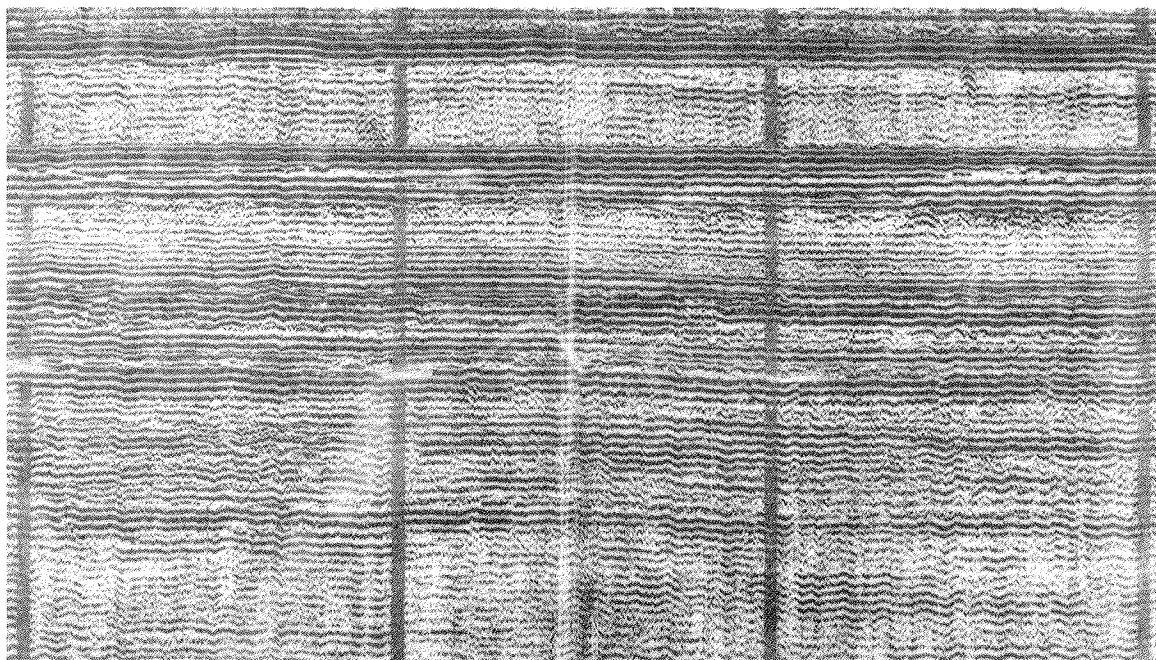
Section of St. Augustine—Cape Canaveral reconnaissance line D showing typical undulatory flexures characteristic of shallow subbottom strata underlying the inner shelf.
