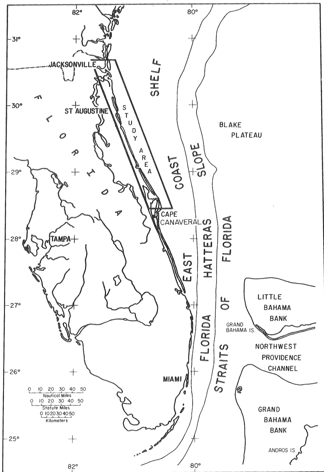
Figure 1. General map of the Florida peninsula showing location of the study area.
