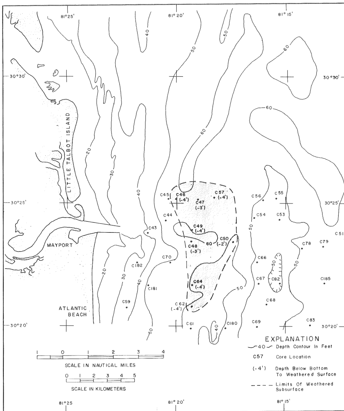
Figure 32. Bathymetric map of the inner shelf near St. Johns Inlet showing location of a subsurface soil horizon. Subsurface depth of weathered sediments is given for each core. The weathered zone unconformably overlies Tertiary deposits.
