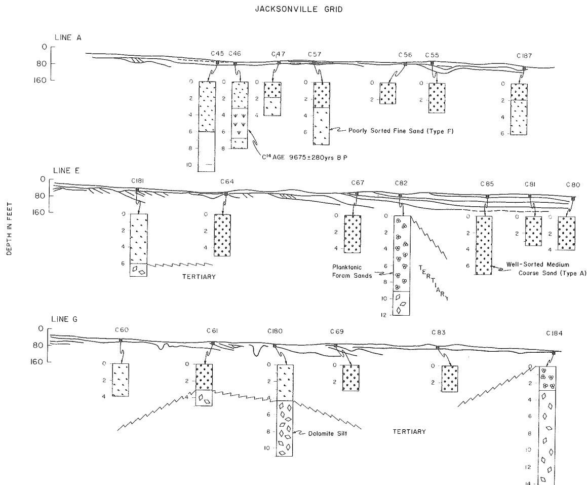
Figure 31. Shallow shelf stratigraphy along lines A, E, and G in the Jacksonville grid. Cores are plotted to scale on the reduced seismic profile and expanded below the line to show lithology. Tertiary sediments are correlated on basis of fauna and mineralogy.
