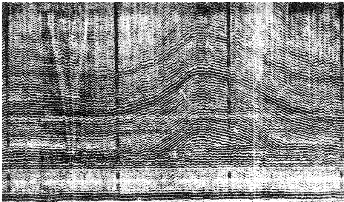
Section of St. Augustine–Cape Canaveral reconnaissance line B showing truncated syncline. Such pronounced structural features are rare in shallow subbottom strata under the inner shelf.
