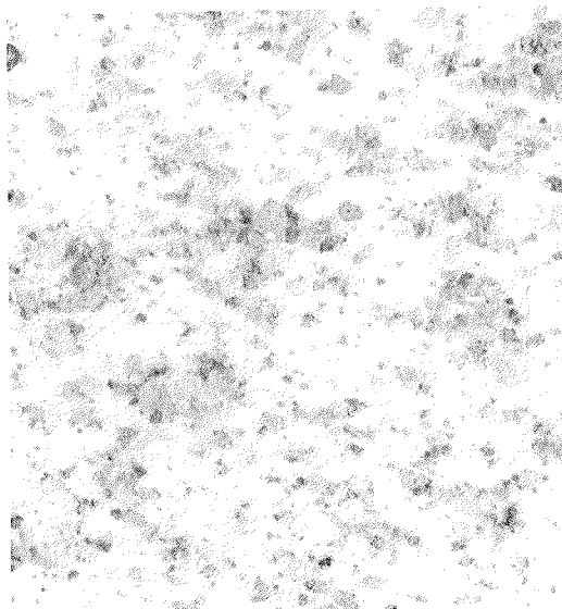
Thin Section
