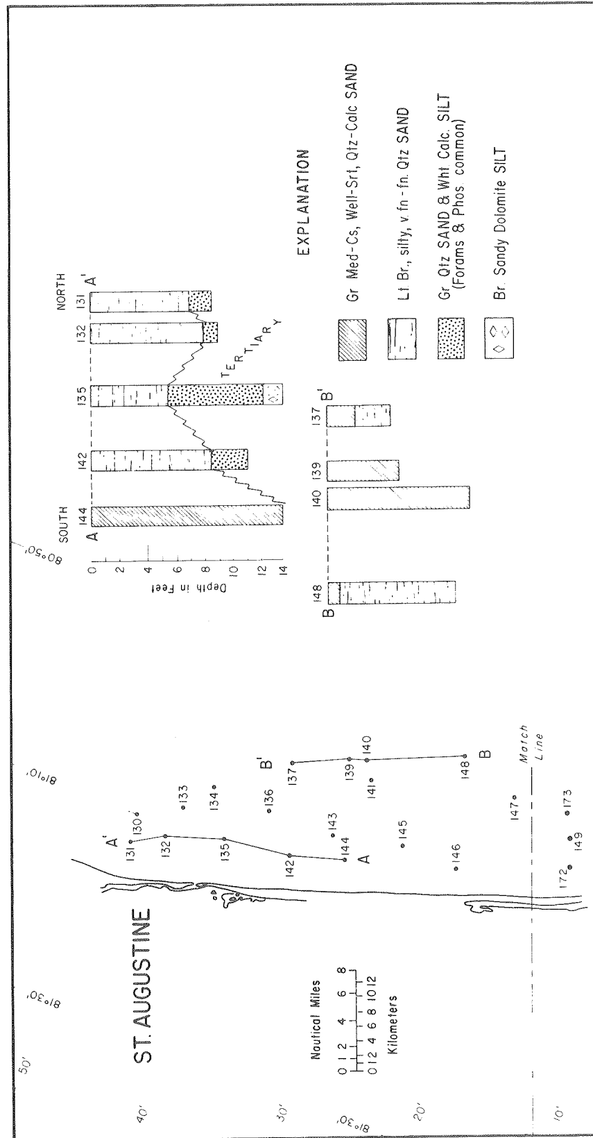
Figure 35. Lithostratigraphic correlations along selected transects between St. Augustine and Daytona Beach.
