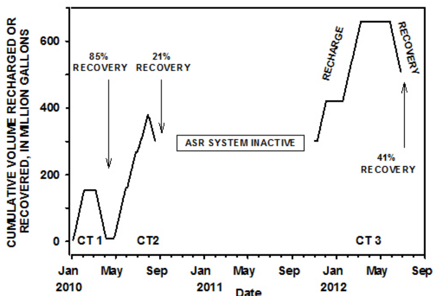
Figure 9-2 -- Cycle test (CT) history at the Hillsboro ASR system.
