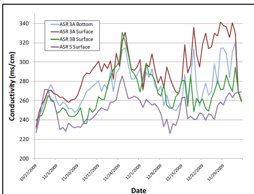
Figure 10-9 -- Specific conductance (ms/cm) at sampling stations in the Kissimmee River
