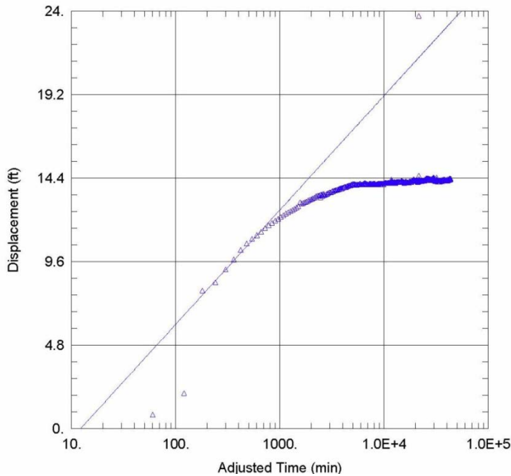
Figure 5-32 -- Drawdown versus Time for the 1,010-ft SZMW (CTD data) during the recovery (extraction) phase of cycle test 1 at HASR.
