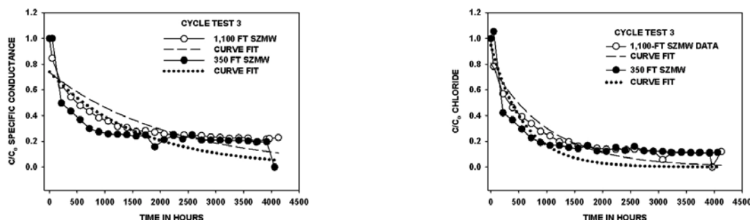
Figure 5-3 -- Plots showing breakthrough curves and curve fits using normalized specific conductance and chloride data at the 1,100-ft SZMW.
