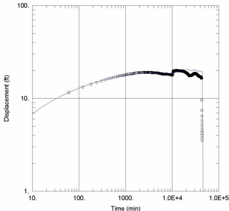
Figure 5-19 -- Displacement versus Time for the 330-ft SZMW (CTD data) during the recharge (injection) phase of cycle test 1 at HASR.
