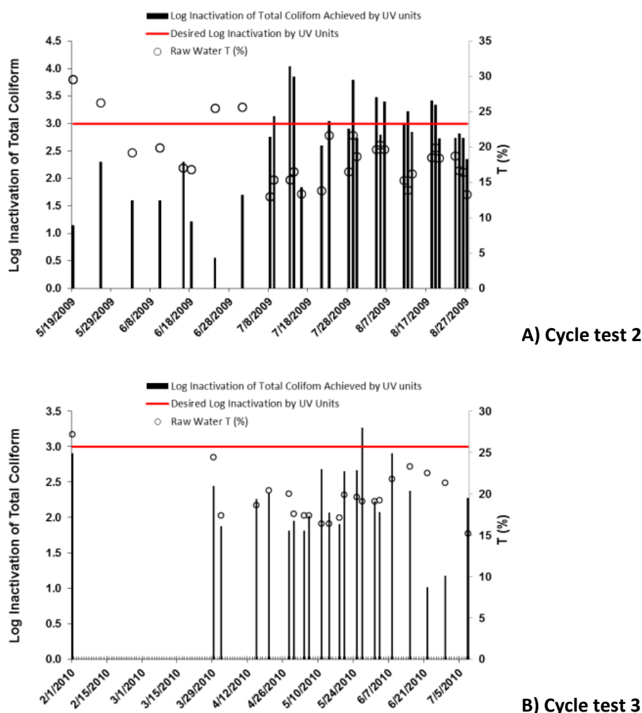
Figure 12-2 (A and B) -- Time-series plots showing UV disinfection system performance (as log inactivation) and percent transmittance.
