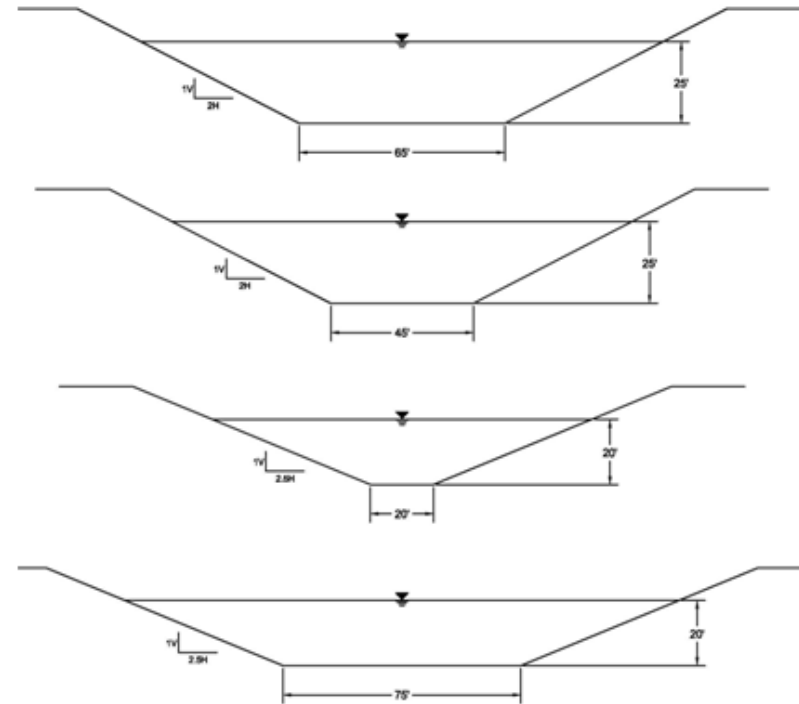
Figure 2. Cross-sections of representative canals within (a) Miami-Dade (C-100), Broward (C-12) and Palm Beach (C-18) counties and Kissimmee River Channel (C-38) and (b) selected locations within the West Palm Beach Canal (C-51).
