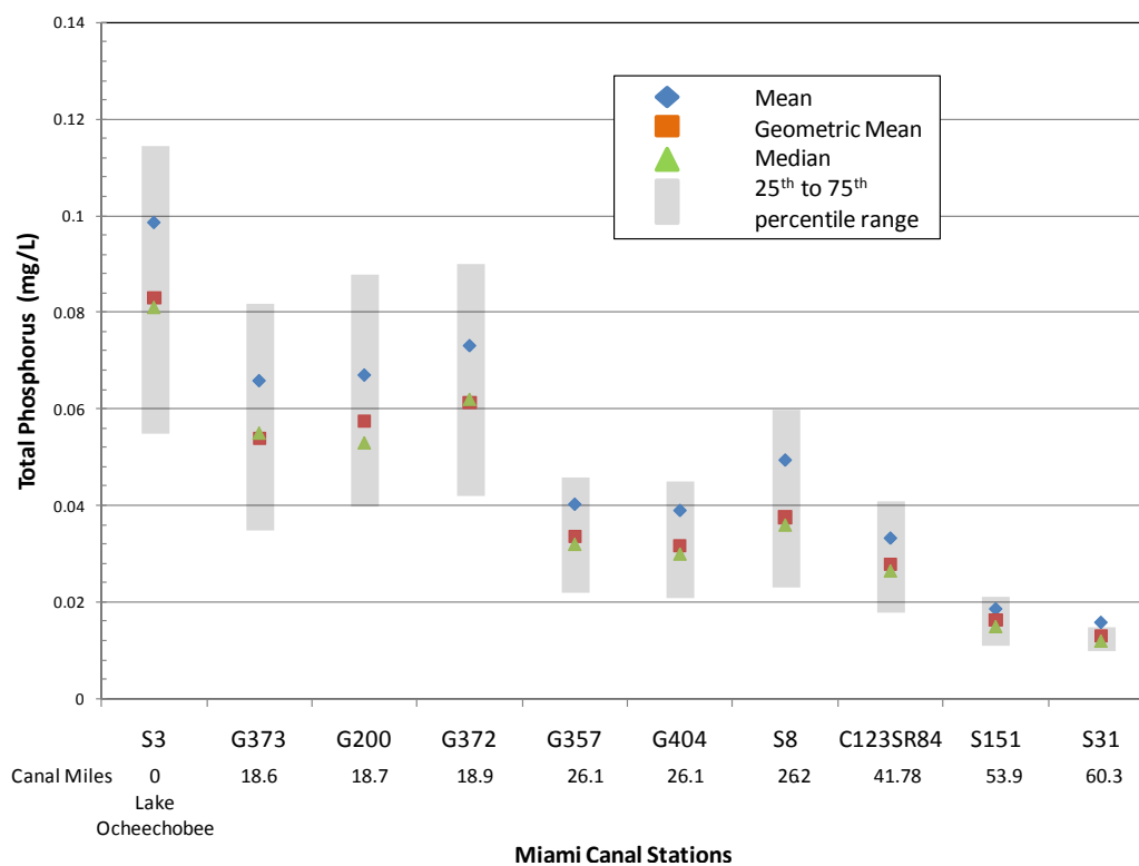
Figure 30. Total phosphorus concentration summary statistics for stations in the Miami Canal.
