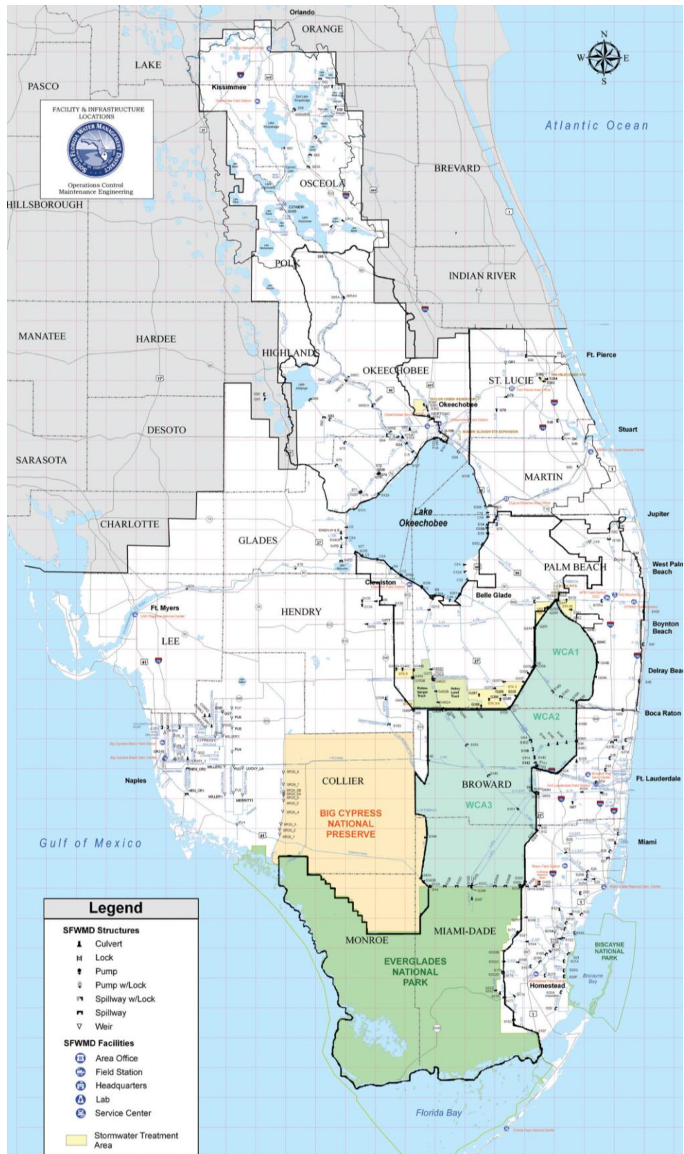
Figure 1. Primary SFWMD canals, structures, and major features of the hydrologic system.
