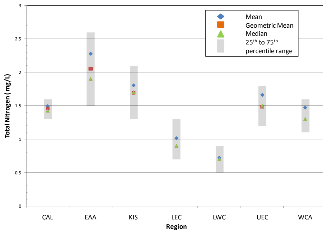
Figure 13. Total nitrogen concentration summary statistics by region.
