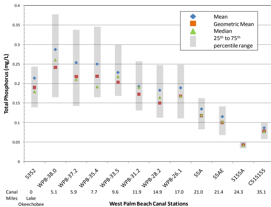
Figure 27. Total phosphorus concentration summary statistics for stations in the West Palm Beach Canal.
