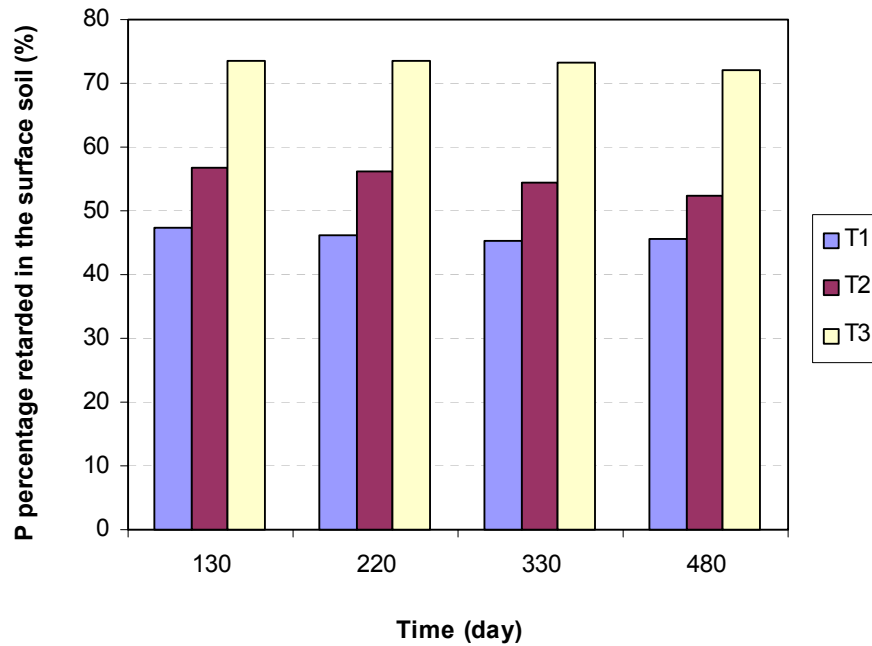
Figure 40. P Retained in the Surface Soil from P-Treated Plots \text{H}_3\text{PO}_4 (T1), \text{H}_3\text{PO}_4 + \text{Ca}(\text{H}_2\text{PO}_4)_2 (T2), and \text{H}_3\text{PO}_4 + Phosphate Rock (T3).
