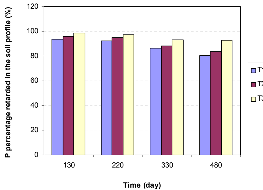
Figure 41. P Retained in the Soil Profile from P-Treated Plots \text{H}_3\text{PO}_4 (T1), \text{H}_3\text{PO}_4 + \text{Ca}(\text{H}_2\text{PO}_4)_2 (T2), and \text{H}_3\text{PO}_4 + Phosphate Rock (T3).
