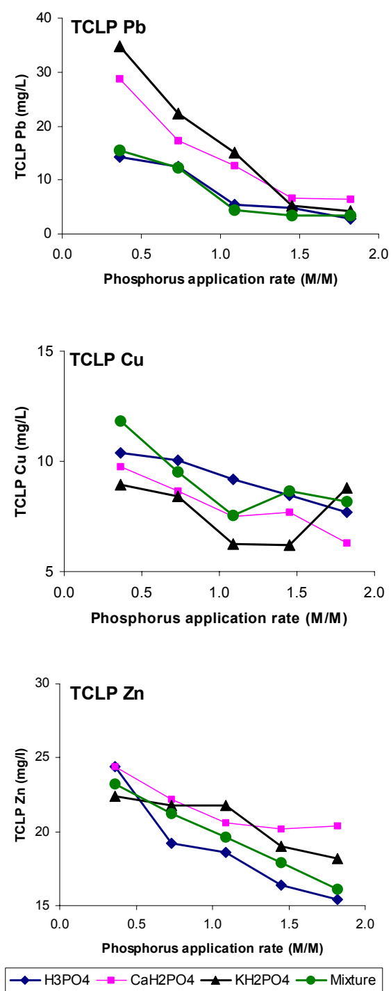
Figure 10. TCLP- Extractable Metals ( \text{mg L}^{-1} ) in Phosphate-Amended Soil.
