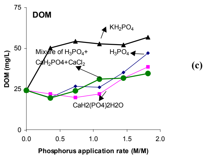
Figure 8. Chemical Characteristics of Batch Leachates: (a) pH, (b) Soluble Phosphorus Concentration ( \text{mg L}^{-1} ), and (c) Dissolved Organic Matter ( \text{mg L}^{-1} ).
