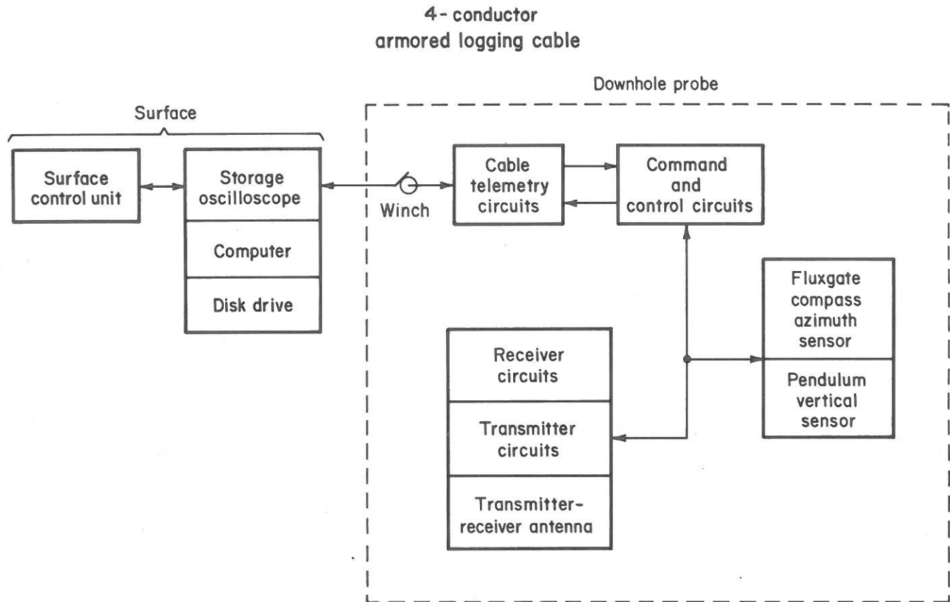
FIGURE 4. - Block diagram detailing major elements of GPR subsurface probe system.
