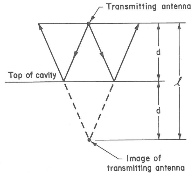
FIGURE 3. - Propagation path of radar waves.
