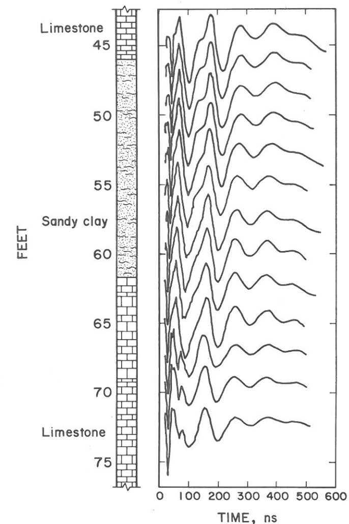
FIGURE 11. - Correlation of signatures obtained in hole H. (Note reflections at approximately 80 ns at the 63- to 71-ft depth.)
