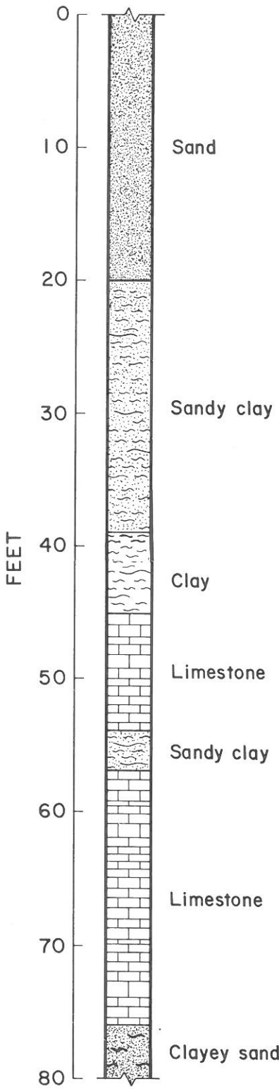
FIGURE 18. - Log of solid-ground hole approximately 1,000 ft north of cavity.
