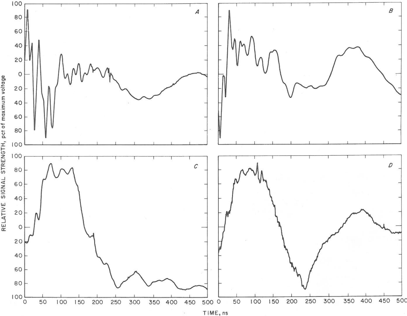
FIGURE 17. - Radar scans: A, taken over cavity hole A; B, taken 1,000 ft from cavity, over solid earth; C, taken over a proposed damsite area; D, taken on existing dam.
