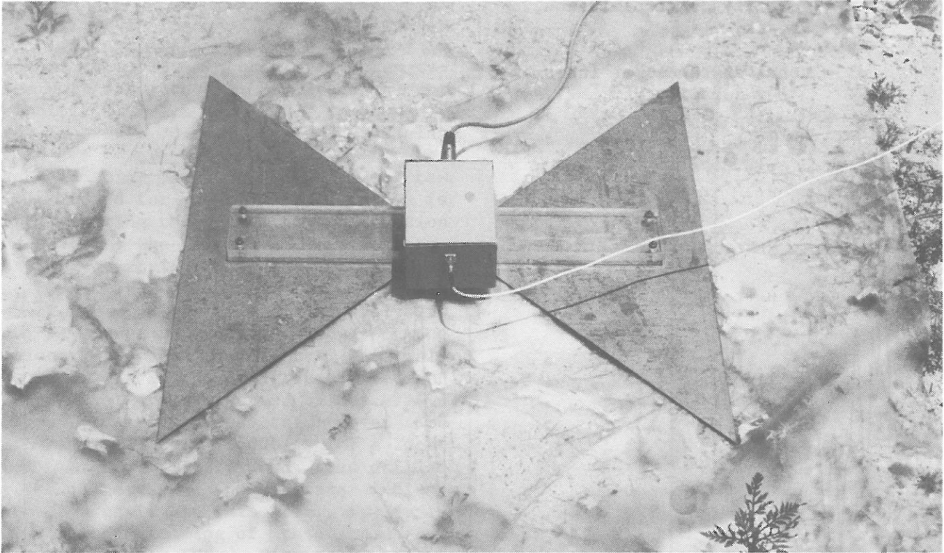
FIGURE 15. - Transmitter attached to surface dipole antenna.
