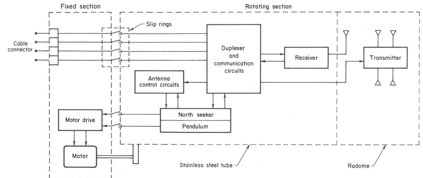
FIGURE 7. - Block diagram detailing circuitry in each major division of borehole probe.
