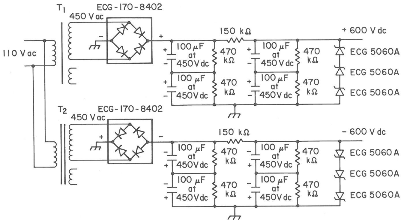
FIGURE 14. - Schematic of 4,000-W, 1,200-V power supply.
