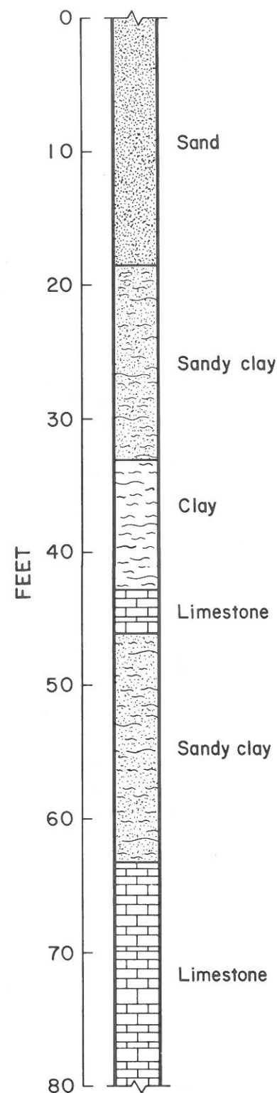
FIGURE 2. - Log of hole H depicting differing strata. The top of the cavity lies at approximately 58 ft.
