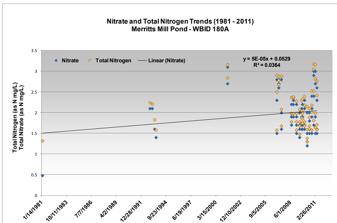
Figure 2.13. Nitrogen Trends for Merritts Mill Pond, 1981–2011
