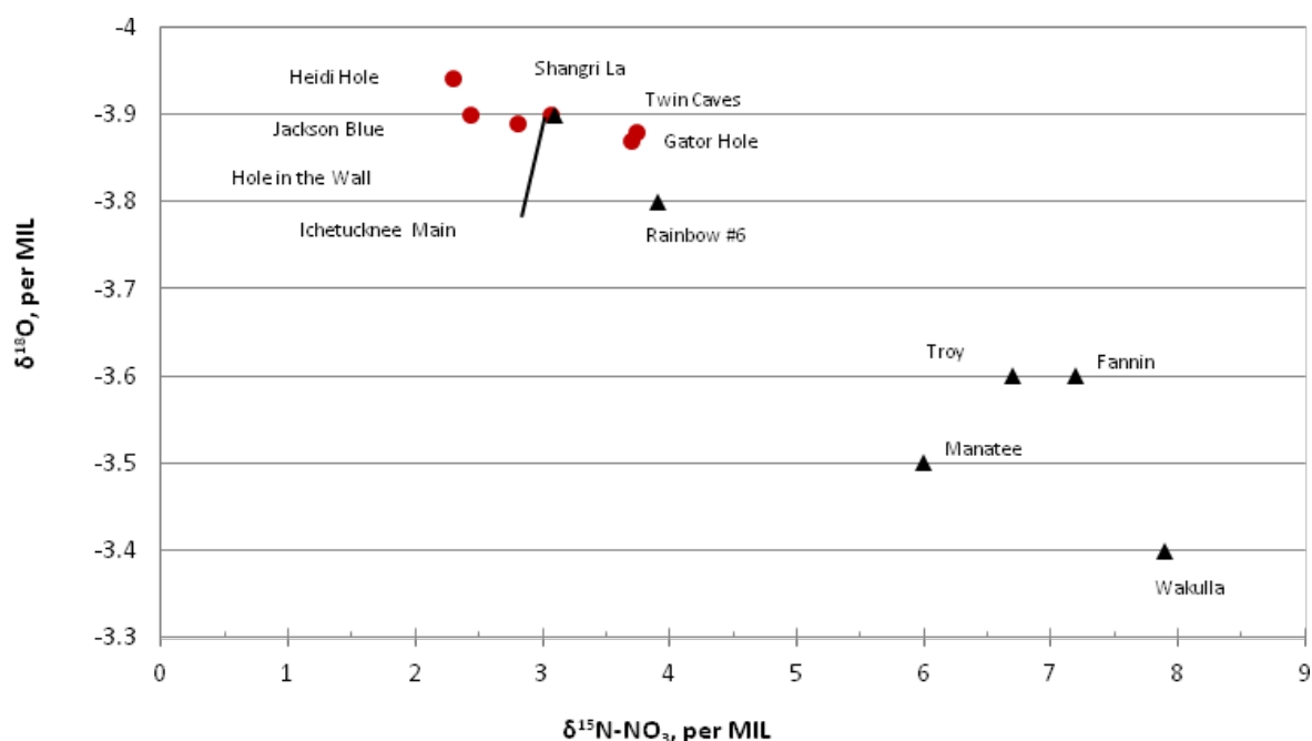
Figure 4.2. Delta ^{15}\text{N} vs. Delta ^{18}\text{O} (Barrios 2011)
