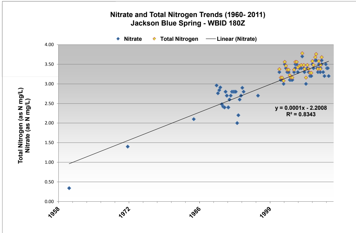
Figure 2.12. Nitrate and Total Nitrogen Trends for Jackson Blue Spring, 1960–2011
