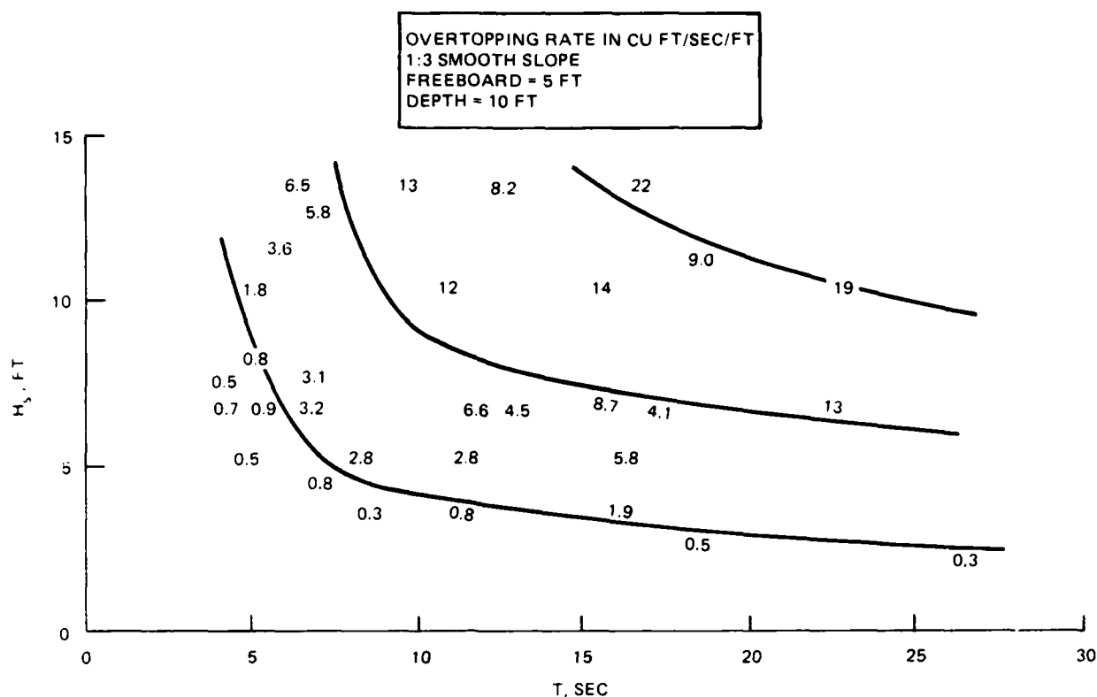
Figure 5. Dimensional overtopping rate plot, Example 2
