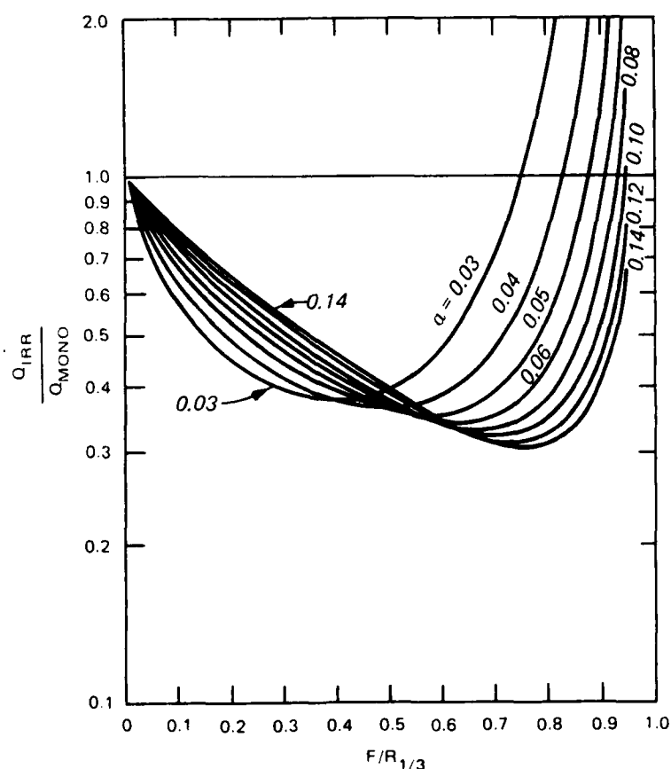
Figure 3. Ahrens' correction factors (from Ahrens 1977a)
