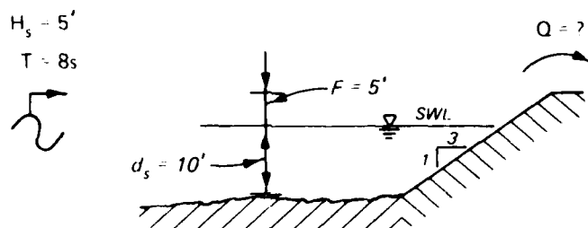
Figure 4. Definition sketch, Example 1
