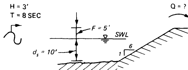
Figure 11. Definition sketch, Example 4
