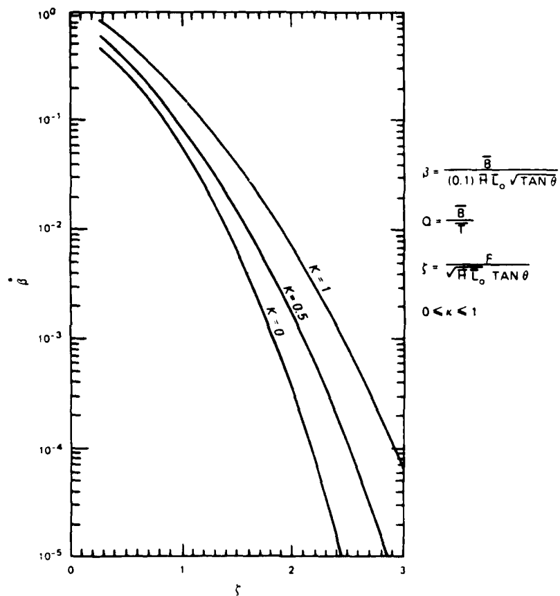
Figure 9. Battjes' irregular wave overtopping (from Battjes 1974)
