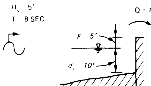
Figure 7. Definition sketch, Example 3
