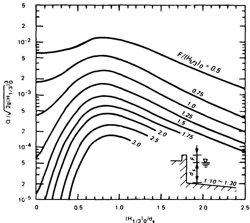
Figure 6. Goda's irregular-wave overtopping rate (from Goda 1971)
