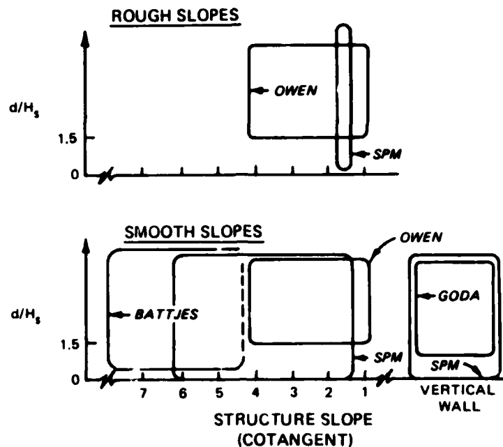
Figure 14. General regions of applicability of overtopping methods
