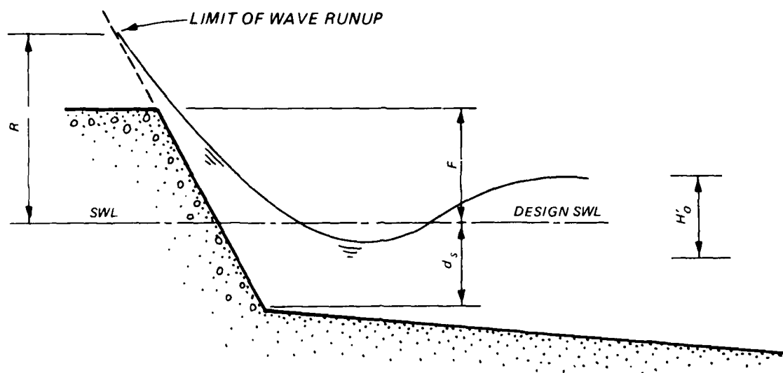
Figure 1. Wave runup definition sketch
